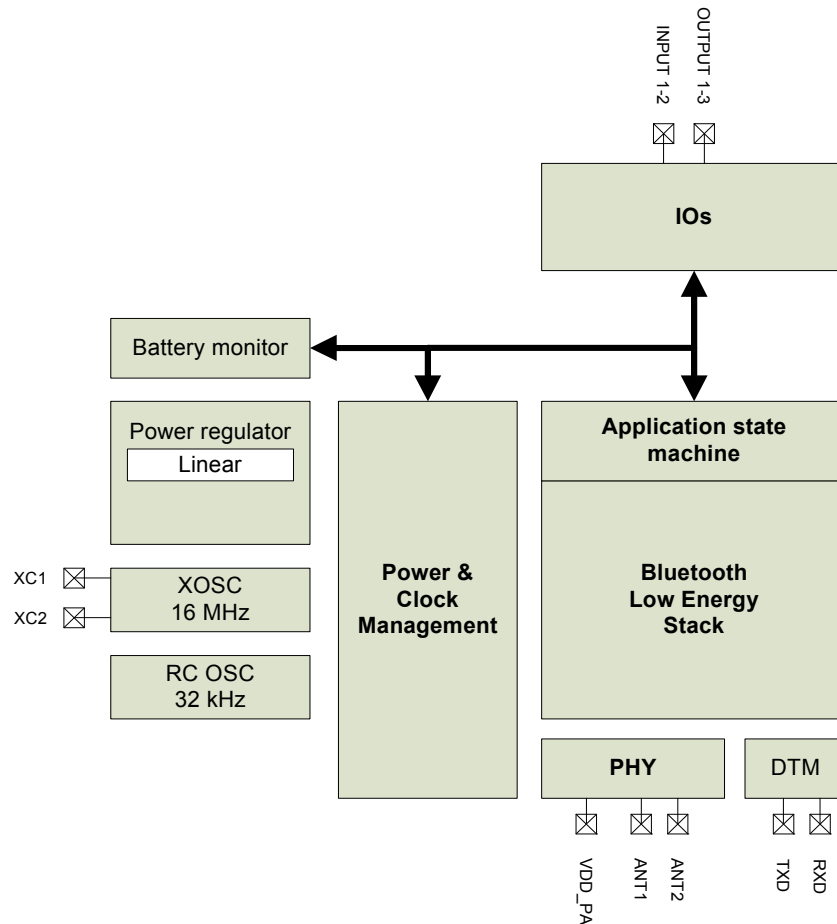
Figure 1. nRF8002 block diagram
