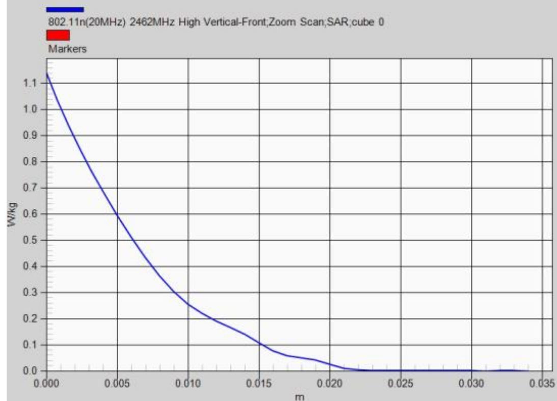
Interpolated Max SAR Z Line(z)
