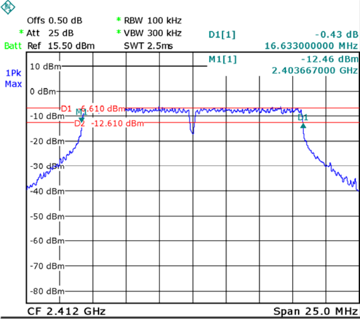
ANT0 TX 11g Low channel
