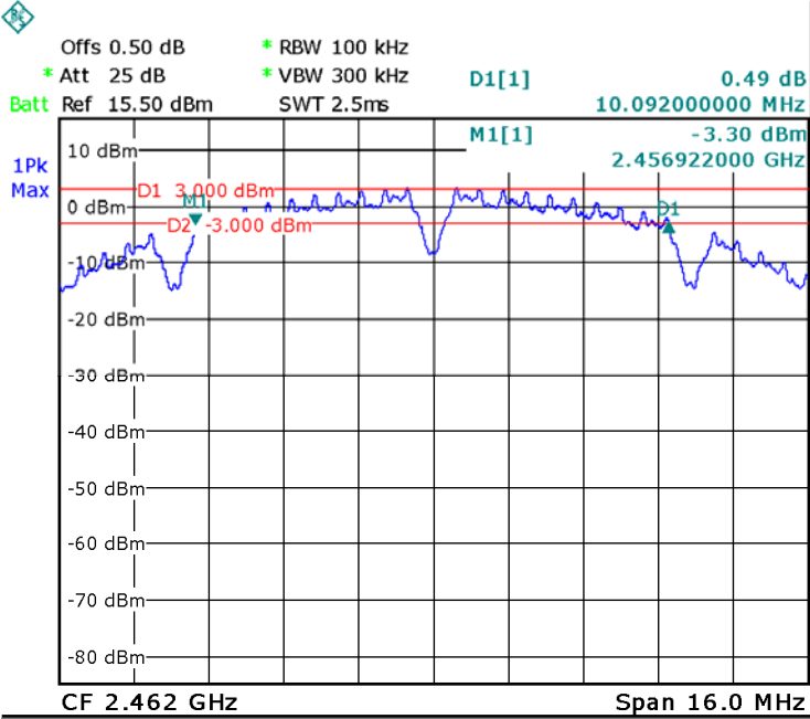
ANT0 TX 11b High channel
