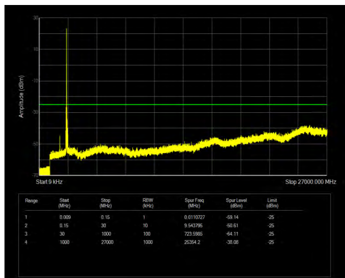
Band38 QPSK BW=15MHz Channel=38000 RB Size=1 Position=#0
