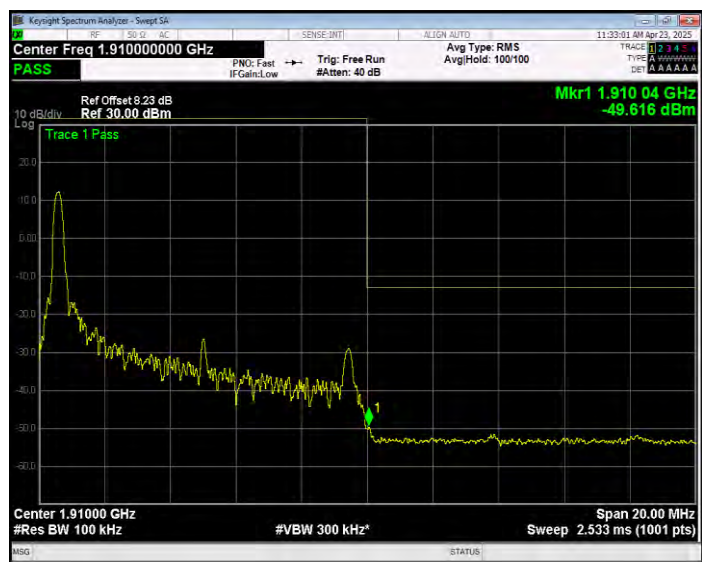
Band2 16QAM BW=10MHz Channel=19150 RB Size=1 Position=#Max Extended
