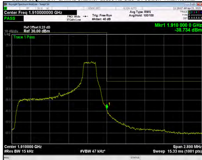
Band2 16QAM BW=1.4MHz Channel=19193 RB Size=6 Position=#0 Extended
