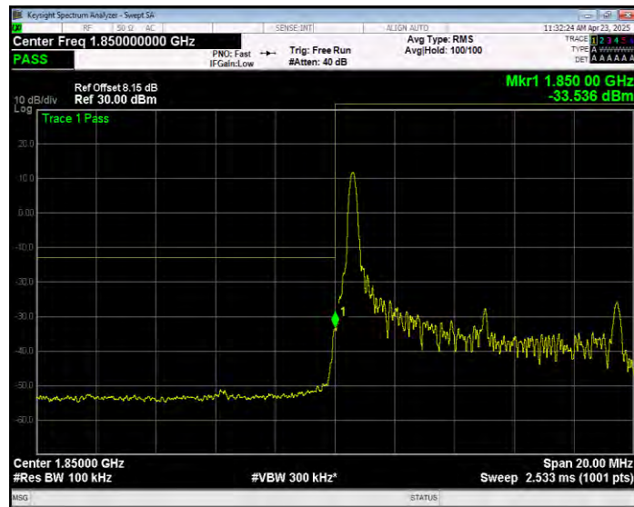
Band2 16QAM BW=10MHz Channel=18650 RB Size=1 Position=#Max Extended
