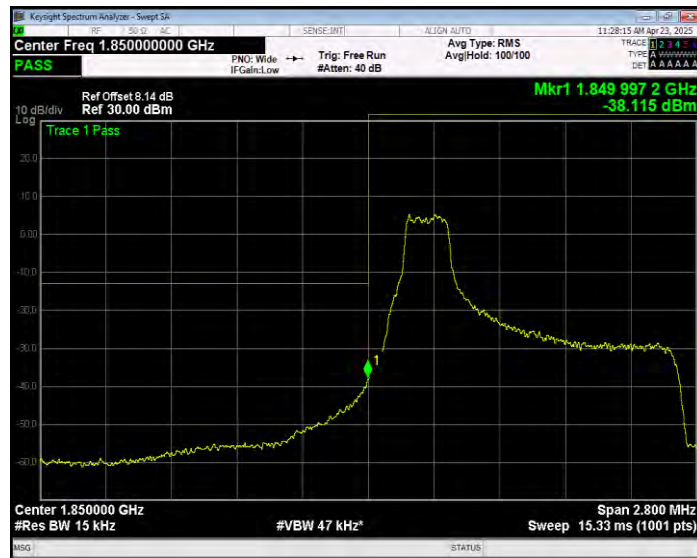
Band2 16QAM BW=1.4MHz Channel=18607 RB Size=1 Position=#Max Extended
