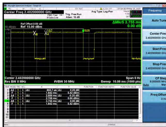
Bluetooth For Classic 2-DH5 2402MHz
