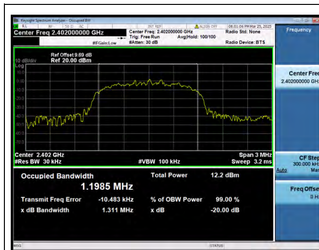
Bluetooth For Classic 3-DH5 2402MHz
