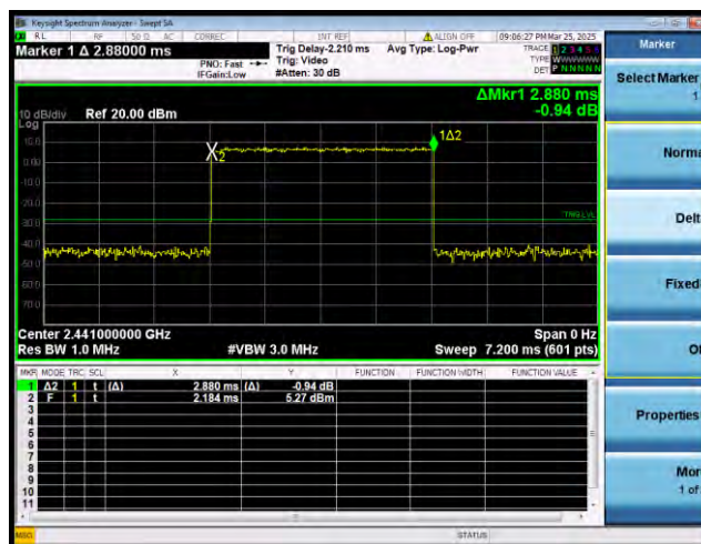
Bluetooth For Classic 3-DH5 2441MHz
