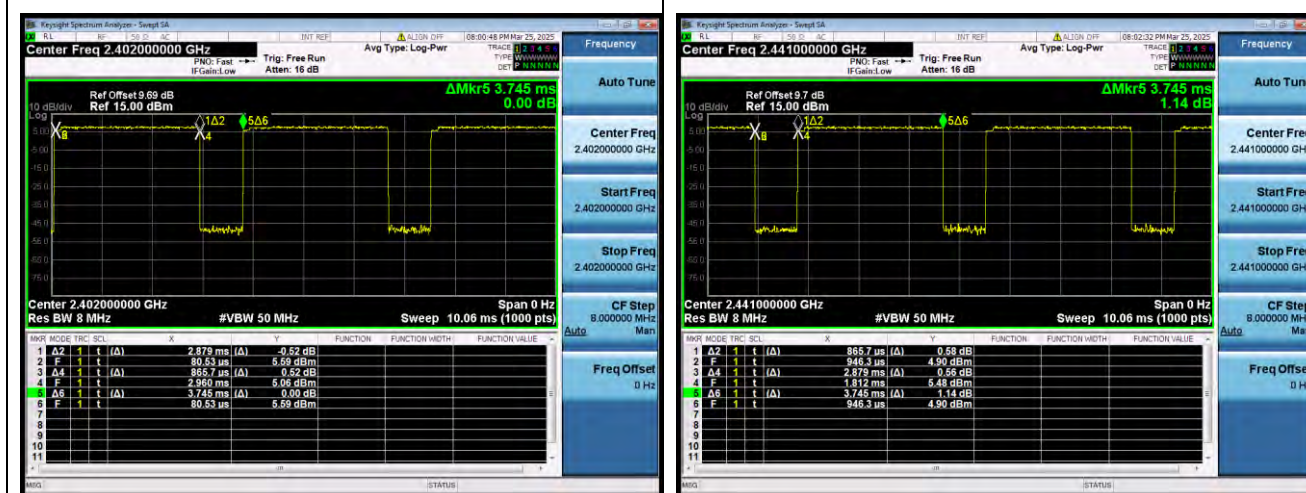
Bluetooth For Classic 3-DH5 2402MHz
