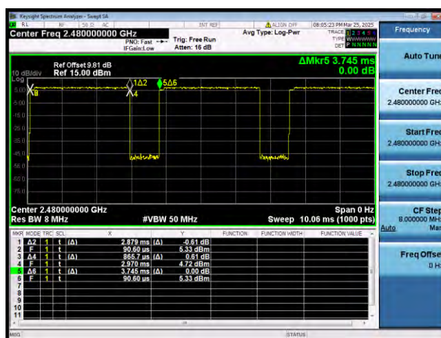
Bluetooth For Classic 3-DH5 2480MHz
