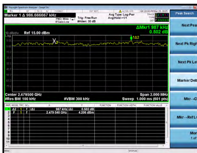
Bluetooth For Classic 3-DH5 2480MHz
