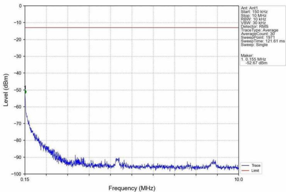
Band25_10MHz_16QAM_HCH_1910MHz_RB_1_0_NTNV
