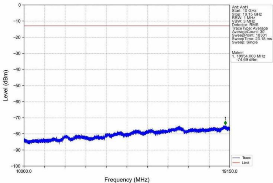
Band25_15MHz_QPSK_HCH_1907.5MHz_RB_1_74_NTNV
