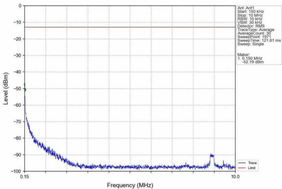
Band25_20MHz_16QAM_LCH_1860MHz_RB_1_0_NTNV
