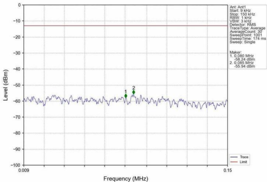
Band25_20MHz_16QAM_LCH_1860MHz_RB_1_0_NTNV
