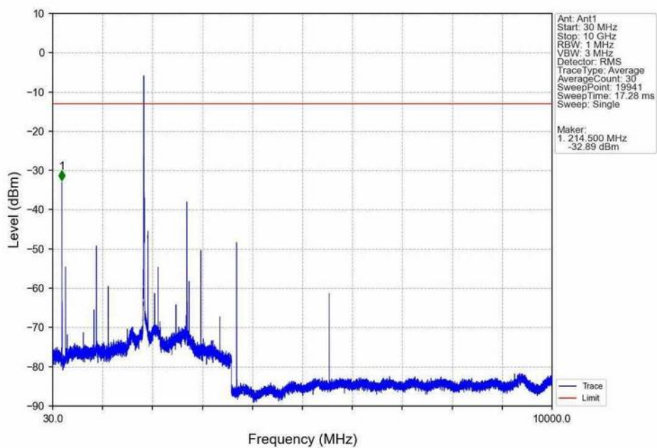
Band25_5MHz_16QAM_LCH_1852.5MHz_RB_1_0_NTNV
