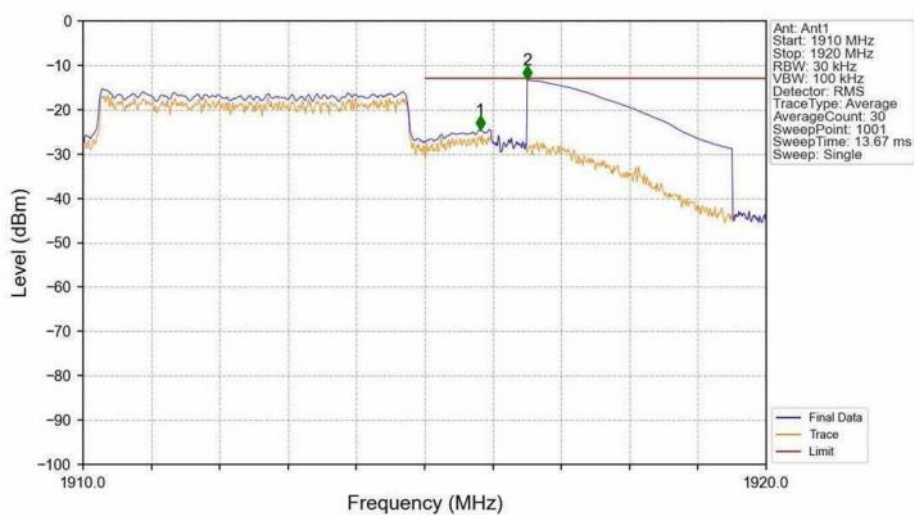
Band25_5MHz_16QAM_HCH_1912.5MHz_RB_25_0_NTNV
