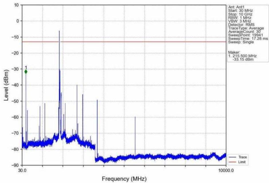
Band25_20MHz_16QAM_LCH_1860MHz_RB_1_0_NTNV
