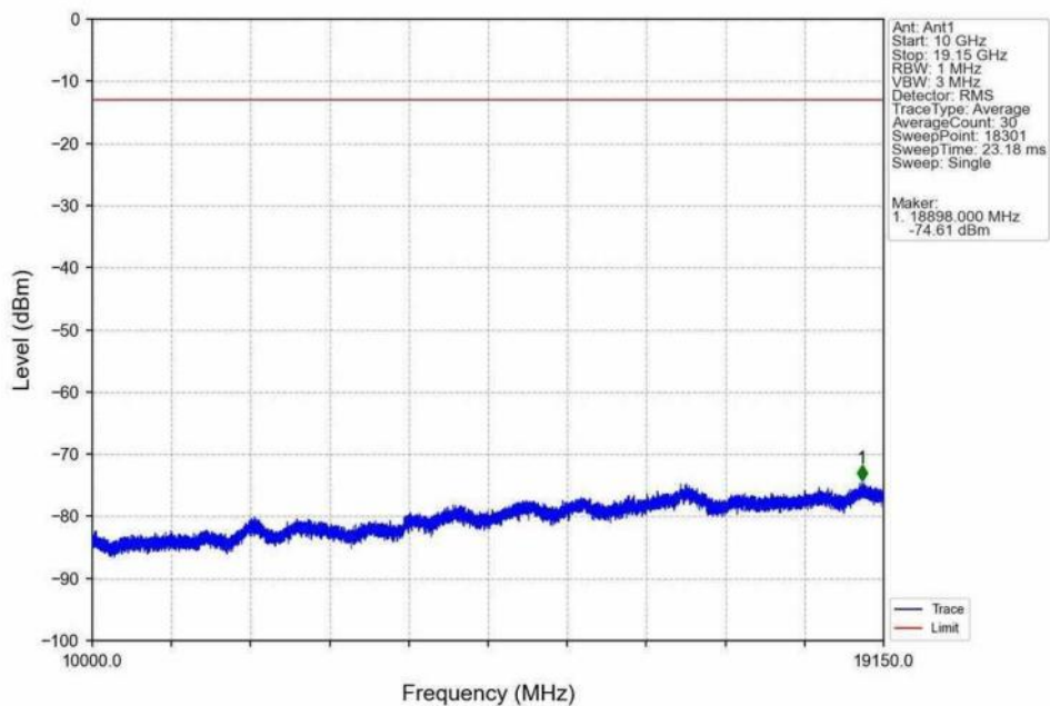
Band25_20MHz_16QAM_HCH_1905MHz_RB_1_99_NTNV
