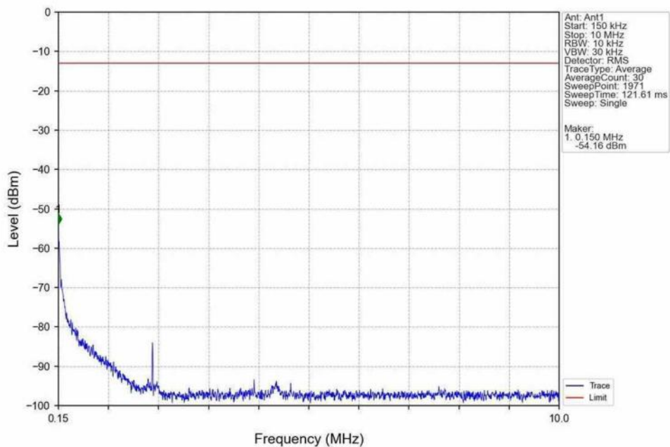
Band25_10MHz_QPSK_MCH_1882.5MHz_RB_1_0_NTNV
