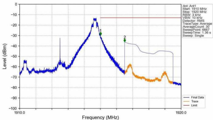
Band25_5MHz_16QAM_HCH_1912.5MHz_RB_1_24_NTNV
