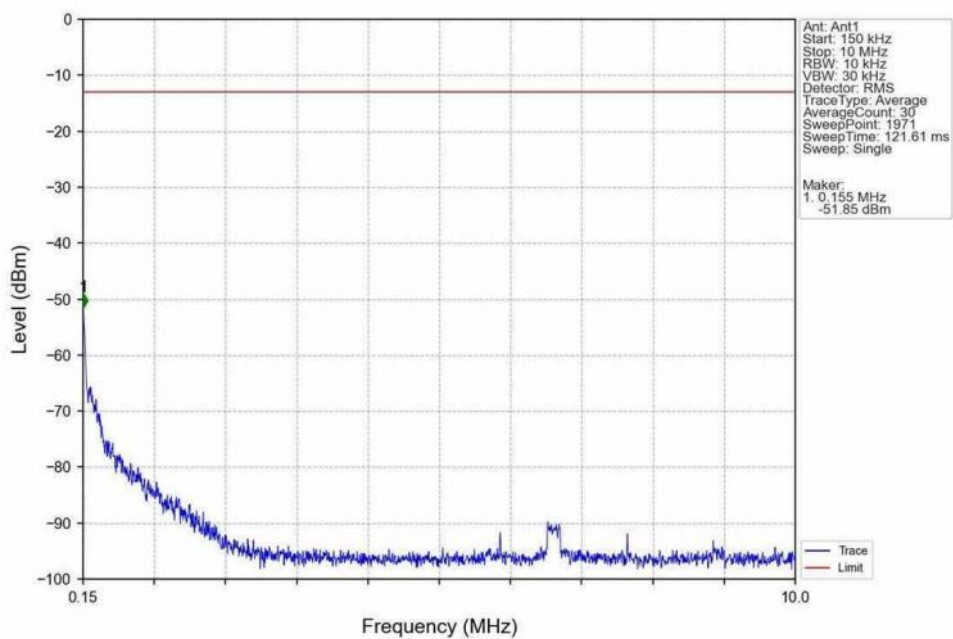
Band25_15MHz_16QAM_HCH_1907.5MHz_RB_1_0_NTNV
