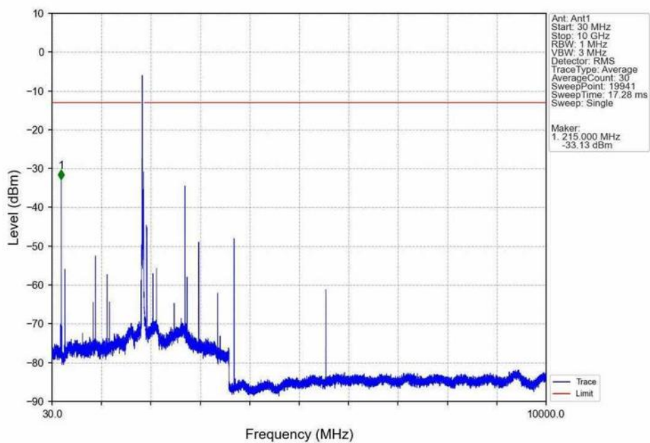
Band25_15MHz_16QAM_LCH_1857.5MHz_RB_1_0_NTNV
