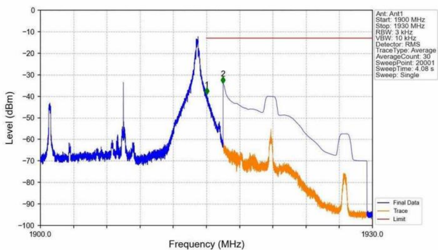
Band25_15MHz_QPSK_HCH_1907.5MHz_RB_1_74_NTNV
