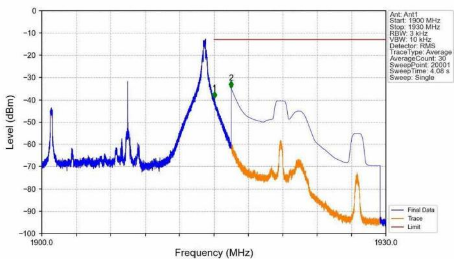
Band25_15MHz_16QAM_HCH_1907.5MHz_RB_1_74_NTNV
