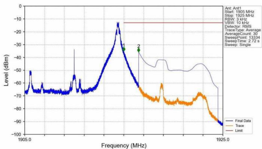
Band25_10MHz_16QAM_HCH_1910MHz_RB_1_49_NTNV
