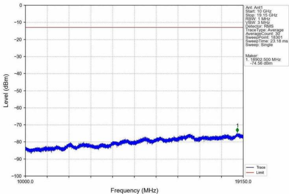
Band25_15MHz_16QAM_HCH_1907.5MHz_RB_1_74_NTNV
