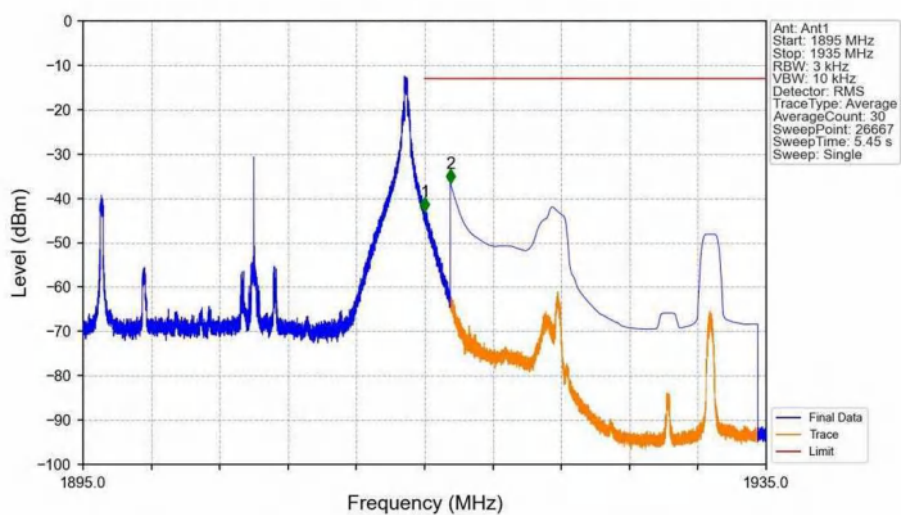
Band25_20MHz_16QAM_HCH_1905MHz_RB_1_99_NTNV
