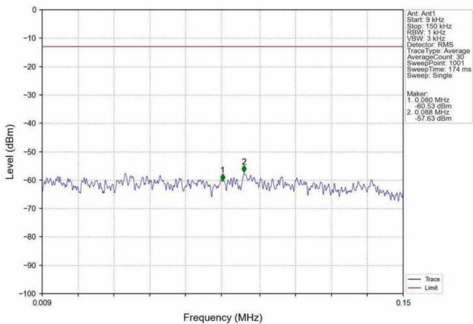
Band25_20MHz_16QAM_MCH_1882.5MHz_RB_1_0_NTNV
