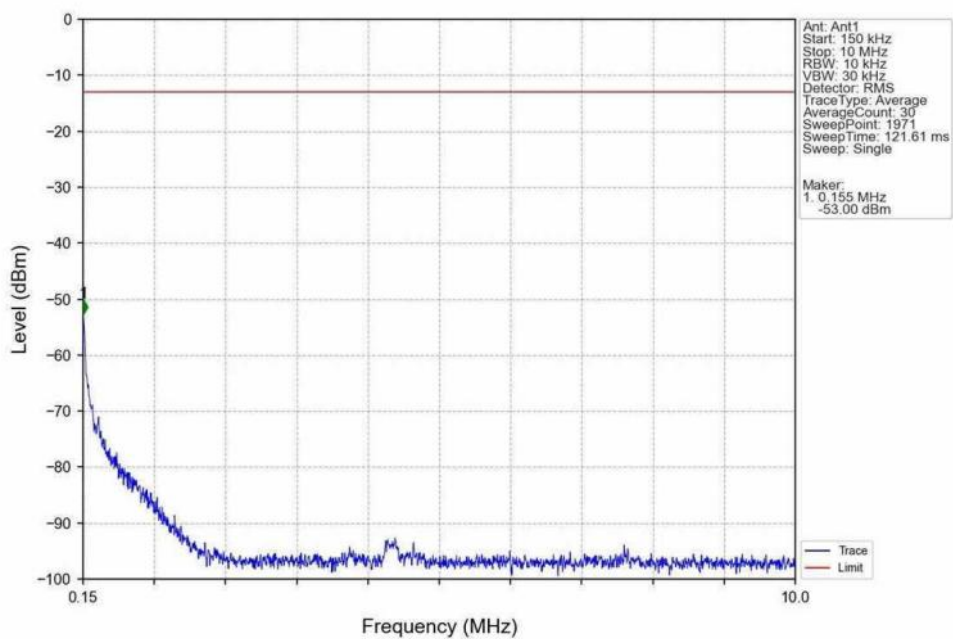
Band25_10MHz_16QAM_LCH_1855MHz_RB_1_0_NTNV
