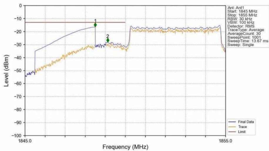
Band25_5MHz_16QAM_LCH_1852.5MHz_RB_25_0_NTNV
