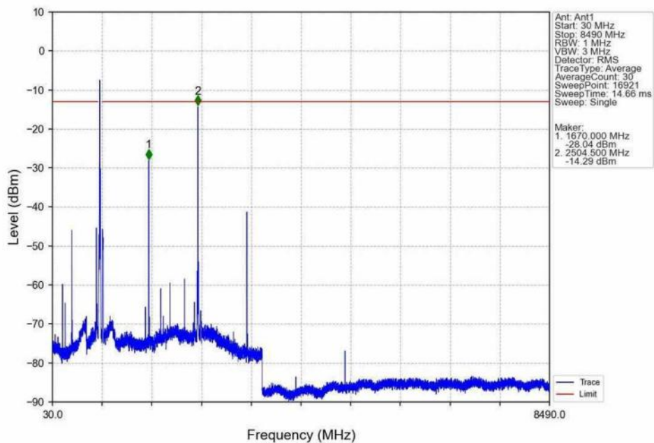
Band26b_15MHz_16QAM_HCH_841.5MHz_RB_1_74_NTNV
