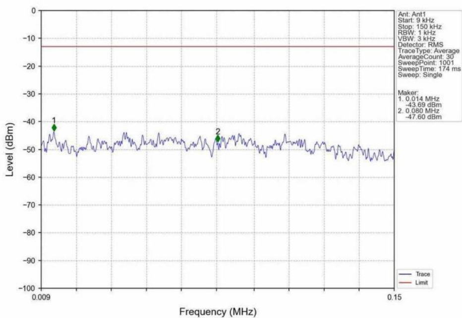
Band26b_15MHz_16QAM_LCH_831.5MHz_RB_1_0_NTNV
