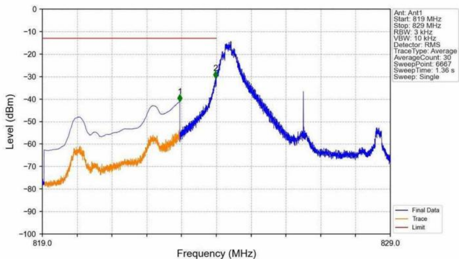
Band26b_5MHz_16QAM_LCH_826.5MHz_RB_1_0_NTNV
