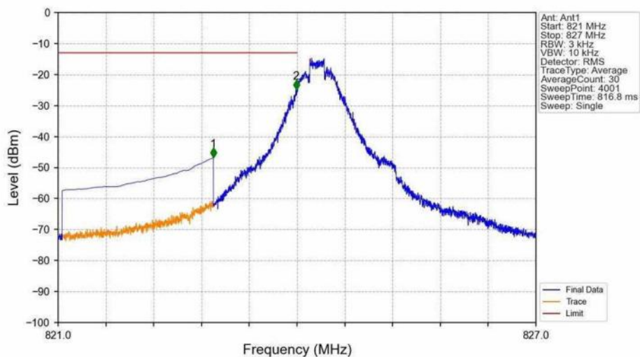
Band26b_1.4MHz_16QAM_LCH_824.7MHz_RB_1_0_NTNV
