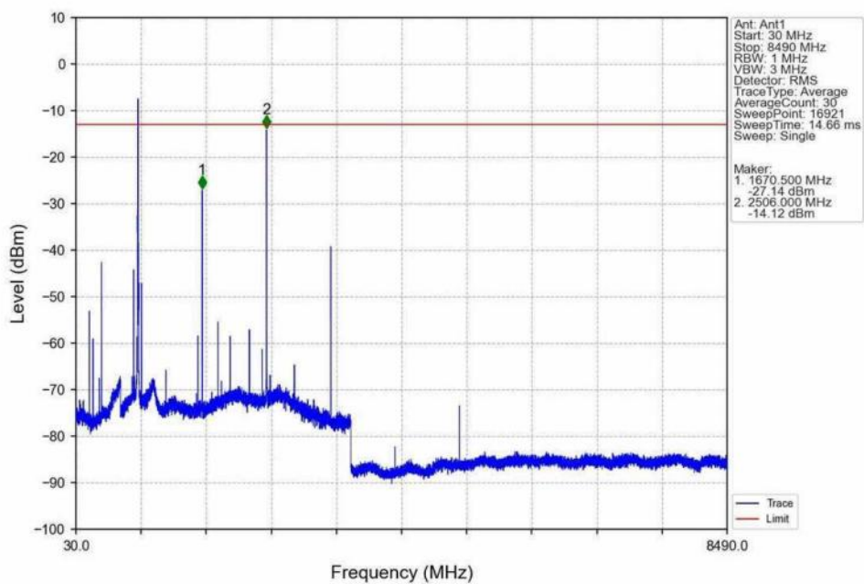
Band26b_3MHz_QPSK_MCH_836.5MHz_RB_1_0_NTNV
