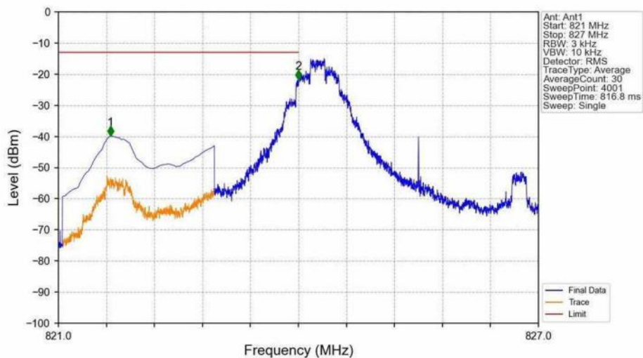
Band26b_3MHz_QPSK_LCH_825.5MHz_RB_1_0_NTNV
