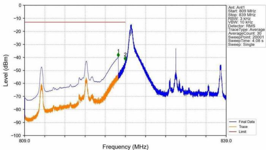
Band26b_15MHz_16QAM_LCH_831.5MHz_RB_1_0_NTNV
