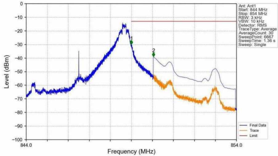
Band26b_5MHz_16QAM_HCH_846.5MHz_RB_1_24_NTNV
