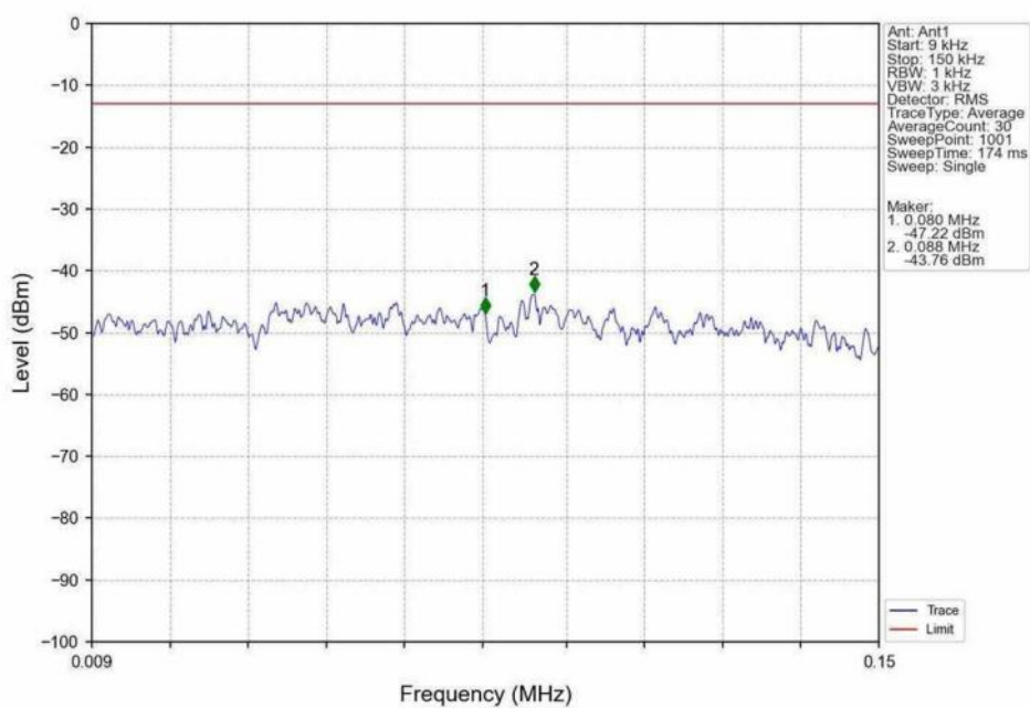
Band26b_1.4MHz_16QAM_LCH_824.7MHz_RB_1_0_NTNV
