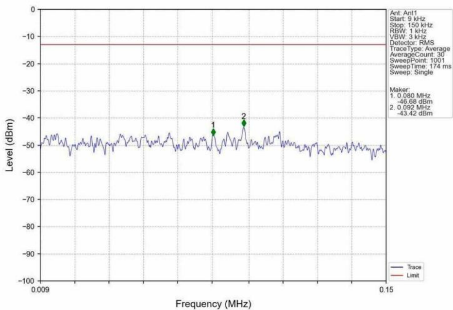
Band26b_15MHz_16QAM_HCH_841.5MHz_RB_1_0_NTNV
