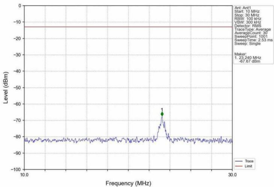
Band26b_3MHz_QPSK_LCH_825.5MHz_RB_1_0_NTNV
