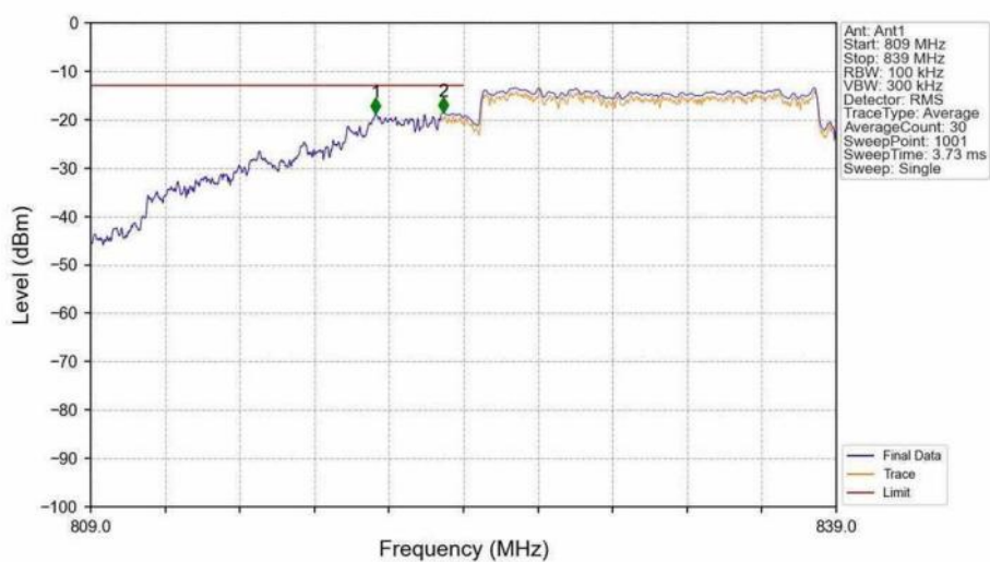
Band26b_15MHz_QPSK_LCH_831.5MHz_RB_75_0_NTNV
