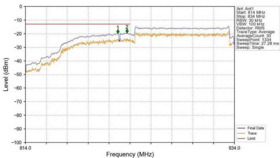
Band26b_10MHz_QPSK_LCH_829MHz_RB_50_0_NTNV
