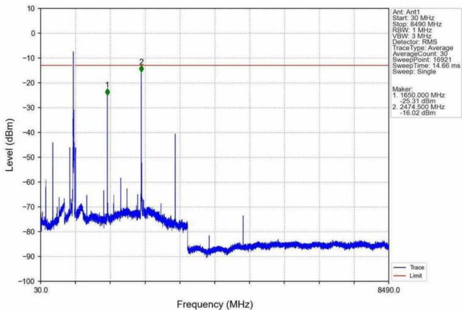
Band26b_15MHz_16QAM_MCH_836.5MHz_RB_1_0_NTNV
