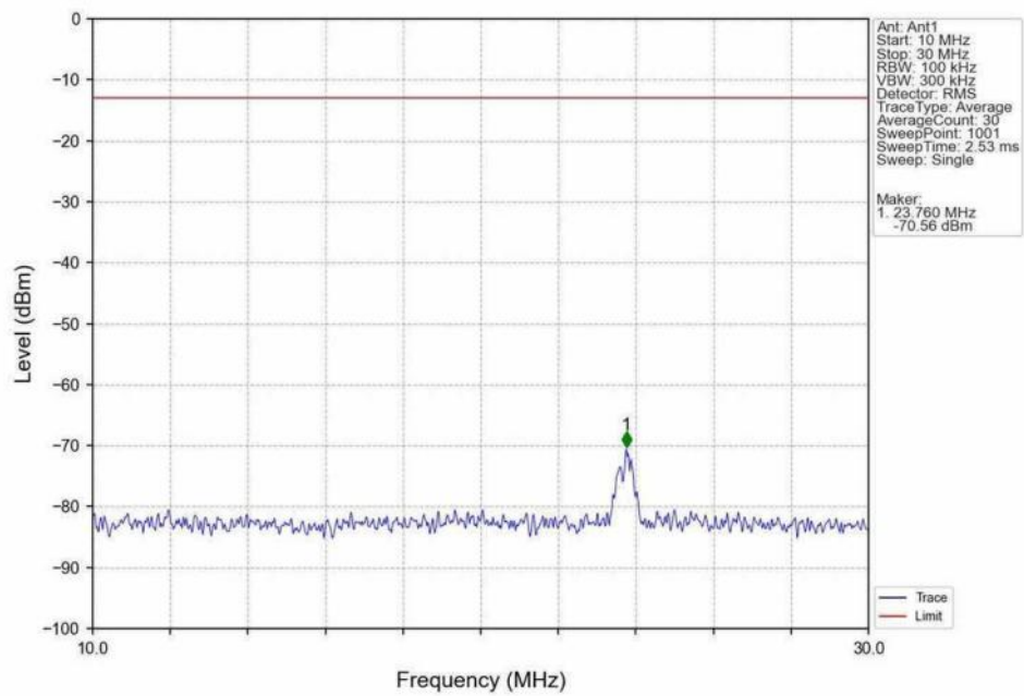
Band26b_5MHz_16QAM_LCH_826.5MHz_RB_1_0_NTNV
