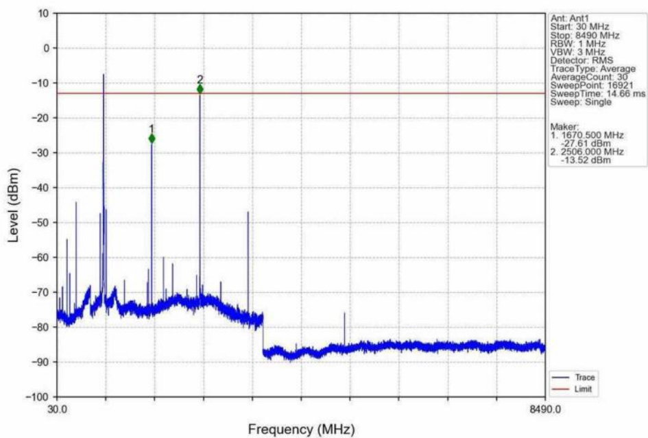
Band26b_3MHz_16QAM_MCH_836.5MHz_RB_1_0_NTNV
