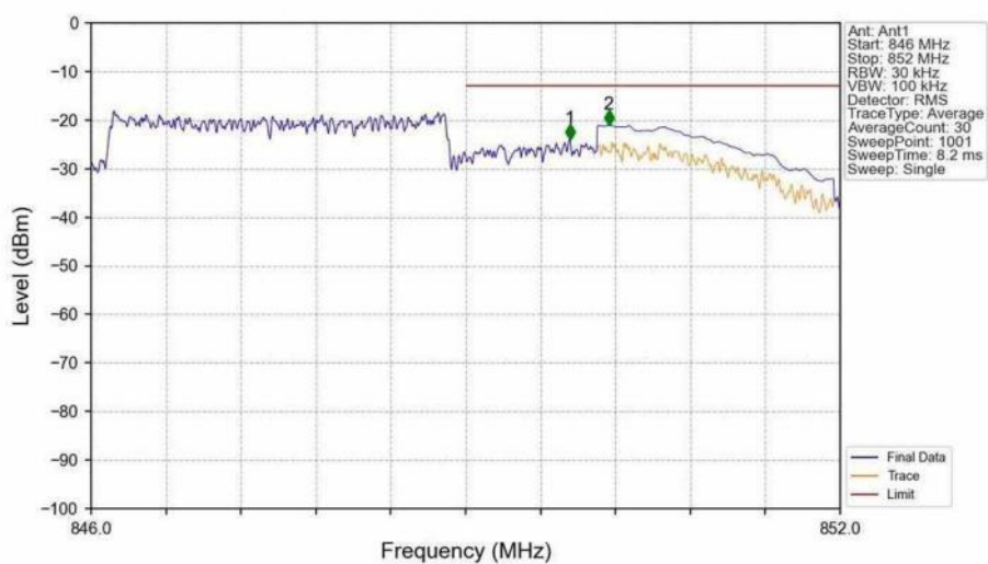
Band26b_3MHz_16QAM_HCH_847.5MHz_RB_15_0_NTNV
