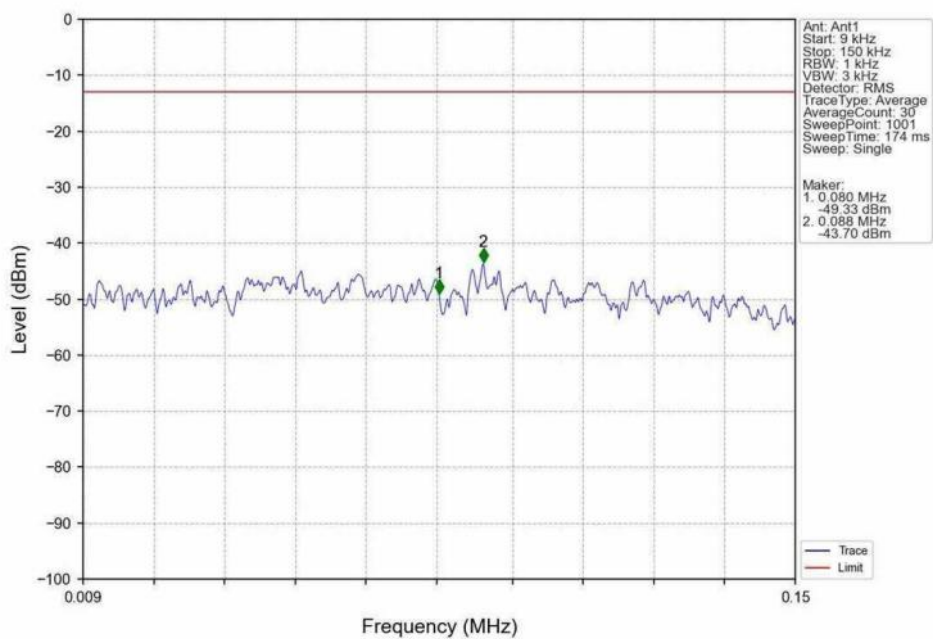
Band26b_15MHz_16QAM_MCH_836.5MHz_RB_1_0_NTNV
