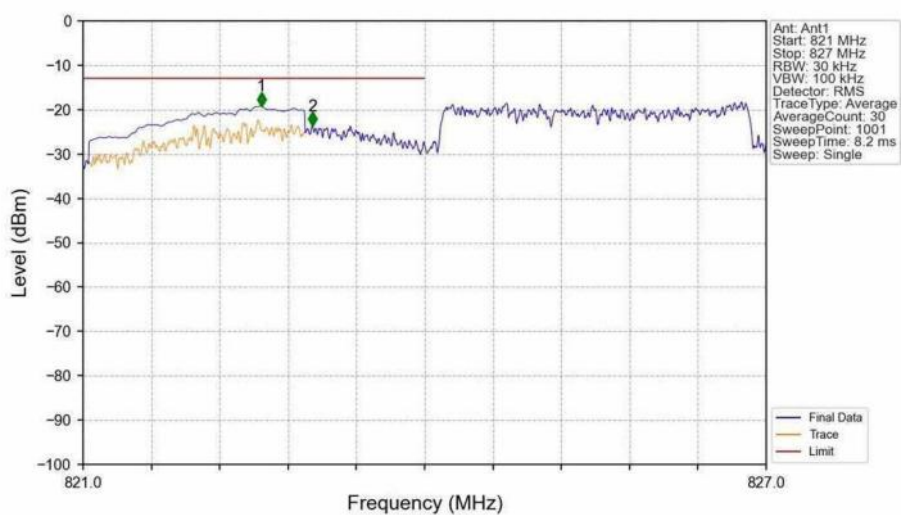
Band26b_3MHz_16QAM_LCH_825.5MHz_RB_15_0_NTNV
