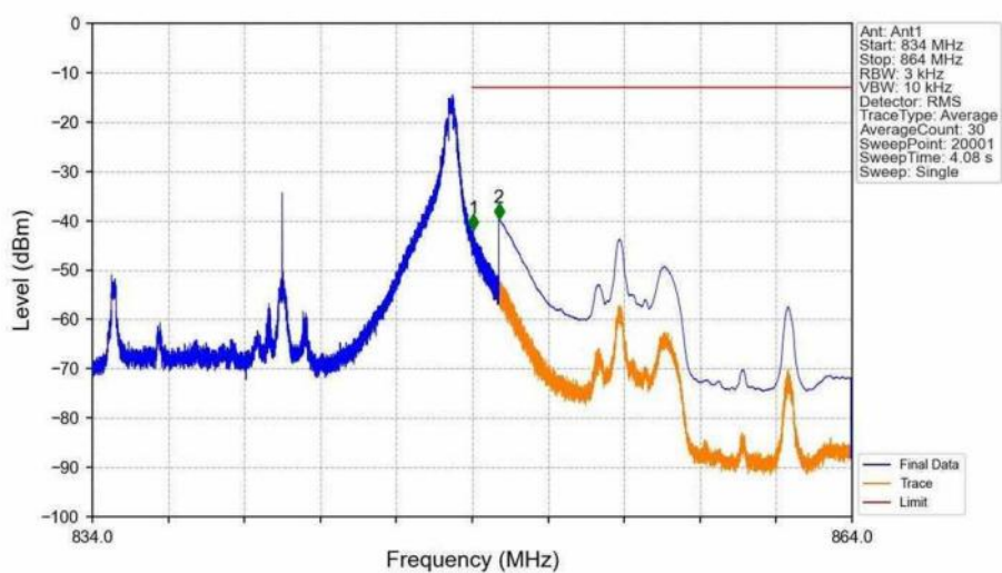
Band26b_15MHz_16QAM_HCH_841.5MHz_RB_1_74_NTNV
