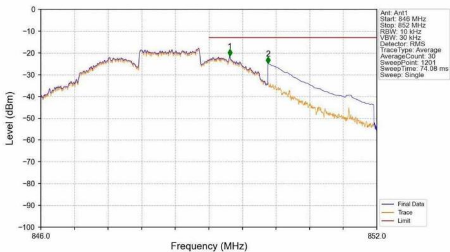
Band26b_1.4MHz_16QAM_HCH_848.3MHz_RB_6_0_NTNV
