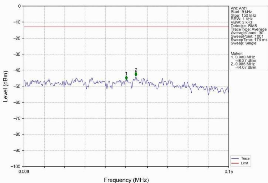
Band26b_10MHz_16QAM_LCH_829MHz_RB_1_0_NTNV
