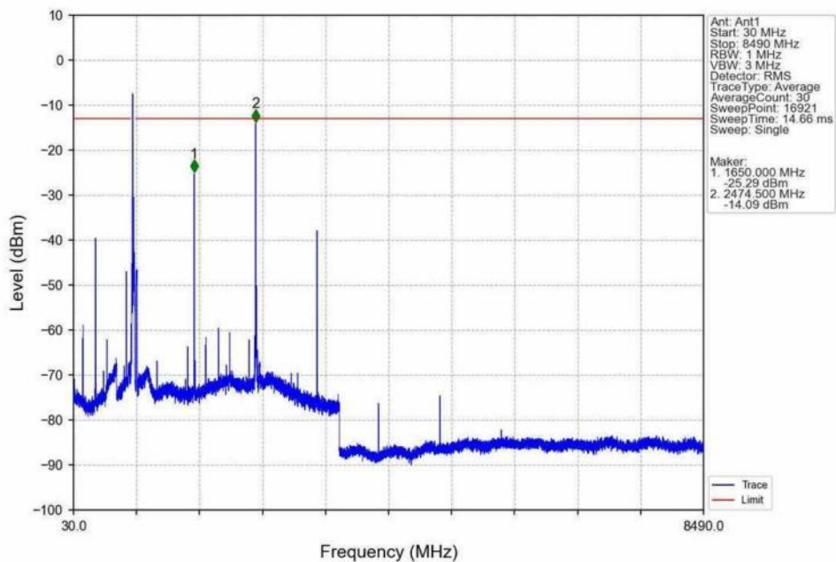
Band26b_15MHz_QPSK_LCH_831.5MHz_RB_75_0_NTNV
