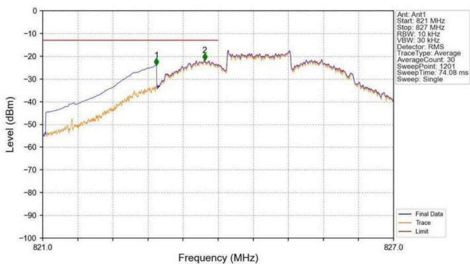
Band26b_1.4MHz_16QAM_LCH_824.7MHz_RB_6_0_NTNV
