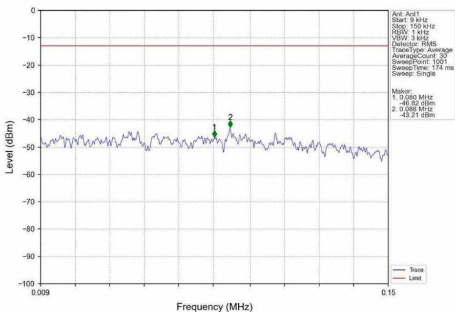
Band26b_3MHz_16QAM_LCH_825.5MHz_RB_1_0_NTNV
