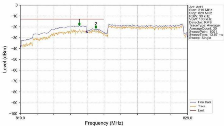
Band26b_5MHz_QPSK_LCH_826.5MHz_RB_25_0_NTNV
