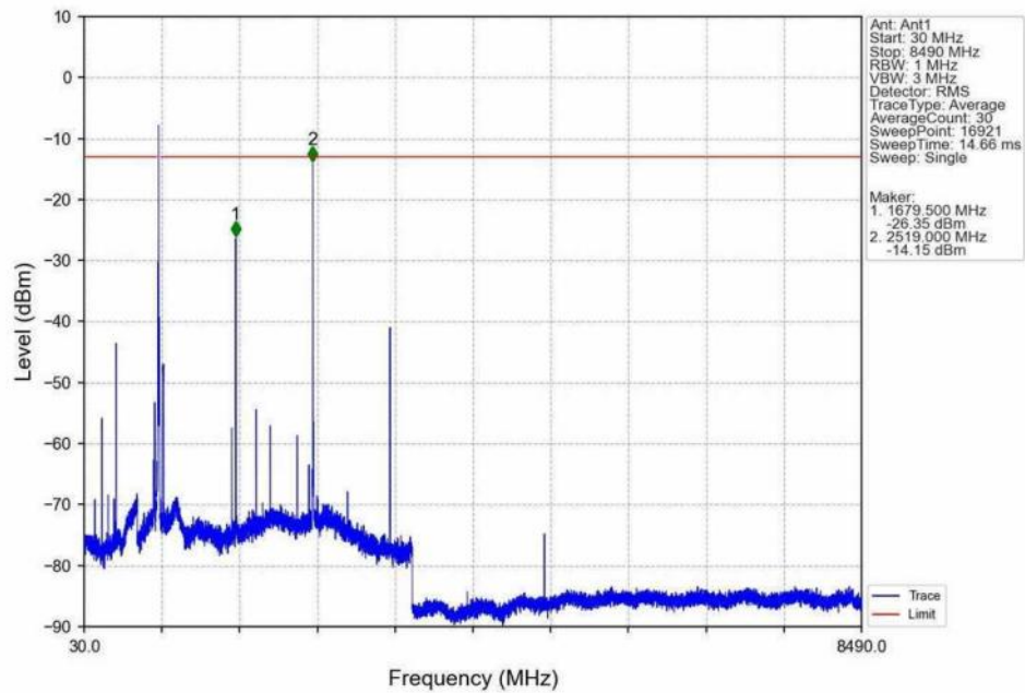
Band26b_10MHz_16QAM_HCH_844MHz_RB_1_49_NTNV
