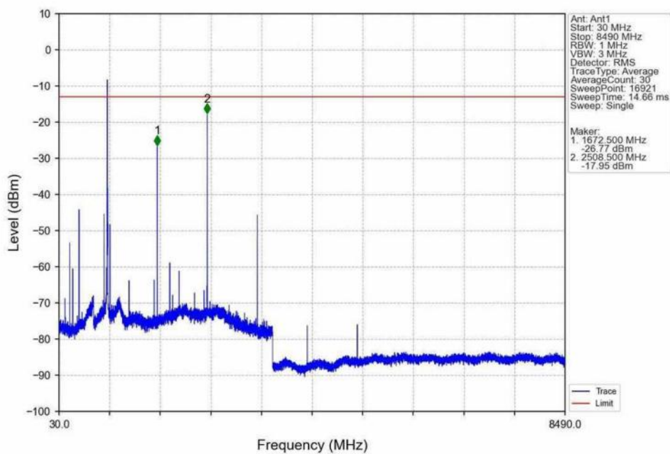
Band26b_1.4MHz_16QAM_MCH_836.5MHz_RB_1_0_NTNV
