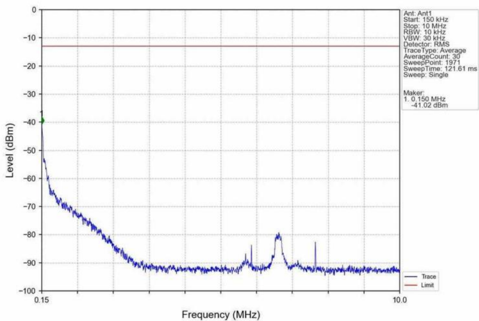
Band26b_15MHz_QPSK_HCH_841.5MHz_RB_1_0_NTNV
