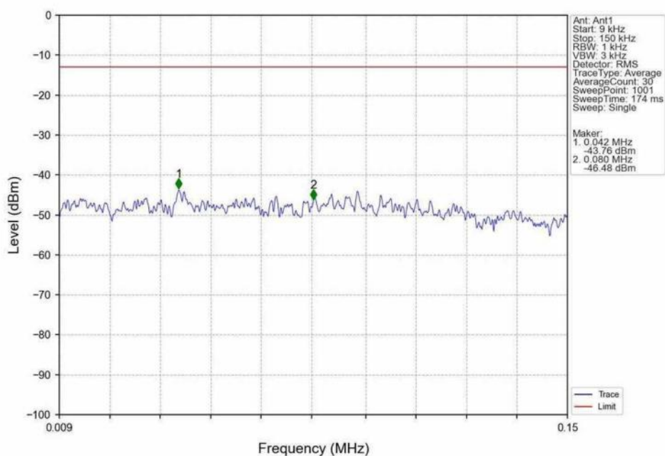
Band26b_5MHz_16QAM_LCH_826.5MHz_RB_1_0_NTNV
