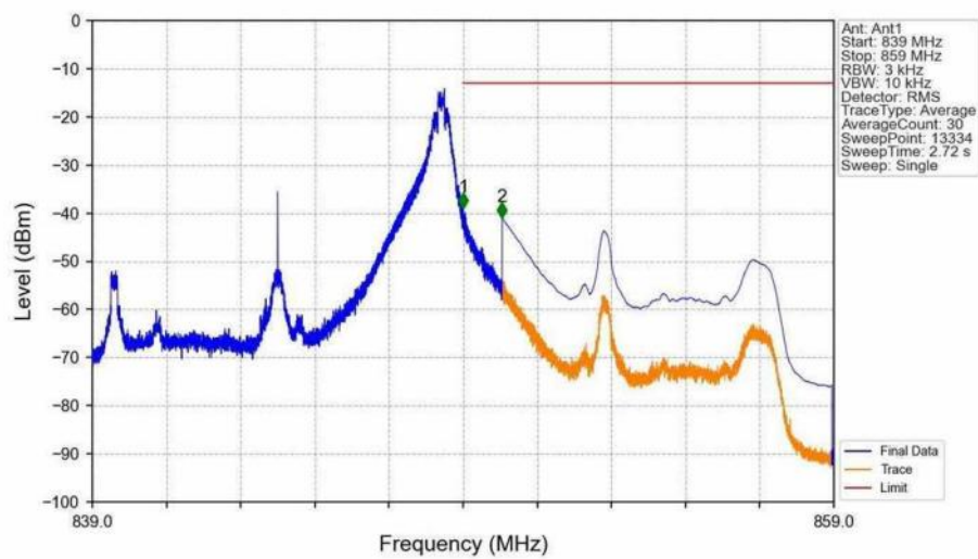
Band26b_10MHz_16QAM_HCH_844MHz_RB_1_49_NTNV
