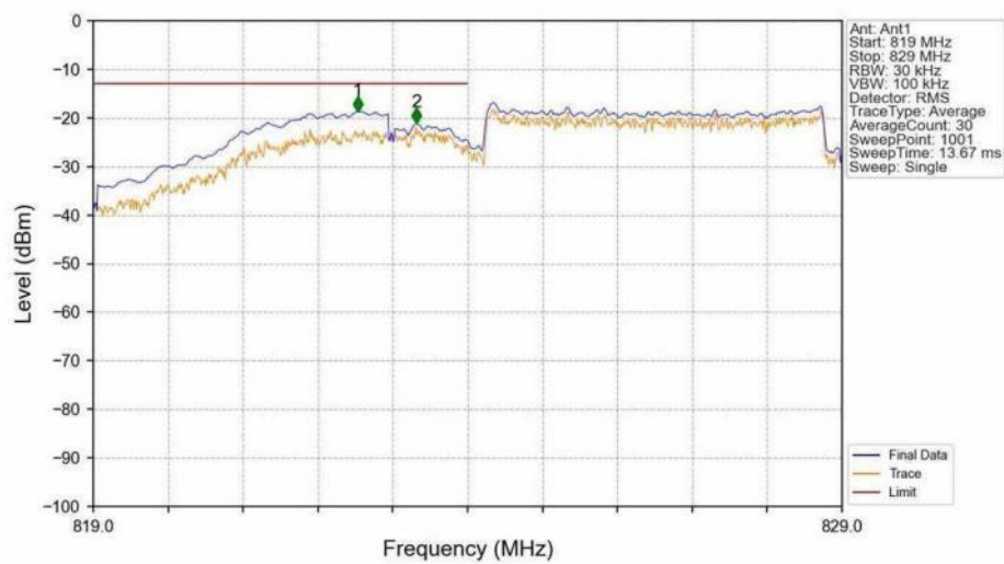
Band26b_5MHz_16QAM_LCH_826.5MHz_RB_25_0_NTNV
