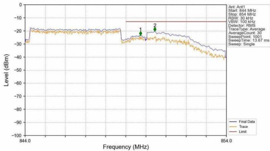
Band26b_5MHz_16QAM_HCH_846.5MHz_RB_25_0_NTNV
