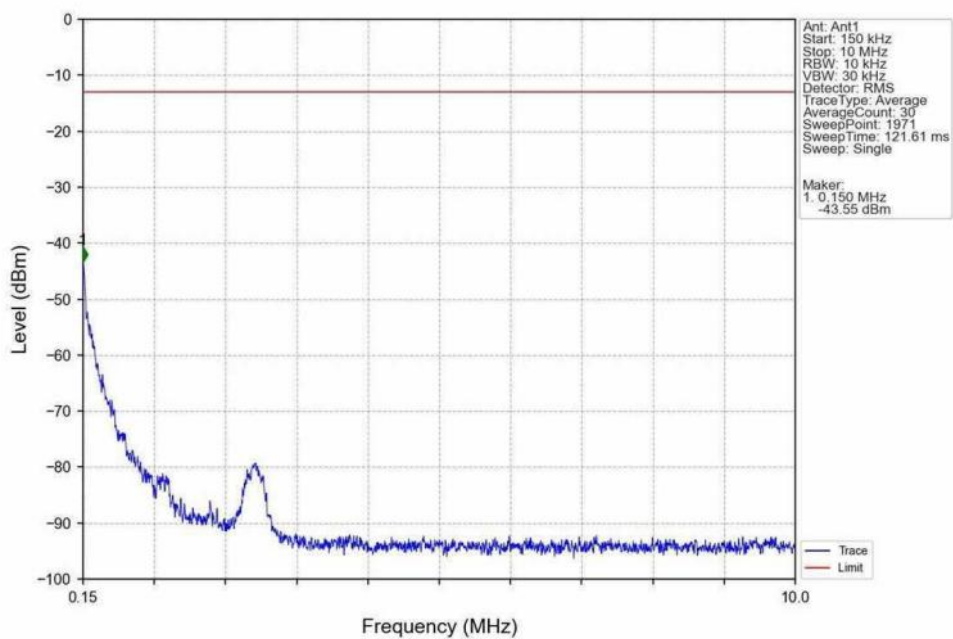
Band26b_3MHz_16QAM_MCH_836.5MHz_RB_1_0_NTNV
