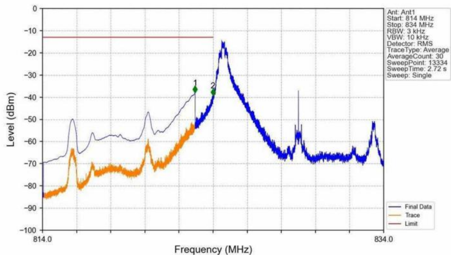
Band26b_10MHz_QPSK_LCH_829MHz_RB_1_0_NTNV
