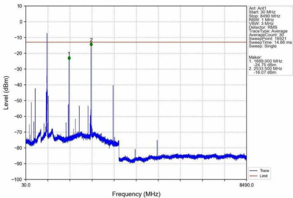
Band26b_5MHz_QPSK_HCH_846.5MHz_RB_1_0_NTNV
