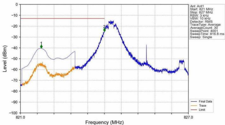
Band26b_3MHz_16QAM_LCH_825.5MHz_RB_1_0_NTNV
