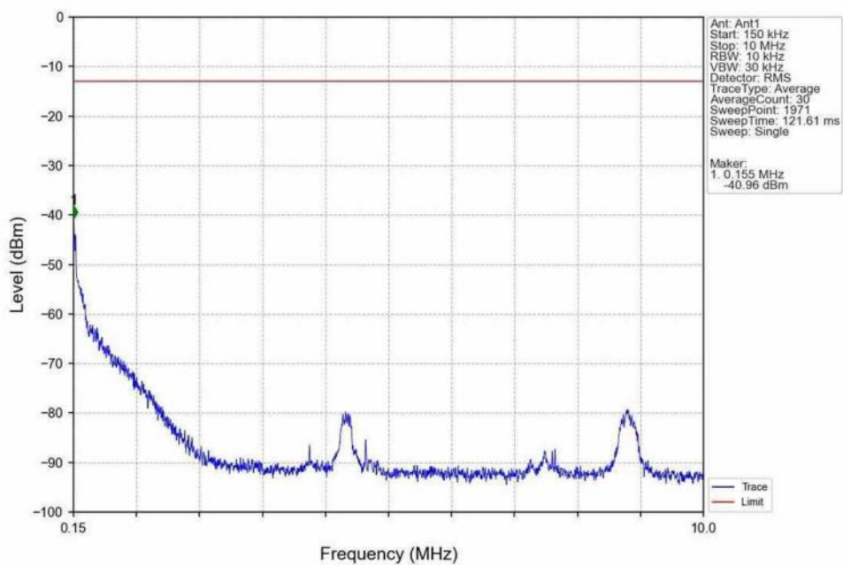
Band26b_10MHz_QPSK_MCH_836.5MHz_RB_1_0_NTNV
