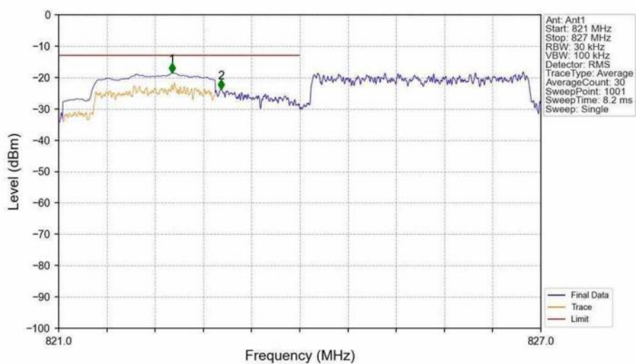
Band26b_3MHz_QPSK_LCH_825.5MHz_RB_15_0_NTNV
