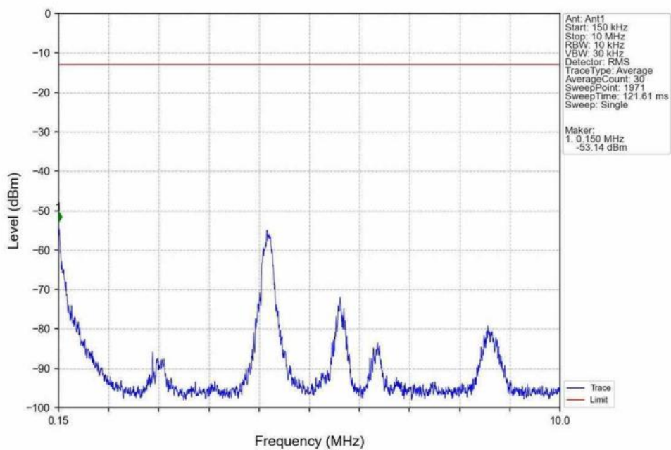
Band66_5MHz_16QAM_LCH_1712.5MHz_RB_1_0_NTNV
