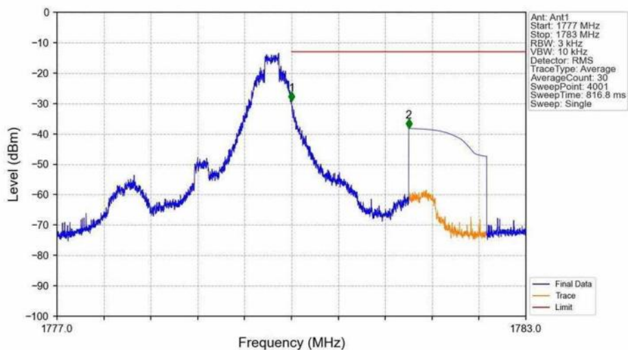
Band66_1.4MHz_16QAM_HCH_1779.3MHz_RB_1_5_NTNV
