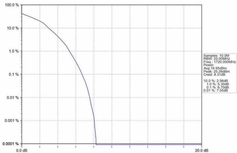
Band66_20MHz_16QAM_LCH_1720MHz_RB_27_0_NTNV
