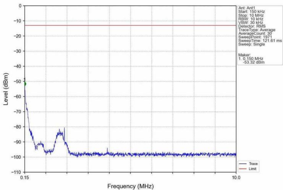
Band66_1.4MHz_QPSK_HCH_1779.3MHz_RB_1_0_NTNV
