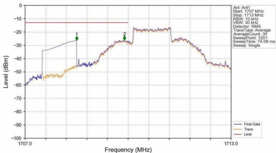
Band66_1.4MHz_QPSK_LCH_1710.7MHz_RB_6_0_NTNV
