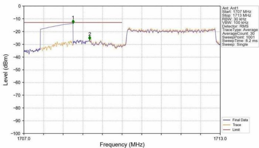
Band66_3MHz_16QAM_LCH_1711.5MHz_RB_15_0_NTNV
