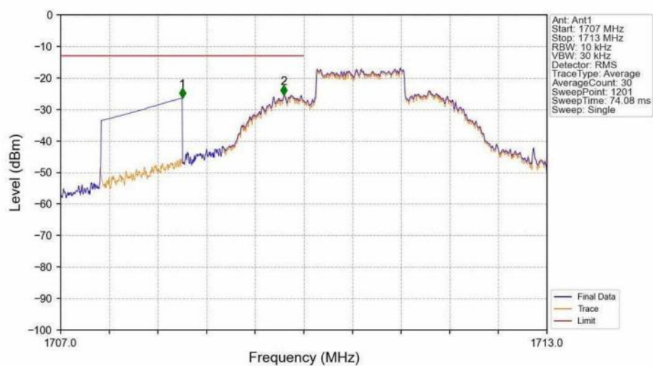
Band66_1.4MHz_16QAM_LCH_1710.7MHz_RB_6_0_NTNV
