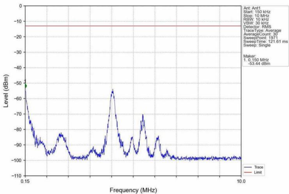
Band66_1.4MHz_16QAM_LCH_1710.7MHz_RB_1_0_NTNV
