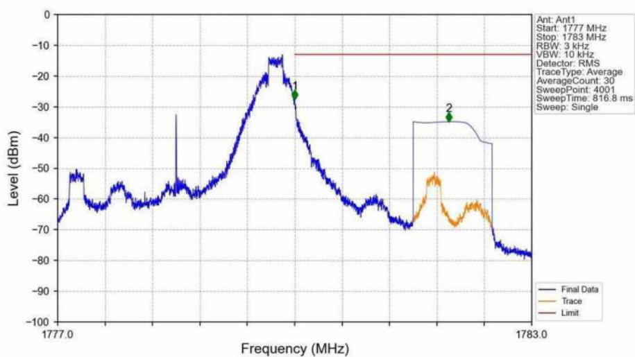
Band66_3MHz_QPSK_HCH_1778.5MHz_RB_1_14_NTNV
