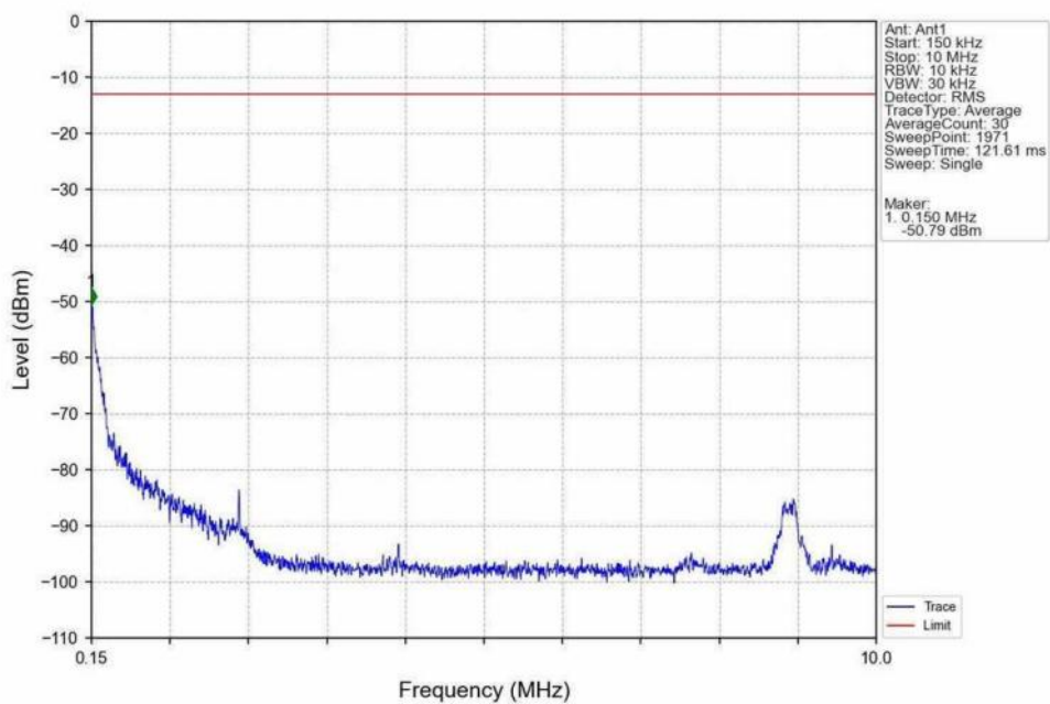
Band66_20MHz_16QAM_HCH_1770MHz_RB_1_0_NTNV
