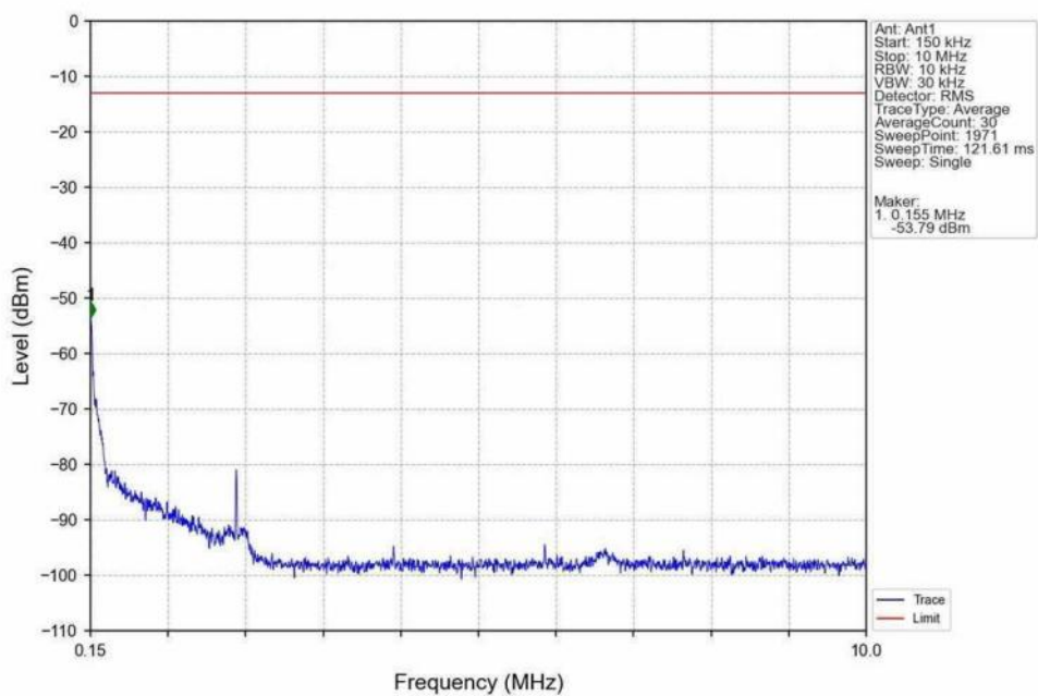
Band66_15MHz_QPSK_HCH_1772.5MHz_RB_1_0_NTNV
