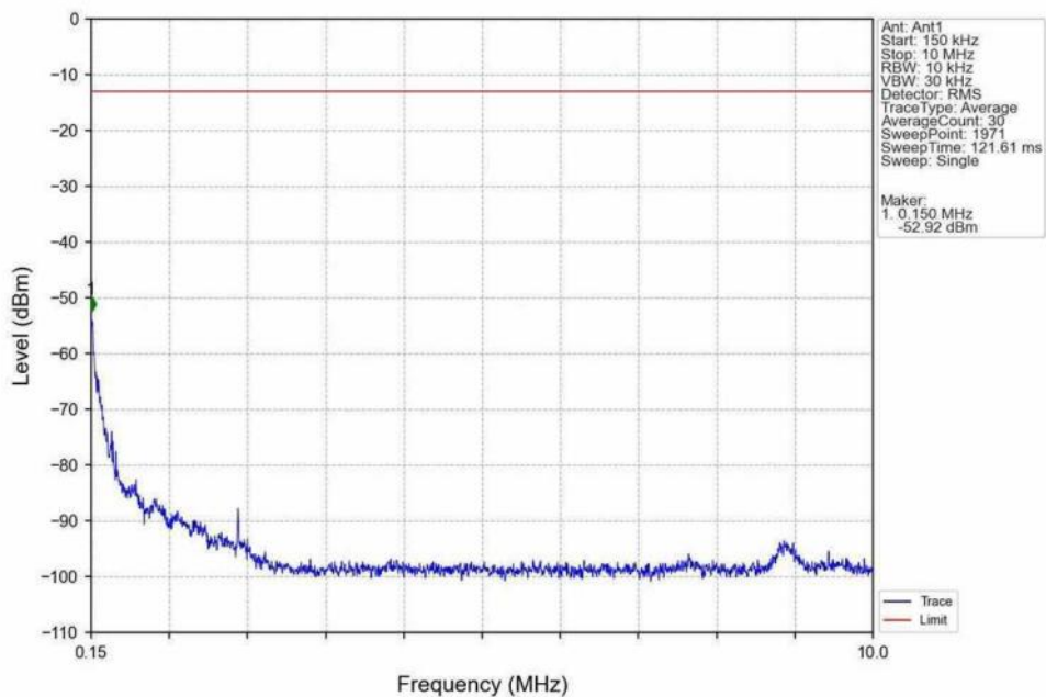
Band66_20MHz_16QAM_MCH_1745MHz_RB_1_0_NTNV
