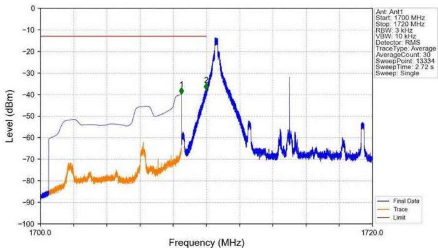
Band66_10MHz_QPSK_LCH_1715MHz_RB_1_0_NTNV
