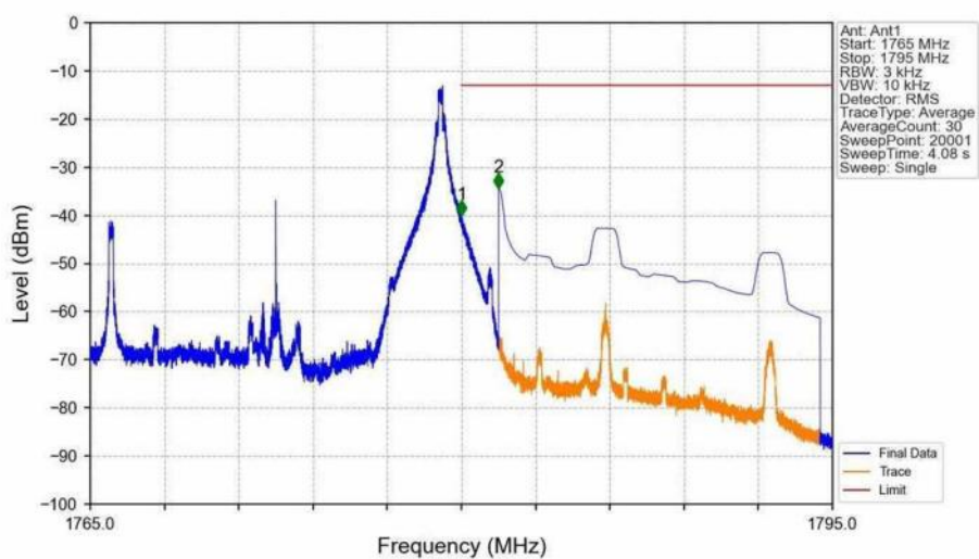
Band66_15MHz_QPSK_HCH_1772.5MHz_RB_1_74_NTNV
