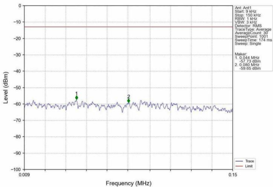
Band66_20MHz_16QAM_MCH_1745MHz_RB_1_0_NTNV
