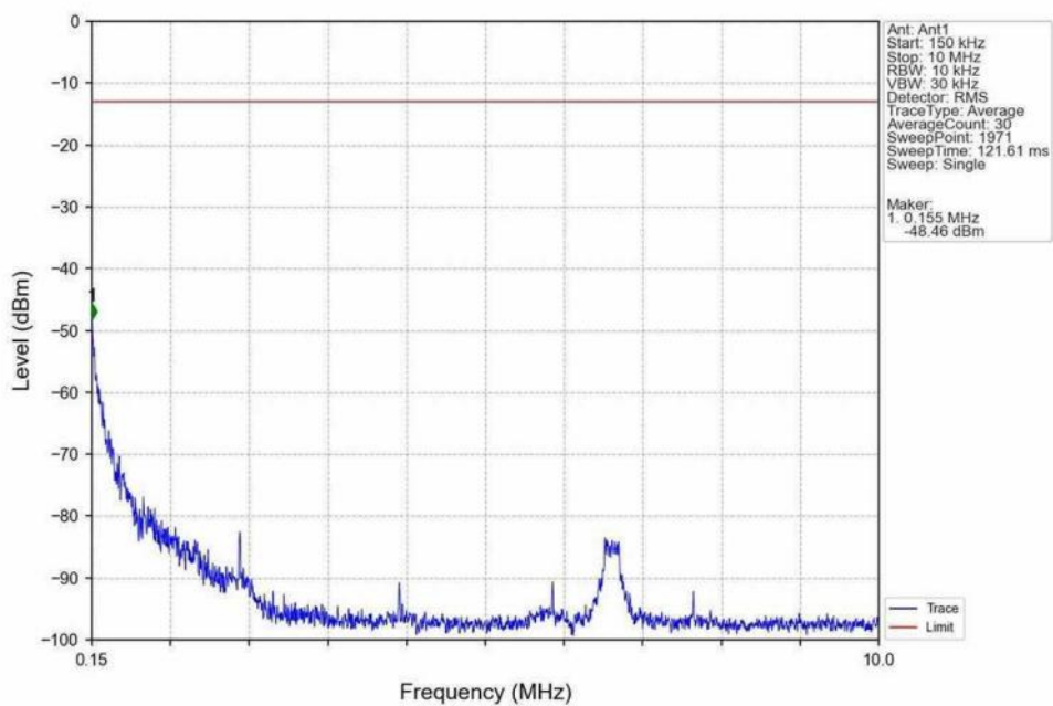
Band66_15MHz_16QAM_HCH_1772.5MHz_RB_1_0_NTNV
