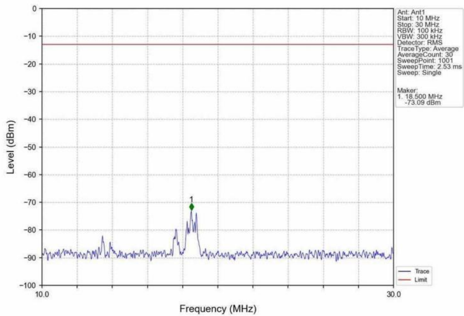
Band66_10MHz_QPSK_LCH_1715MHz_RB_1_0_NTNV
