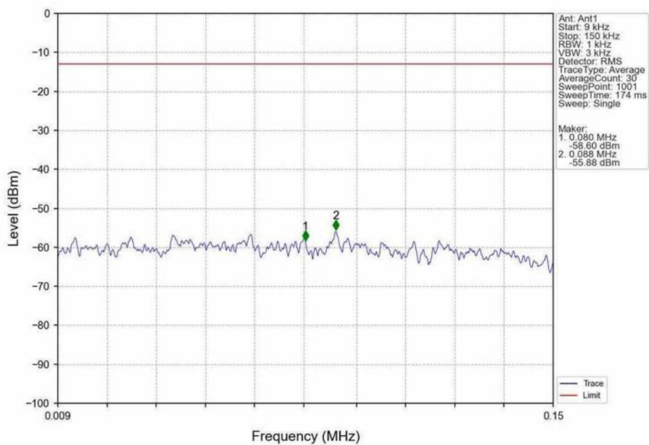
Band66_15MHz_16QAM_MCH_1745MHz_RB_1_0_NTNV
