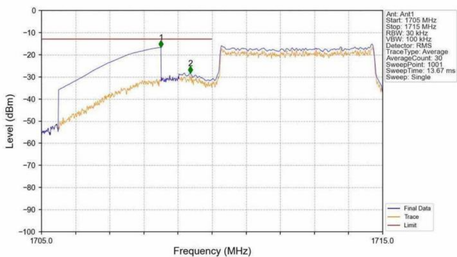
Band66_5MHz_16QAM_LCH_1712.5MHz_RB_25_0_NTNV
