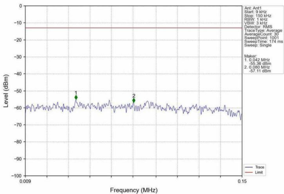
Band66_10MHz_16QAM_MCH_1745MHz_RB_1_0_NTNV
