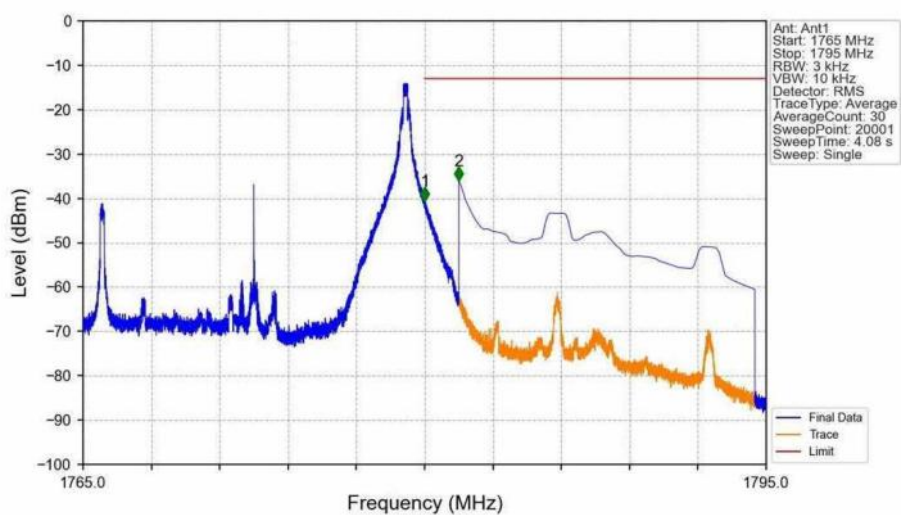
Band66_15MHz_16QAM_HCH_1772.5MHz_RB_1_74_NTNV
