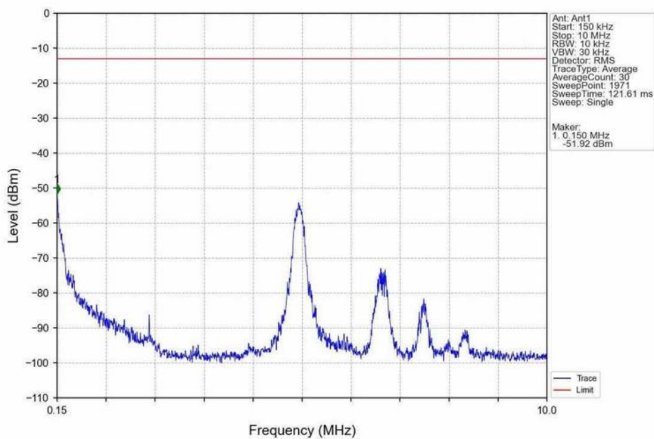
Band66_15MHz_16QAM_LCH_1717.5MHz_RB_1_0_NTNV
