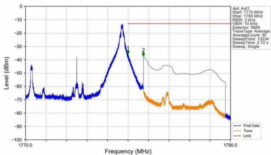
Band66_10MHz_16QAM_HCH_1775MHz_RB_1_49_NTNV
