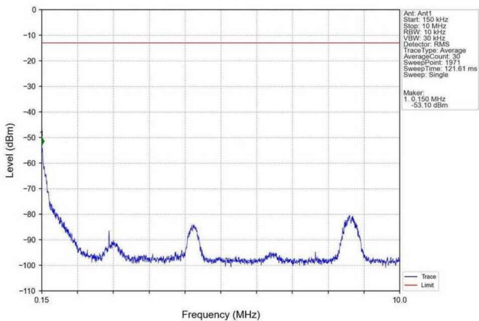
Band66_5MHz_16QAM_MCH_1745MHz_RB_1_0_NTNV
