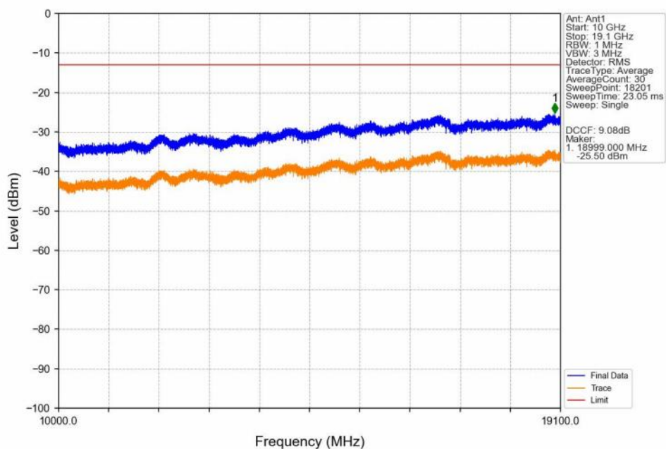
PCS1900_GSM_LCH_1850.2MHz_GSM_NTNV
