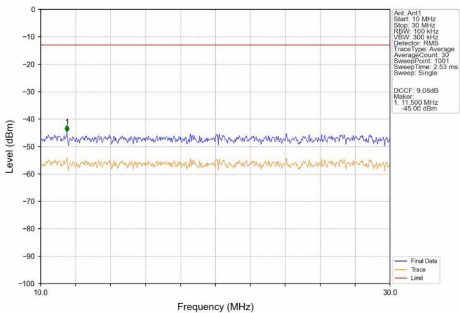
PCS1900_GSM_LCH_1850.2MHz_GSM_NTNV
