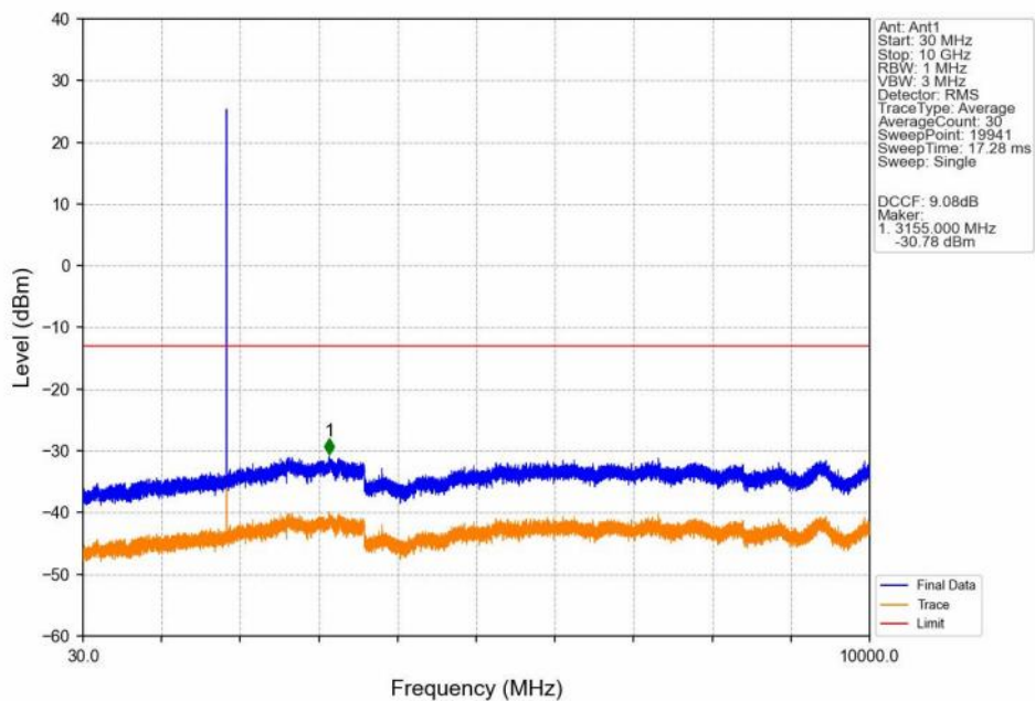
PCS1900_GSM_LCH_1850.2MHz_GSM_NTNV
