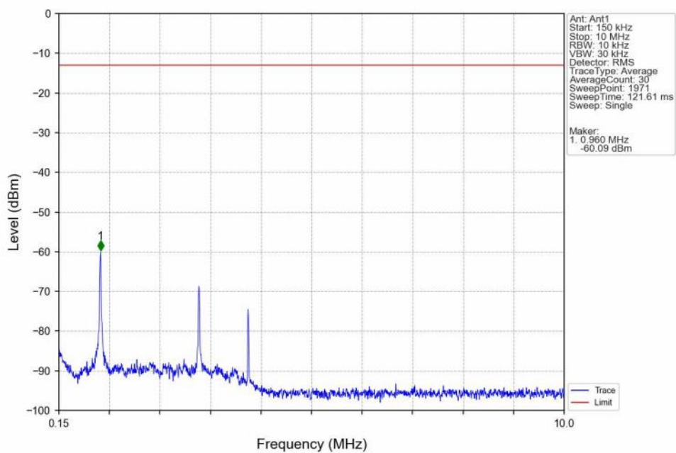
Band2_HSDPA_LCH_1852.4MHz_Subtest 1_NTNV
