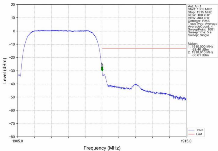
Band2_HSUPA_HCH_1907.6MHz_Subtest 1_NTNV
