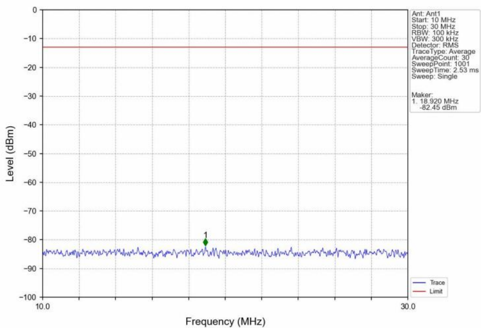
Band2_RMC_LCH_1852.4MHz_12.2kbps RMC_NTNV
