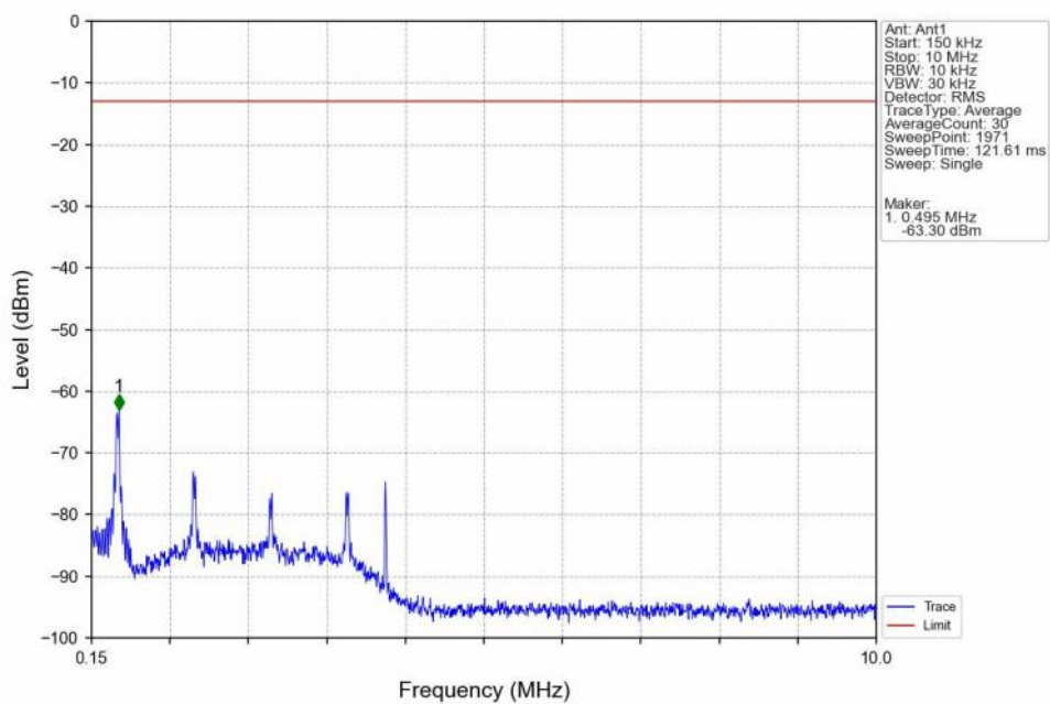
Band2_HSUPA_HCH_1907.6MHz_Subtest 1_NTNV
