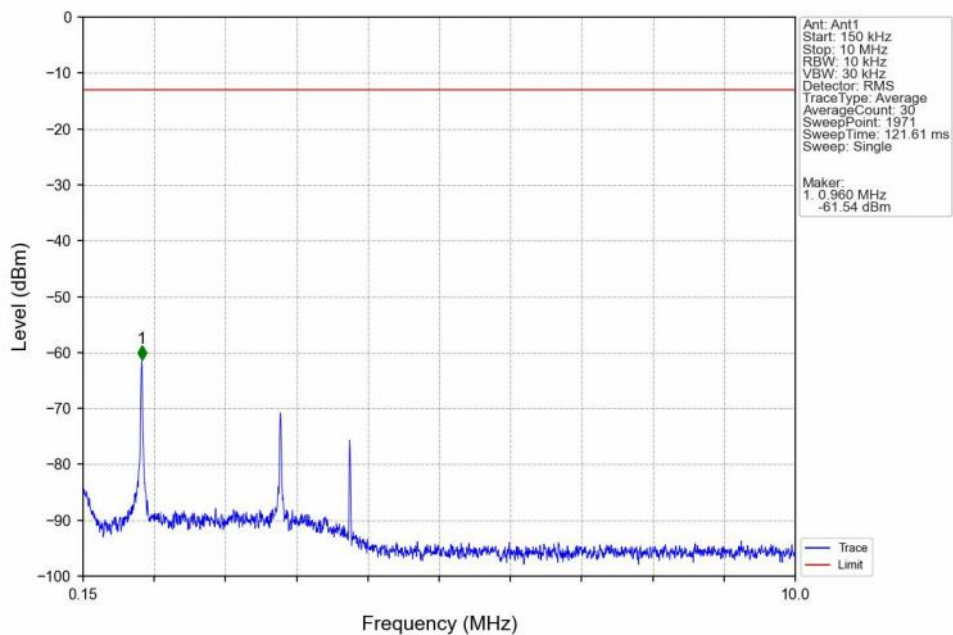
Band2_HSDPA_MCH_1880MHz_Subtest 1_NTNV
