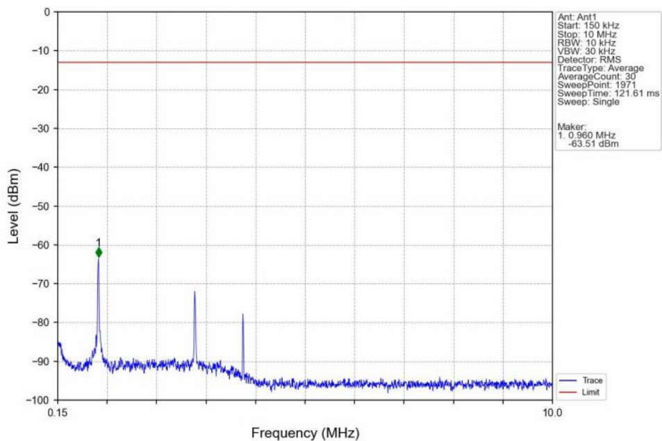
Band4_HSDPA_MCH_1732.6MHz_Subtest 1_NTNV
