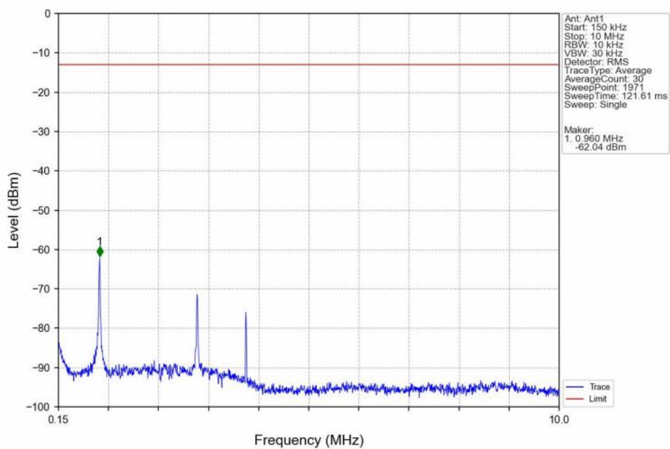
Band4_HSDPA_LCH_1712.4MHz_Subtest 1_NTNV
