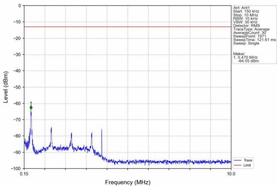
Band4_HSUPA_HCH_1752.6MHz_Subtest 1_NTNV
