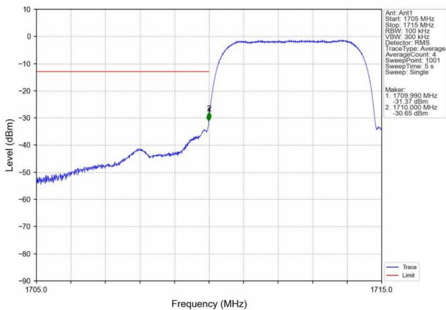
Band4_HSDPA_LCH_1712.4MHz_Subtest 1_NTNV
