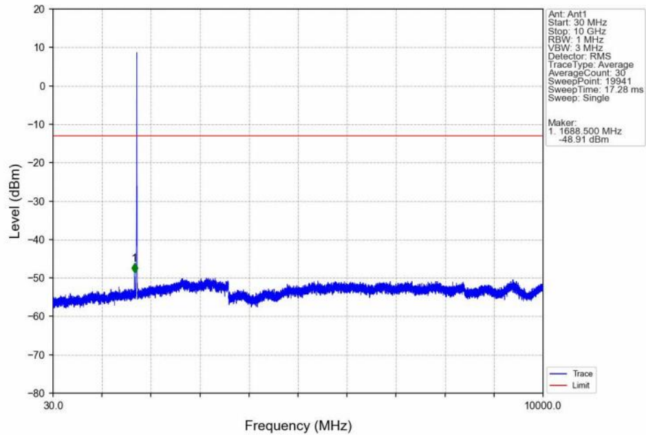
Band4_HSDPA_MCH_1732.6MHz_Subtest 1_NTNV
