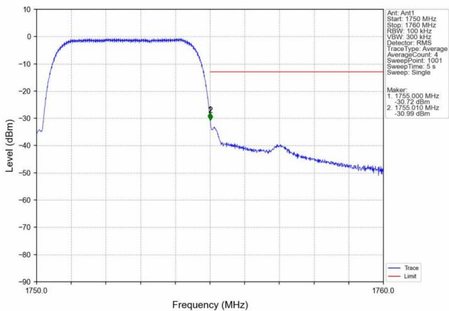
Band4_HSUPA_HCH_1752.6MHz_Subtest 1_NTNV
