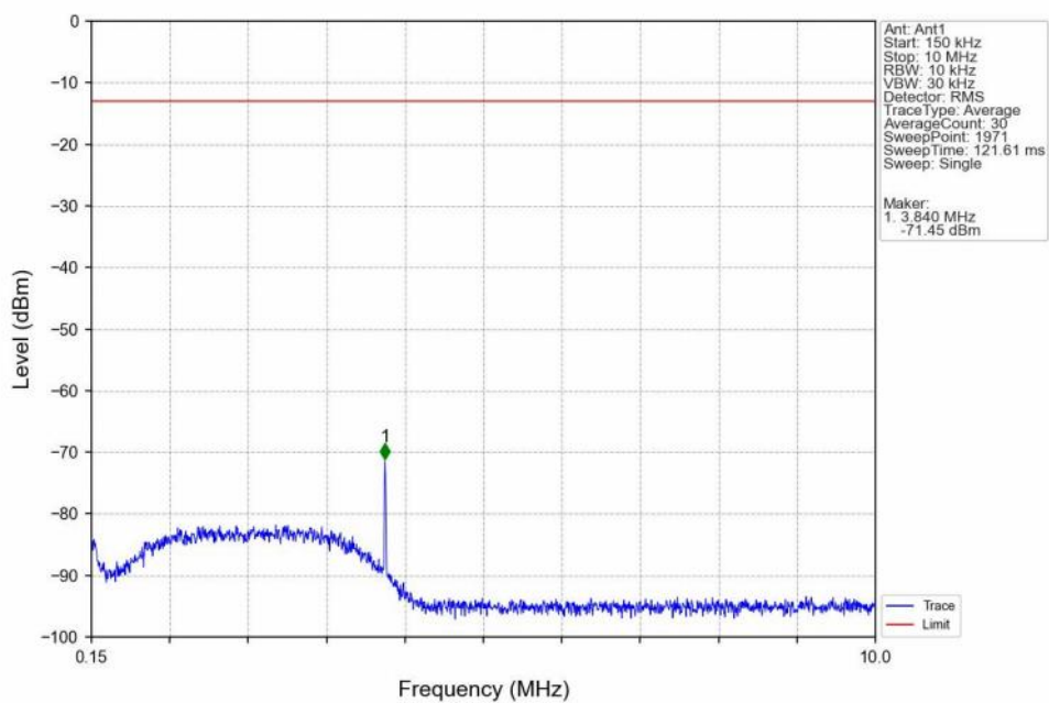
Band4_RMC_HCH_1752.6MHz_12.2kbps RMC_NTNV
