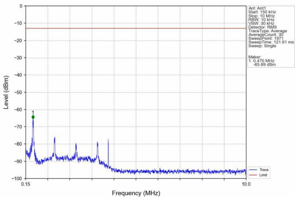
Band4_HSUPA_MCH_1732.6MHz_Subtest 1_NTNV
