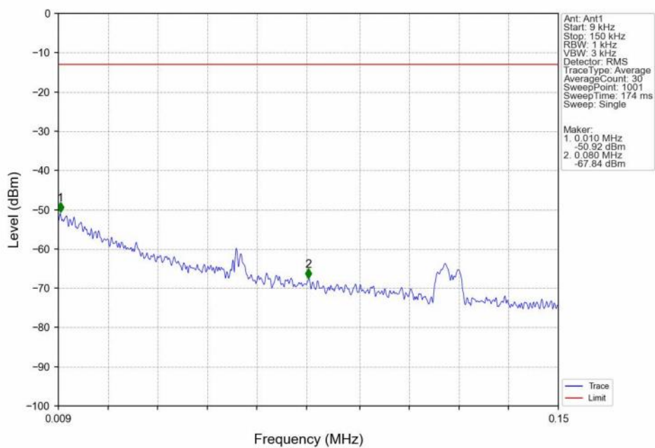
Band4_HSDPA_MCH_1732.6MHz_Subtest 1_NTNV
