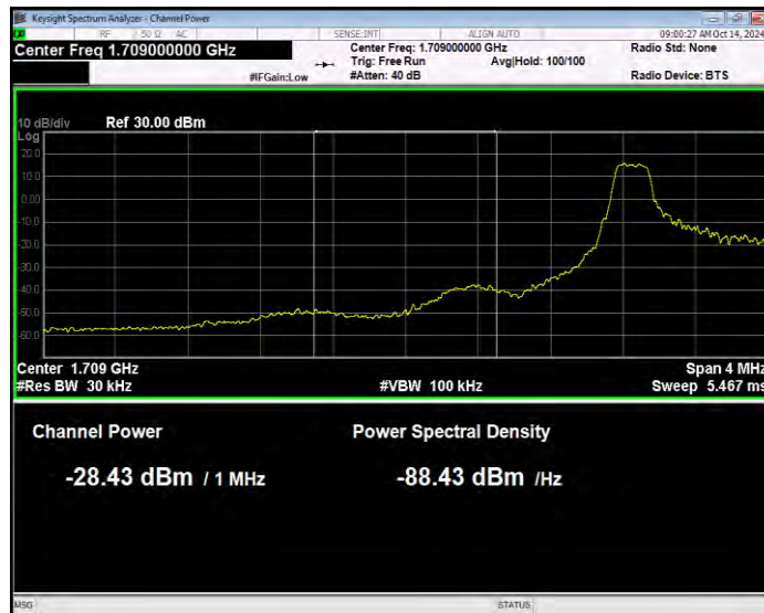
Band4 16QAM BW=1.4MHz Channel=19957 RB Size=1 Position=#0 Normal
