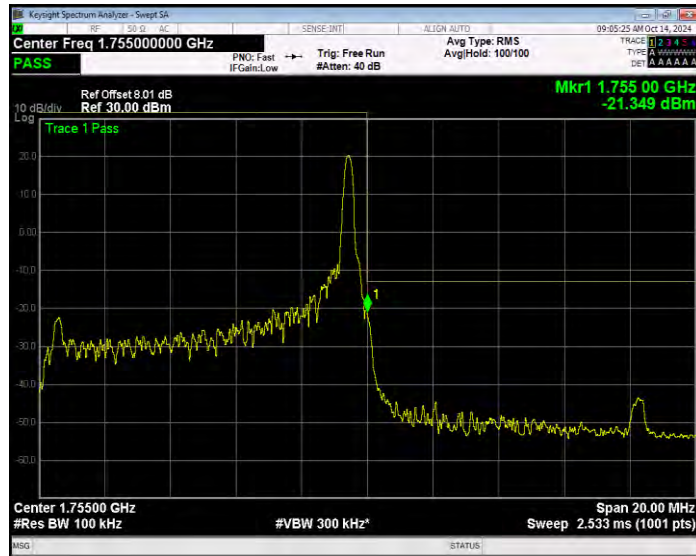
Band4 16QAM BW=10MHz Channel=20350 RB Size=50 Position=#0 Extended
