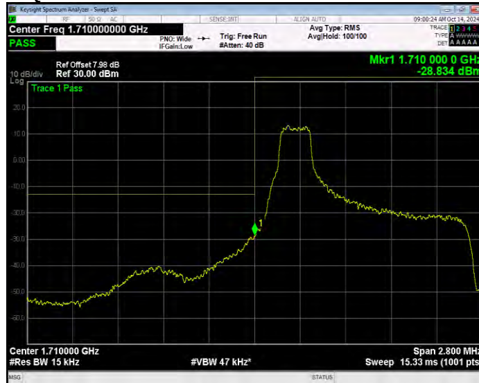
Band4 16QAM BW=1.4MHz Channel=19957 RB Size=1 Position=#Max Extended
