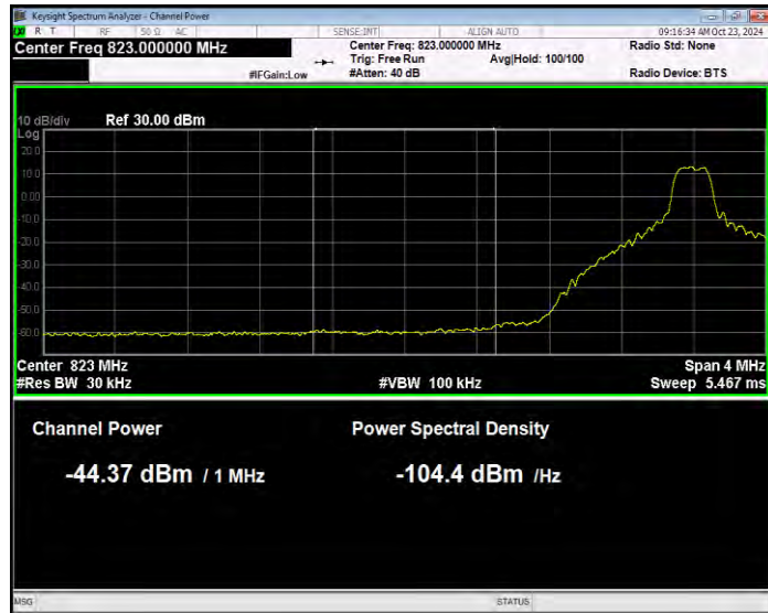
Band5 QPSK BW=10MHz Channel=20450 RB Size=1 Position=#0 Normal
