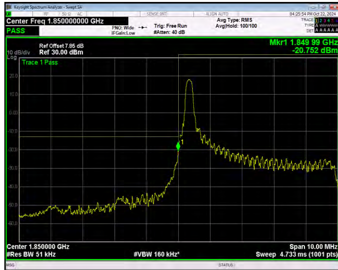
Band25 QPSK BW=5MHz Channel=26065 RB Size=1 Position=#Max Normal
