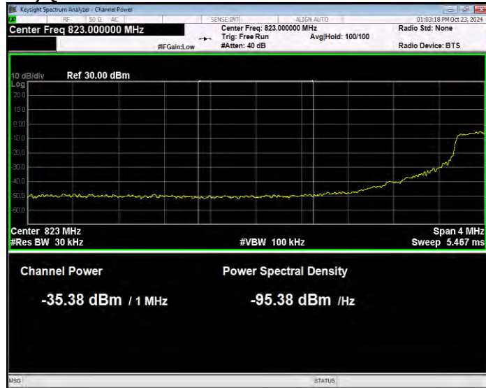
Band26(824-849) QPSK BW=15MHz Channel=26865 RB Size=75 Position=#0 Normal
