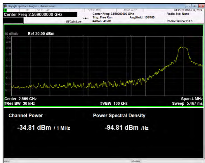
Band38 16QAM BW=10MHz Channel=37800 RB Size=1 Position=#0 Normal
