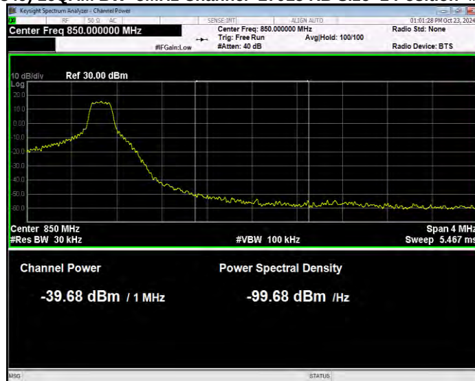
Band26(824-849) 16QAM BW=5MHz Channel=27015 RB Size=1 Position=#Max Normal
