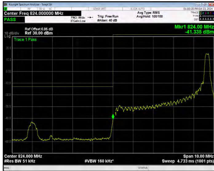
Band26(824-849) QPSK BW=5MHz Channel=26815 RB Size=25 Position=#0 Extended
