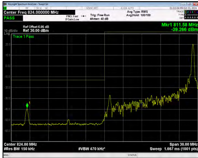
Band26(824-849) QPSK BW=15MHz Channel=26865 RB Size=75 Position=#0 Extended
