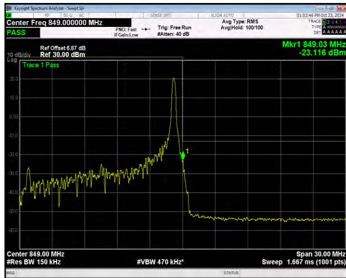
Band26(824-849) QPSK BW=15MHz Channel=26965 RB Size=75 Position=#0 Extended
