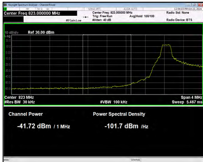
Band26(824-849) QPSK BW=3MHz Channel=26805 RB Size=1 Position=#0 Normal
