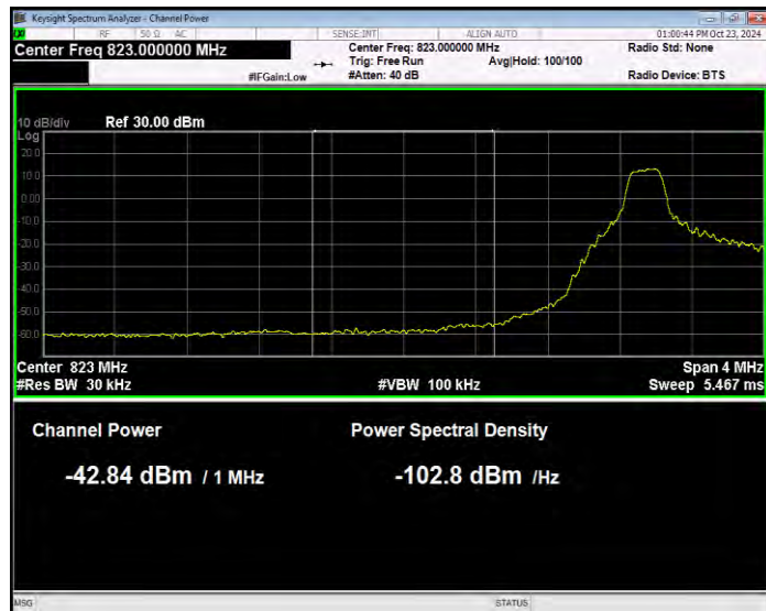
Band26(824-849) 16QAM BW=5MHz Channel=26815 RB Size=1 Position=#0 Normal
