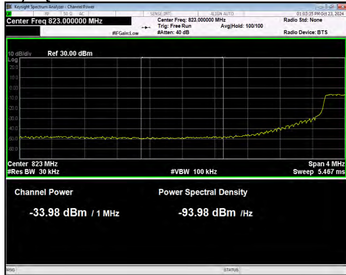
Band26(824-849) 16QAM BW=15MHz Channel=26865 RB Size=75 Position=#0 Normal
