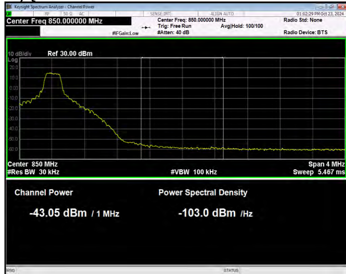
Band26(824-849) QPSK BW=10MHz Channel=26990 RB Size=1 Position=#Max Normal
