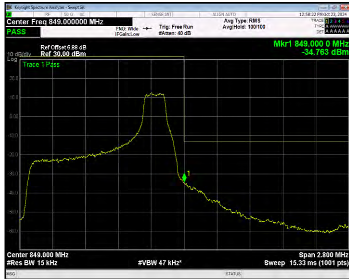
Band26(824-849) QPSK BW=1.4MHz Channel=27033 RB Size=6 Position=#0 Extended
