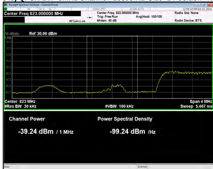
Band26(824-849) QPSK BW=3MHz Channel=26805 RB Size=1 Position=#Max Normal
