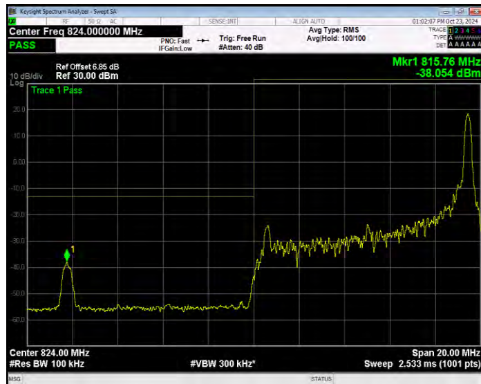
Band26(824-849) 16QAM BW=10MHz Channel=26840 RB Size=50 Position=#0 Extended
