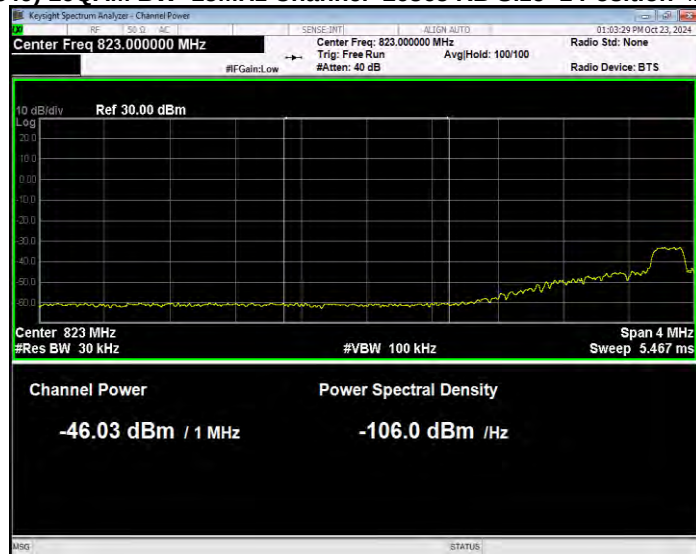
Band26(824-849) 16QAM BW=15MHz Channel=26865 RB Size=1 Position=#Max Normal
