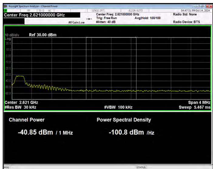
Band38 16QAM BW=15MHz Channel=38175 RB Size=1 Position=#0 Normal
