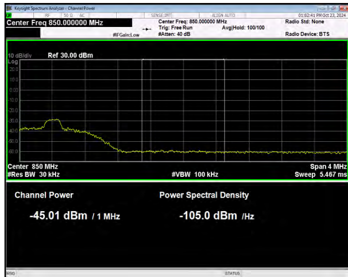
Band26(824-849) 16QAM BW=10MHz Channel=26990 RB Size=1 Position=#0 Normal
