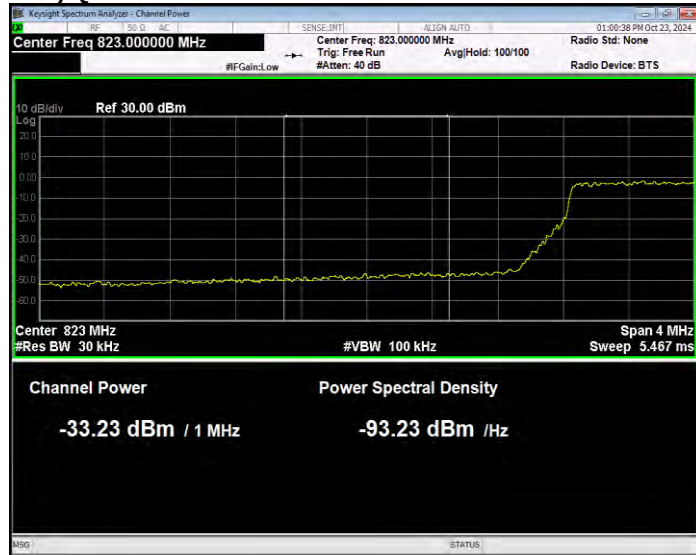
Band26(824-849) QPSK BW=5MHz Channel=26815 RB Size=25 Position=#0 Normal
