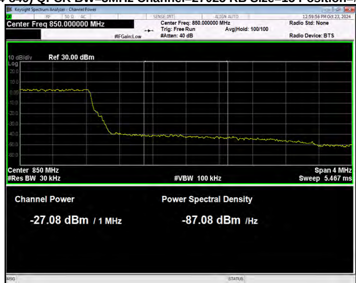
Band26(824-849) QPSK BW=3MHz Channel=27025 RB Size=15 Position=#0 Normal
