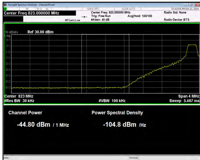
Band26(824-849) QPSK BW=15MHz Channel=26865 RB Size=1 Position=#0 Normal
