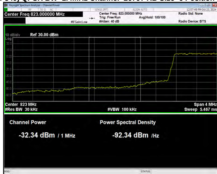
Band26(824-849) QPSK BW=1.4MHz Channel=26797 RB Size=6 Position=#0 Normal
