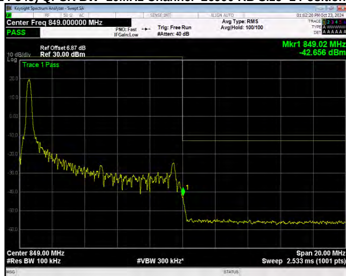
Band26(824-849) QPSK BW=10MHz Channel=26990 RB Size=1 Position=#Max Extended
