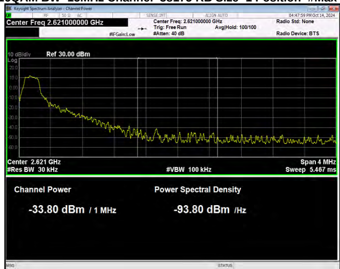
Band38 16QAM BW=15MHz Channel=38175 RB Size=1 Position=#Max Normal
