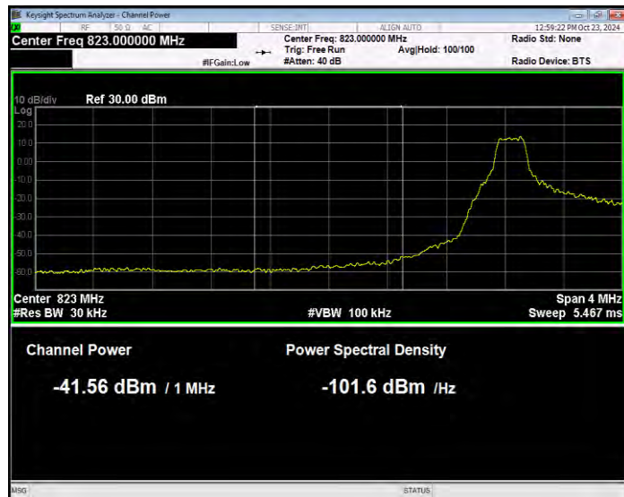
Band26(824-849) 16QAM BW=3MHz Channel=26805 RB Size=1 Position=#0 Normal
