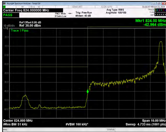
Band26(824-849) 16QAM BW=5MHz Channel=26815 RB Size=25 Position=#0 Extended
