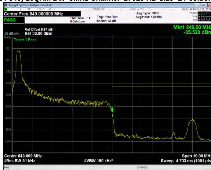
Band26(824-849) 16QAM BW=5MHz Channel=27015 RB Size=1 Position=#Max Extended
