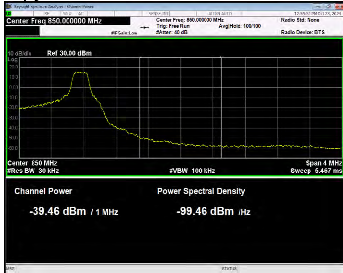
Band26(824-849) QPSK BW=3MHz Channel=27025 RB Size=1 Position=#Max Normal
