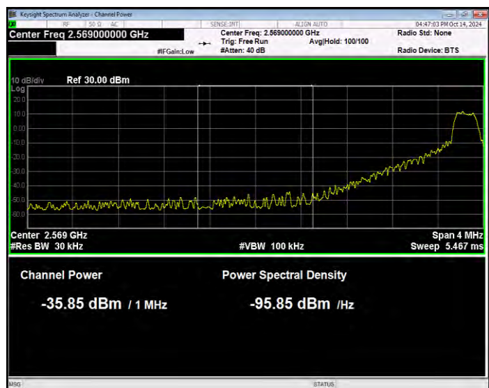
Band38 16QAM BW=15MHz Channel=37825 RB Size=1 Position=#0 Normal
