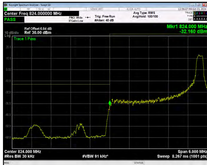
Band26(824-849) QPSK BW=3MHz Channel=26805 RB Size=15 Position=#0 Extended
