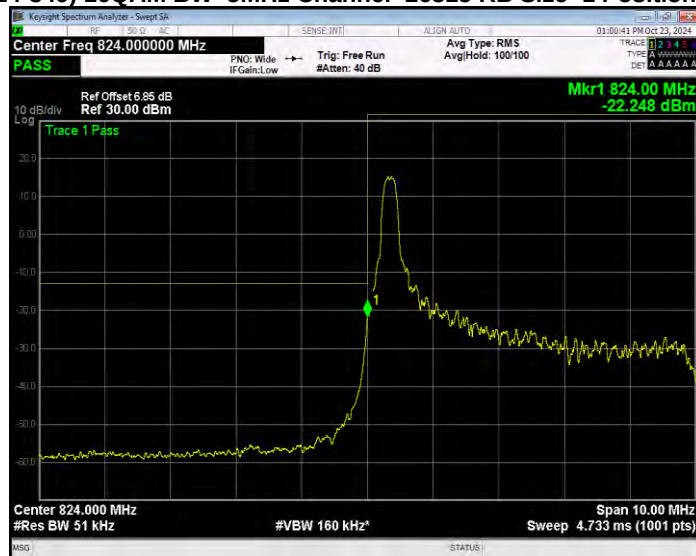
Band26(824-849) 16QAM BW=5MHz Channel=26815 RB Size=1 Position=#Max Extended
