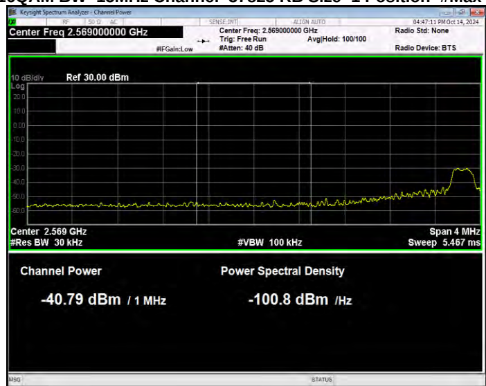
Band38 16QAM BW=15MHz Channel=37825 RB Size=1 Position=#Max Normal
