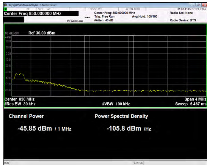
Band26(824-849) QPSK BW=15MHz Channel=26965 RB Size=1 Position=#0 Normal
