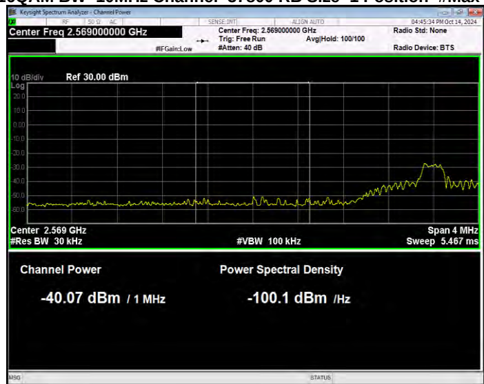
Band38 16QAM BW=10MHz Channel=37800 RB Size=1 Position=#Max Normal
