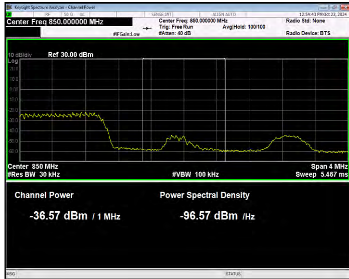
Band26(824-849) QPSK BW=3MHz Channel=27025 RB Size=1 Position=#0 Normal
