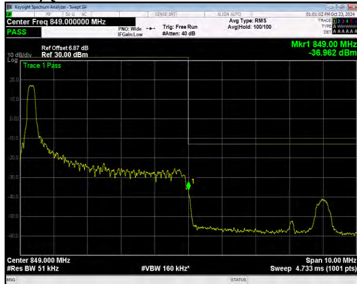
Band26(824-849) QPSK BW=5MHz Channel=27015 RB Size=1 Position=#Max Extended
