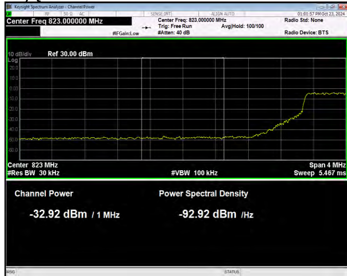
Band26(824-849) QPSK BW=10MHz Channel=26840 RB Size=50 Position=#0 Normal
