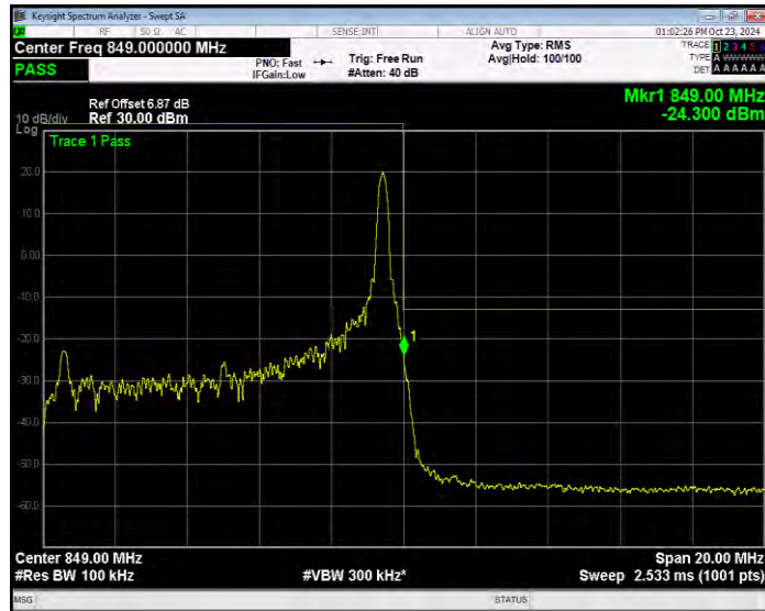
Band26(824-849) QPSK BW=10MHz Channel=26990 RB Size=50 Position=#0 Extended
