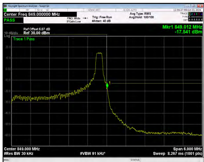
Band26(824-849) QPSK BW=3MHz Channel=27025 RB Size=15 Position=#0 Extended
