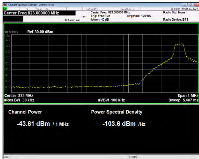
Band26(824-849) 16QAM BW=10MHz Channel=26840 RB Size=1 Position=#0 Normal
