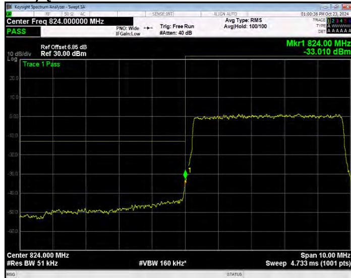
Band26(824-849) QPSK BW=5MHz Channel=27015 RB Size=1 Position=#0 Extended
