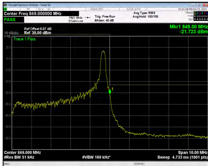
Band26(824-849) QPSK BW=5MHz Channel=27015 RB Size=25 Position=#0 Extended
