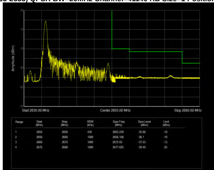
Band41(2535-2655) QPSK BW=20MHz Channel=41140 RB Size=1 Position=#Max Extended
