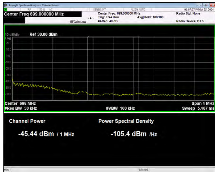
Band71 16QAM BW=20MHz Channel=133372 RB Size=1 Position=#0 Normal
