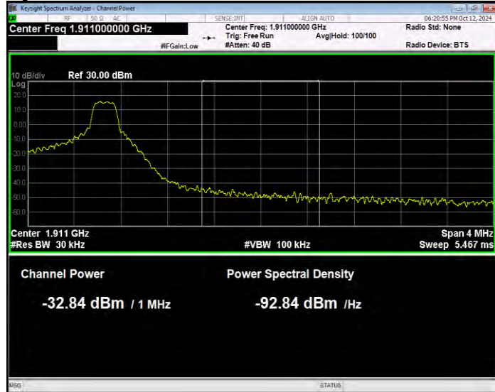
Band2 16QAM BW=5MHz Channel=19175 RB Size=1 Position=#Max Normal
