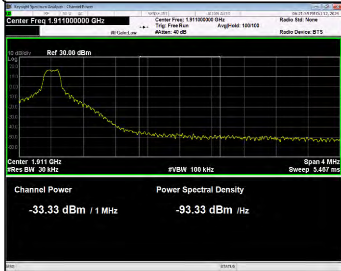
Band2 QPSK BW=10MHz Channel=19150 RB Size=1 Position=#Max Normal
