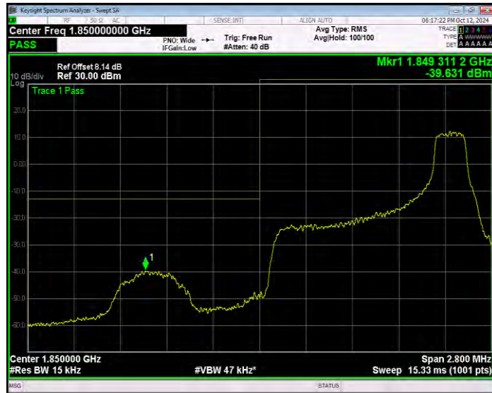
Band2 16QAM BW=1.4MHz Channel=18607 RB Size=6 Position=#0 Extended
