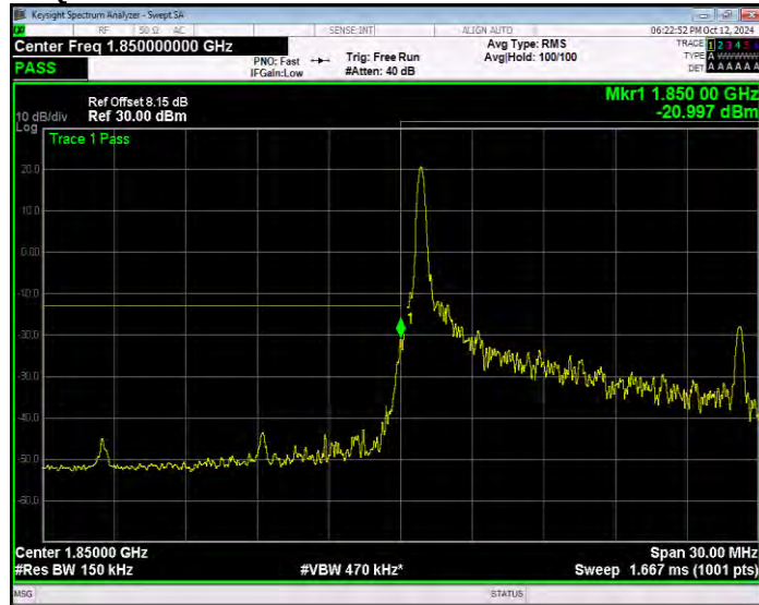
Band2 16QAM BW=15MHz Channel=18675 RB Size=1 Position=#Max Extended
