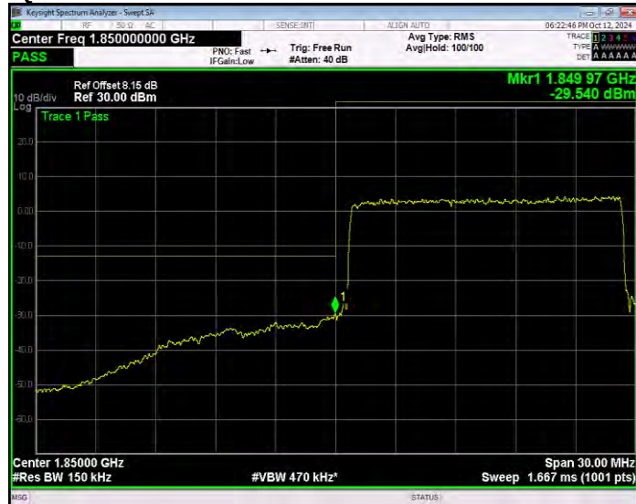
Band2 QPSK BW=15MHz Channel=19125 RB Size=1 Position=#0 Extended
