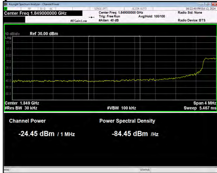
Band2 QPSK BW=15MHz Channel=18675 RB Size=75 Position=#0 Normal
