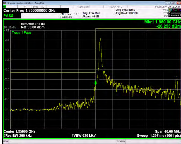
Band2 16QAM BW=20MHz Channel=18700 RB Size=1 Position=#Max Extended
