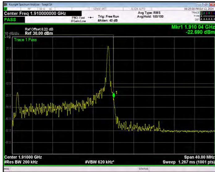
Band2 16QAM BW=20MHz Channel=19100 RB Size=100 Position=#0 Extended
