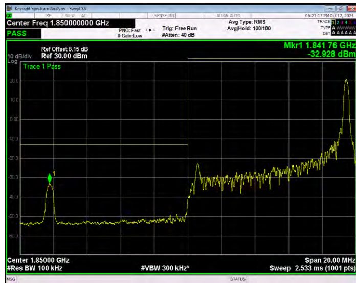
Band2 QPSK BW=10MHz Channel=18650 RB Size=50 Position=#0 Extended
