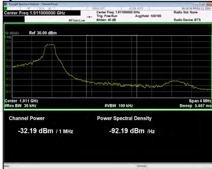
Band2 16QAM BW=3MHz Channel=19185 RB Size=1 Position=#Max Normal
