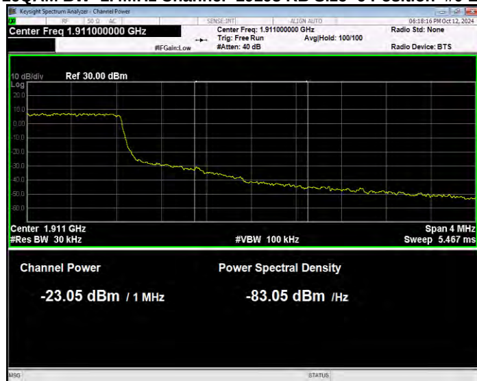
Band2 16QAM BW=1.4MHz Channel=19193 RB Size=6 Position=#0 Normal
