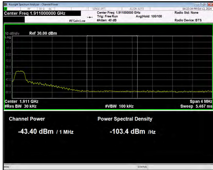
Band2 16QAM BW=15MHz Channel=19125 RB Size=1 Position=#0 Normal
