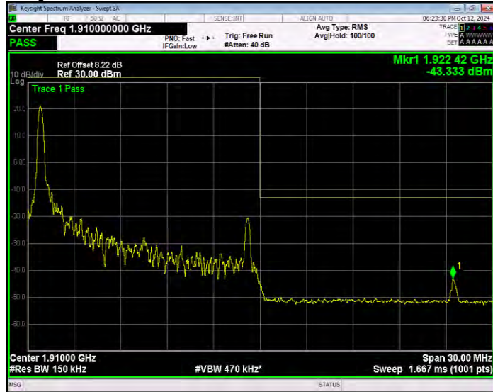
Band2 16QAM BW=15MHz Channel=19125 RB Size=1 Position=#Max Extended
