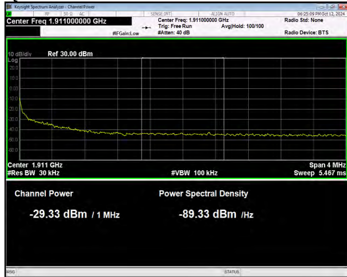
Band2 16QAM BW=20MHz Channel=19100 RB Size=100 Position=#0 Normal
