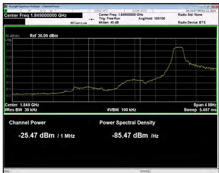
Band2 QPSK BW=1.4MHz Channel=18607 RB Size=1 Position=#0 Normal
