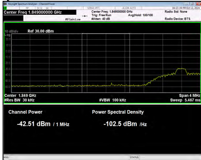
Band2 16QAM BW=10MHz Channel=18650 RB Size=1 Position=#Max Normal
