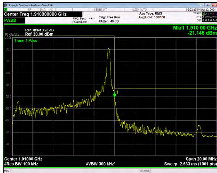
Band2 16QAM BW=10MHz Channel=19150 RB Size=50 Position=#0 Extended
