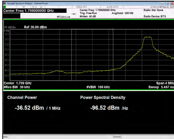
Band4 16QAM BW=5MHz Channel=19975 RB Size=1 Position=#Max Extended
