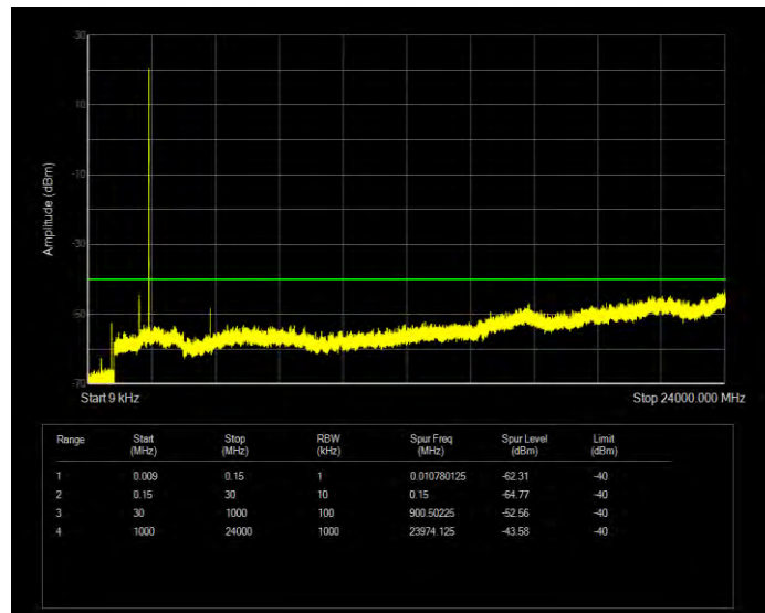
Band30 QPSK BW=10MHz Channel=27710 RB Size=1 Position=#0
