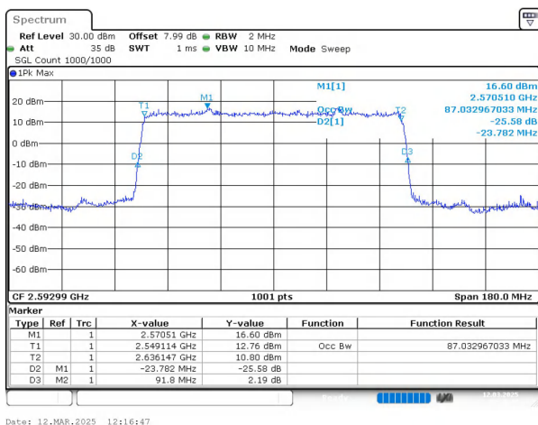
n41 SCS=30kHz DFT_BPSK BW=90MHz Channel=518598 RB=243@0
