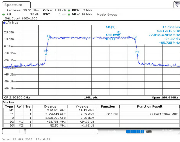
n41 SCS=30kHz CP_64QAM BW=80MHz Channel=518598 RB=217@0
