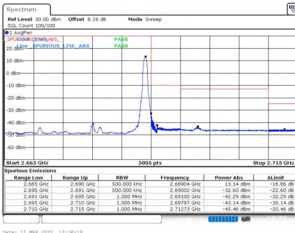
n41 SCS=30kHz DFT_64QAM BW=20MHz HighChannel=535998 RB=1@50
