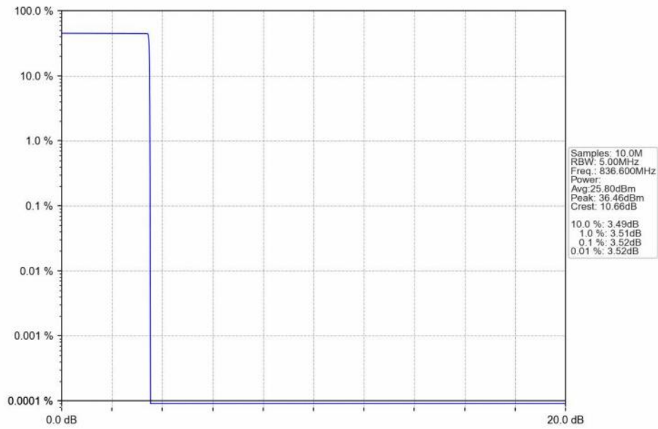
GSM850 GPRS MCH 836.6MHz 4 TX Slots NTV
