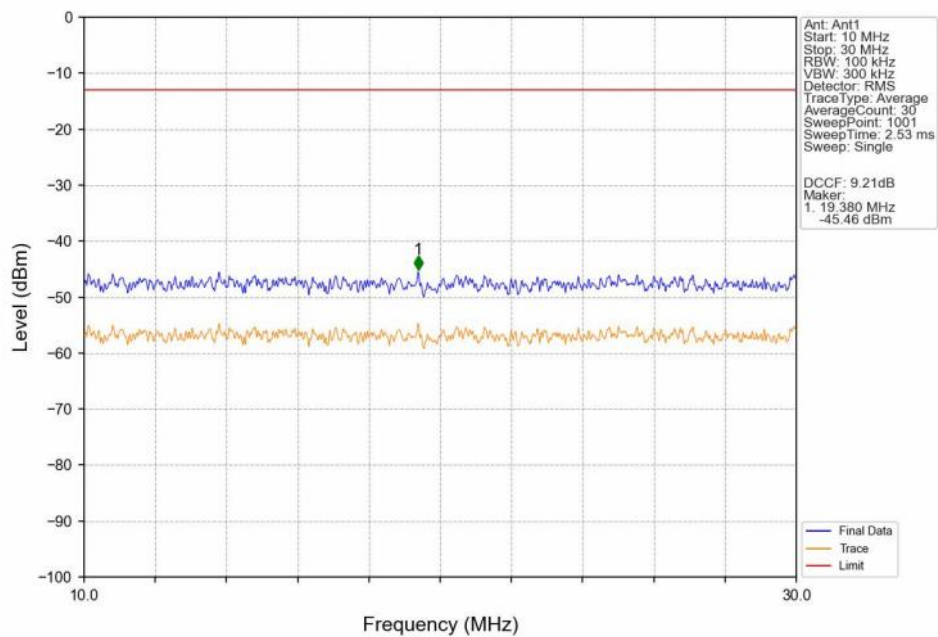
GSM850 EGPRS LCH 824.2MHz 1 TX Slot NTN
