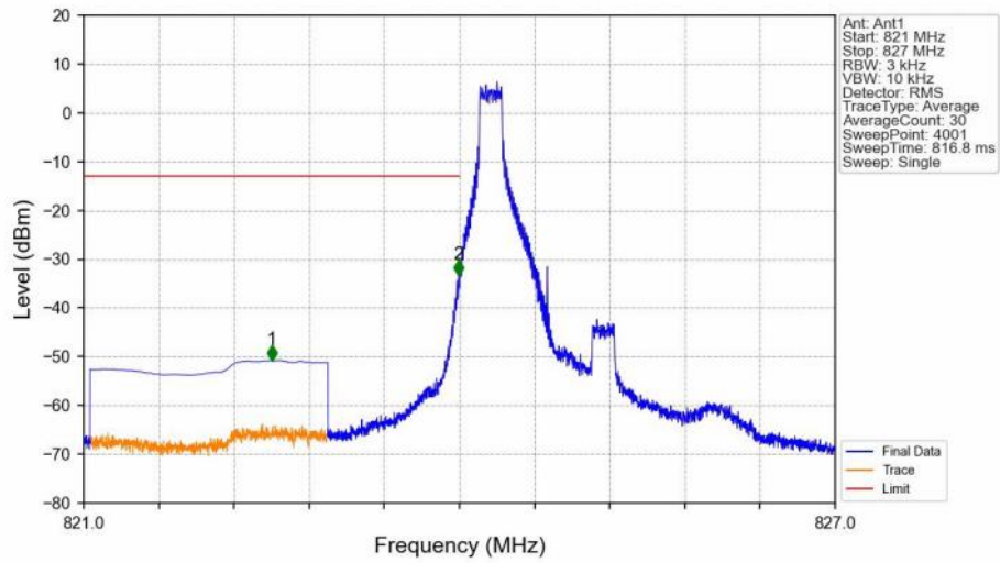
Band26b 1.4MHz 16QAM LCH 824.7MHz RB 1 0 NTNV
