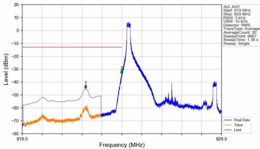
Band26b_5MHz_16QAM_LCH_826.5MHz_RB_1_0_NTNV
