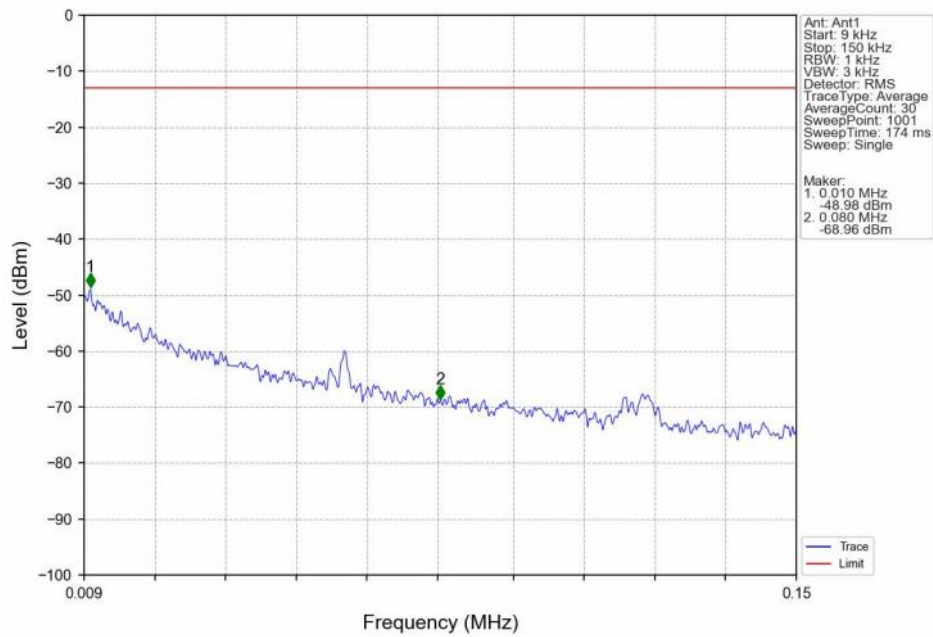
Band26b 3MHz QPSK MCH 836.5MHz RB 1 0 NTNV
