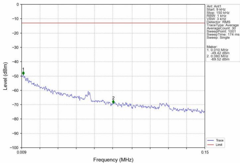
Band26b 1.4MHz 16QAM LCH 824.7MHz RB 1 0 NTNV
