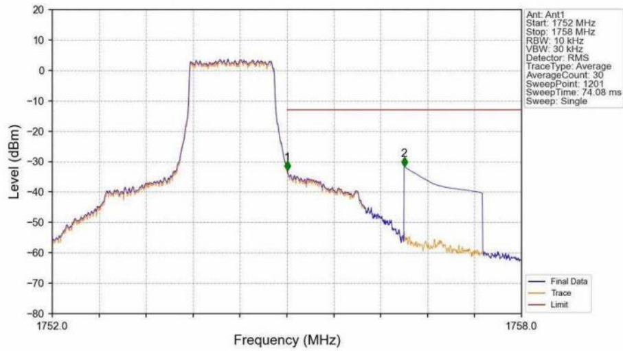
Band4 1.4MHz QPSK HCH 1754.3MHz RB 6 0 NTNV
