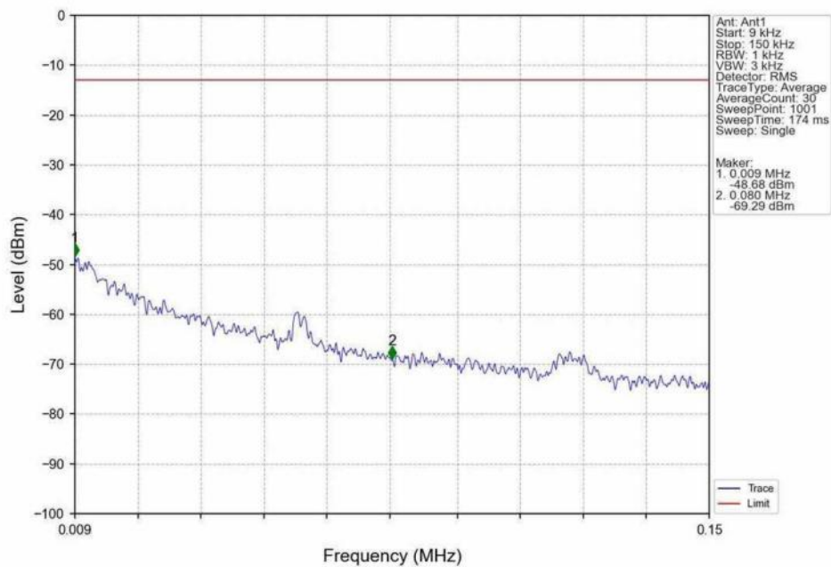
Band4 1.4MHz 16QAM HCH 1754.3MHz RB 1 0 NTN
