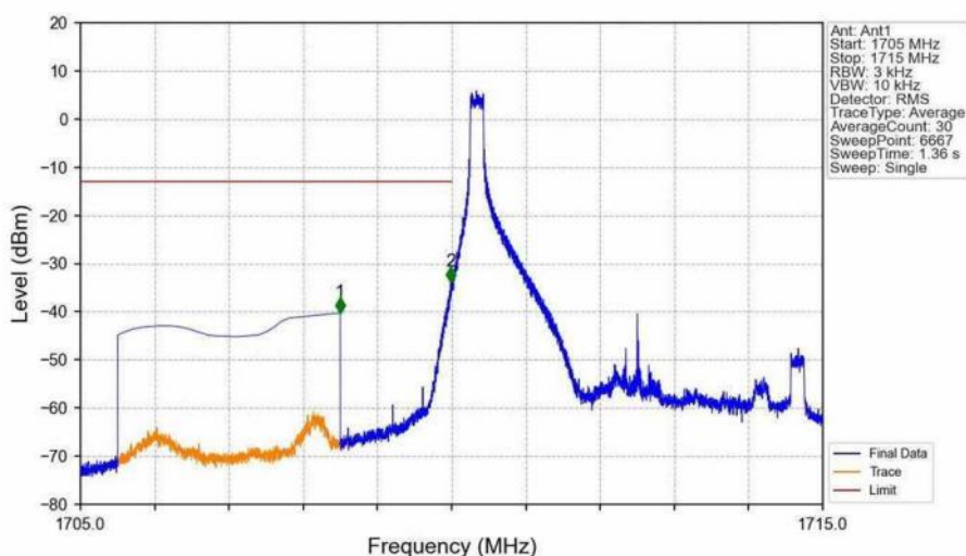
Band4_5MHz_16QAM_LCH_1712.5MHz_RB_1_0_NTNV
