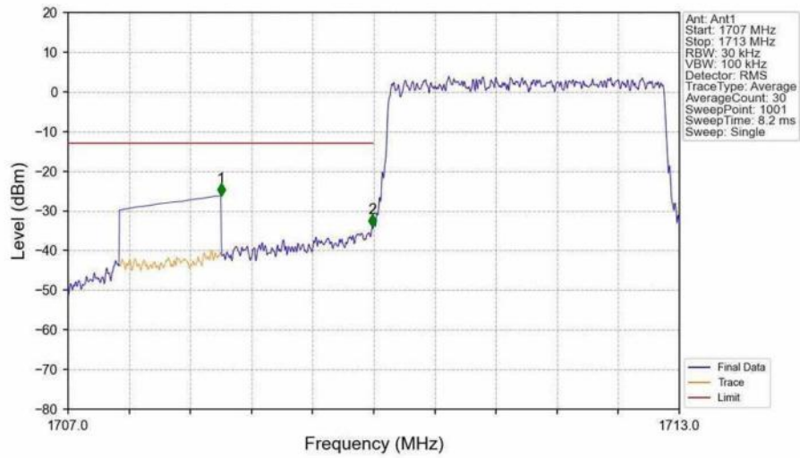
Band4 3MHz QPSK LCH 1711.5MHz RB 15 0 NTNV
