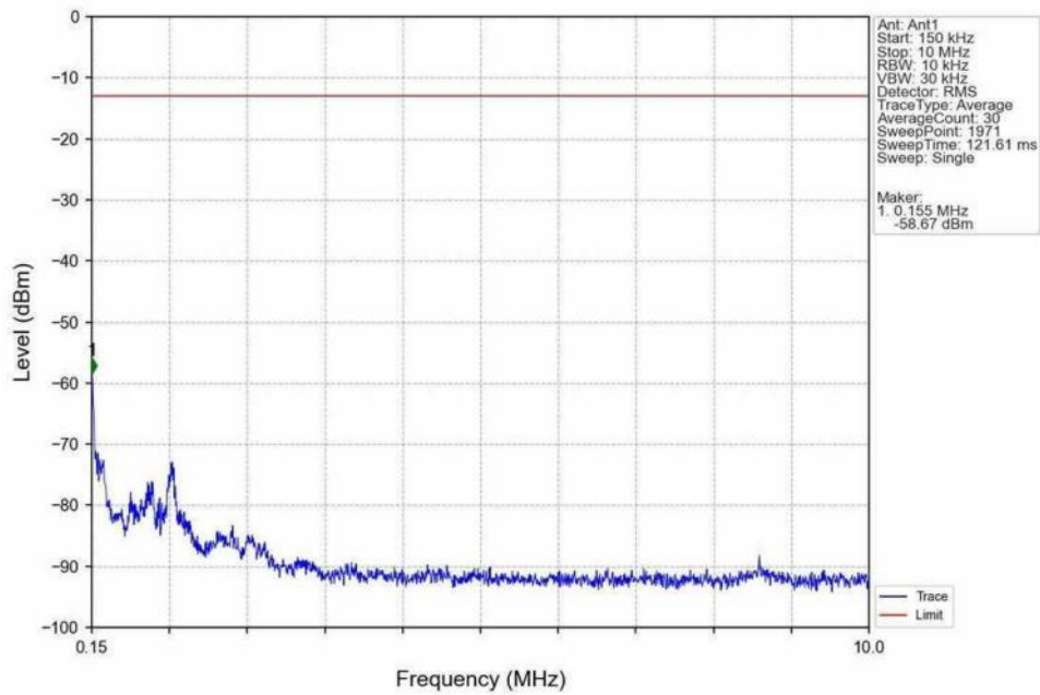
Band4_5MHz_QPSK_MCH_1732.5MHz_RB_1_0_NTNV
