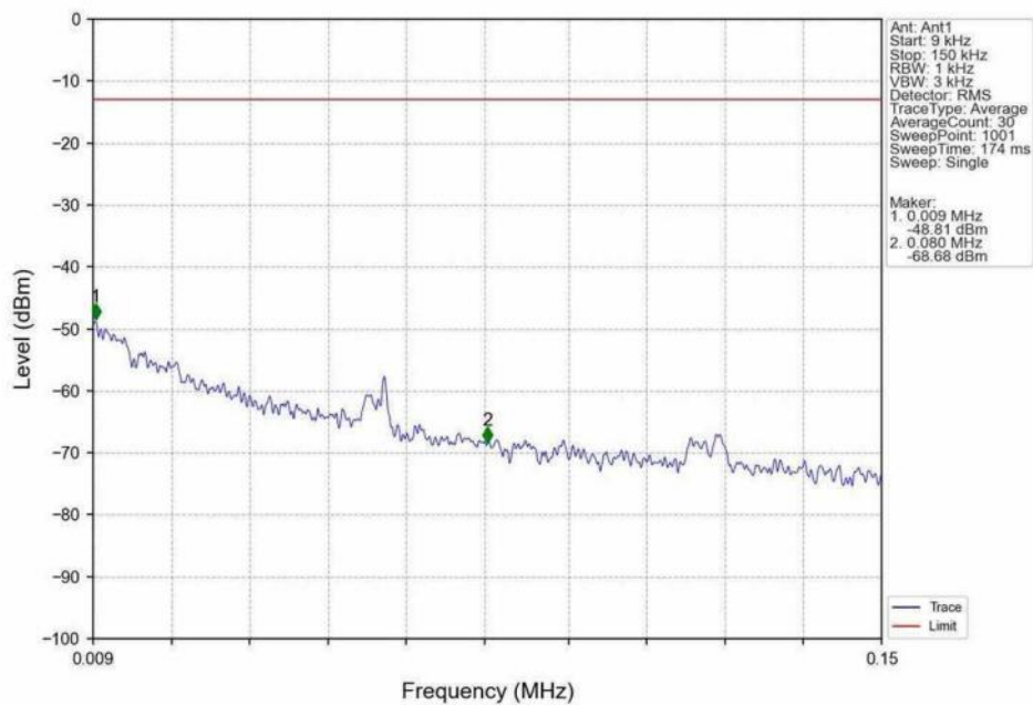
Band4 1.4MHz QPSK MCH 1732.5MHz RB 1 0 NTNV
