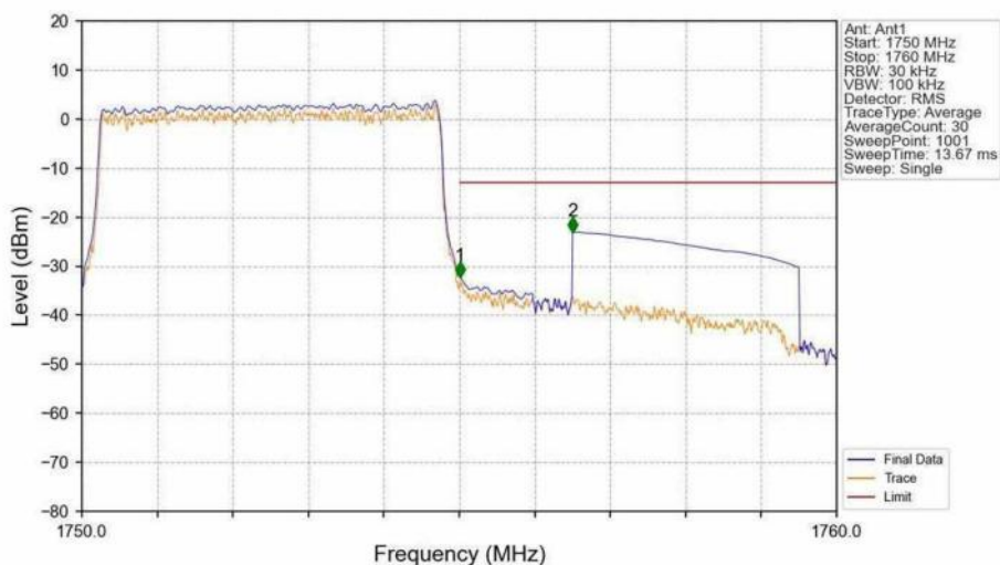
Band4_5MHz_QPSK_HCH_1752.5MHz_RB_25_0_NTNV
