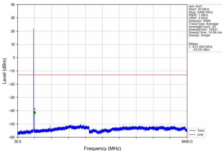
Band5_5MHz_QPSK_LCH_826.5MHz_RB_25_0_NTNV
