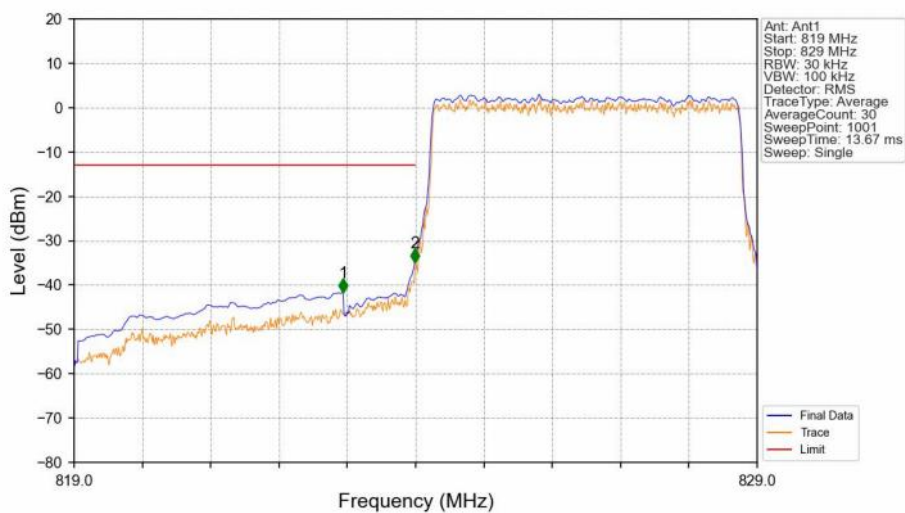
Band5_5MHz_QPSK_LCH_826.5MHz_RB_25_0_NTNV
