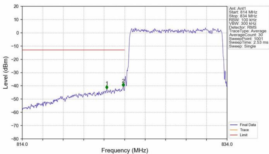
Band5_10MHz_16QAM_LCH_829MHz_RB_50_0_NTNV
