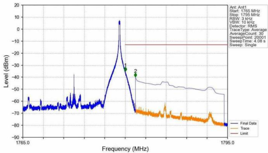
Band66_15MHz_QPSK_HCH_1772.5MHz_RB_1_74_NTNV
