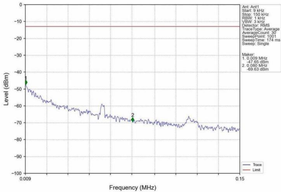
Band66_20MHz_16QAM_MCH_1745MHz_RB_1_0_NTNV
