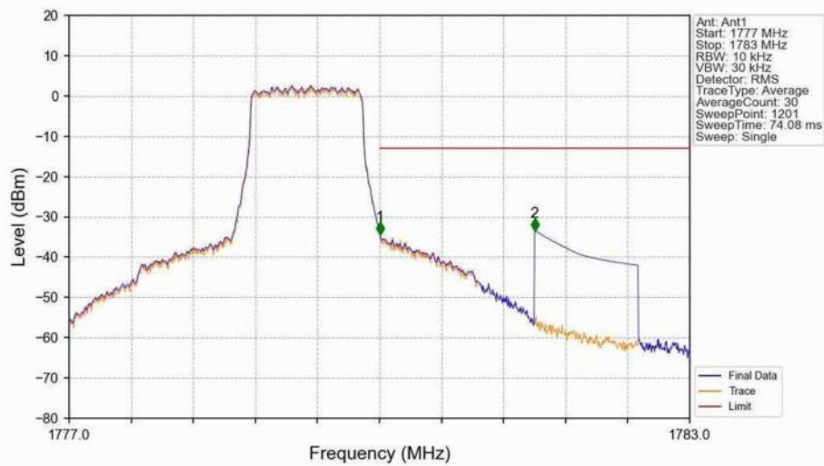
Band66 1.4MHz 16QAM HCH 1779.3MHz RB 6 0 NTN
