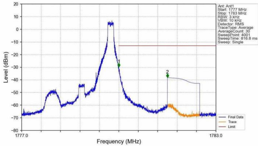
Band66 1.4MHz 16QAM HCH 1779.3MHz RB 1 5 NTN
