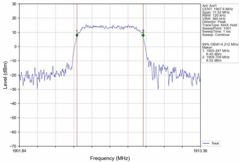
Band2 HSUPA HCH 1907.6MHz Subtest 1 NTV
