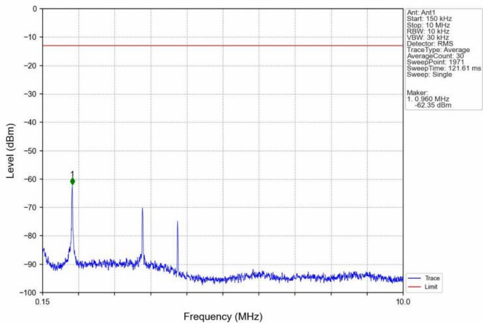
Band4 HSDPA_LCH 1712.4MHz Subtest 1_NTNV
