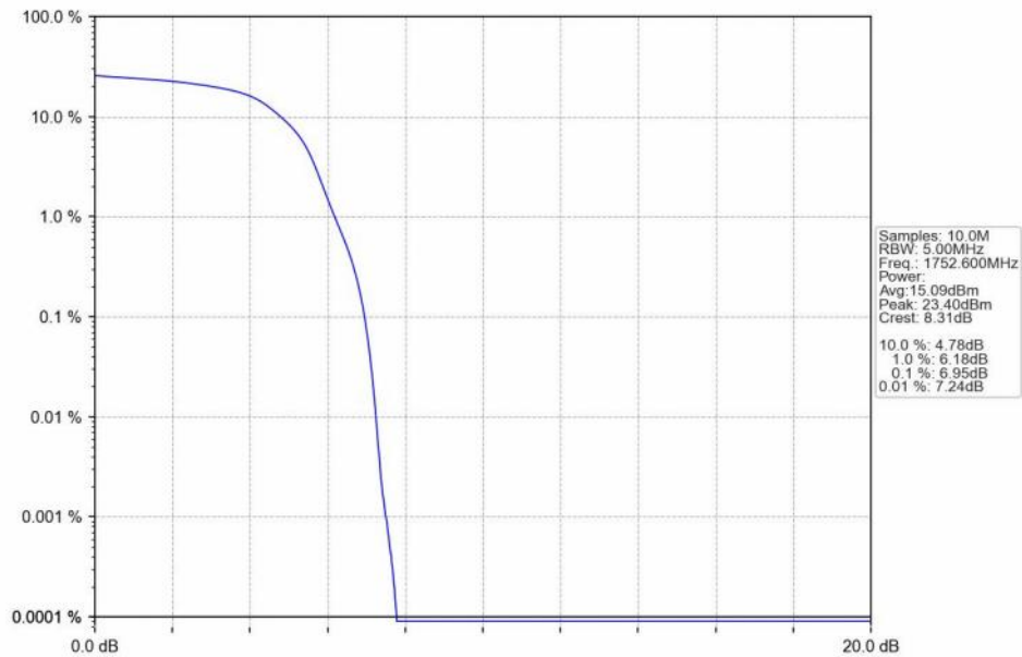
Band4 HSUPA HCH 1752.6MHz Subtest 1 NTV
