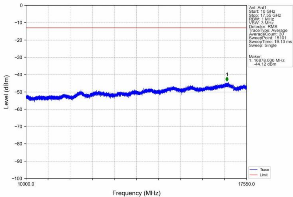
Band4 HSDPA MCH 1732.6MHz Subtest 1 NTV
