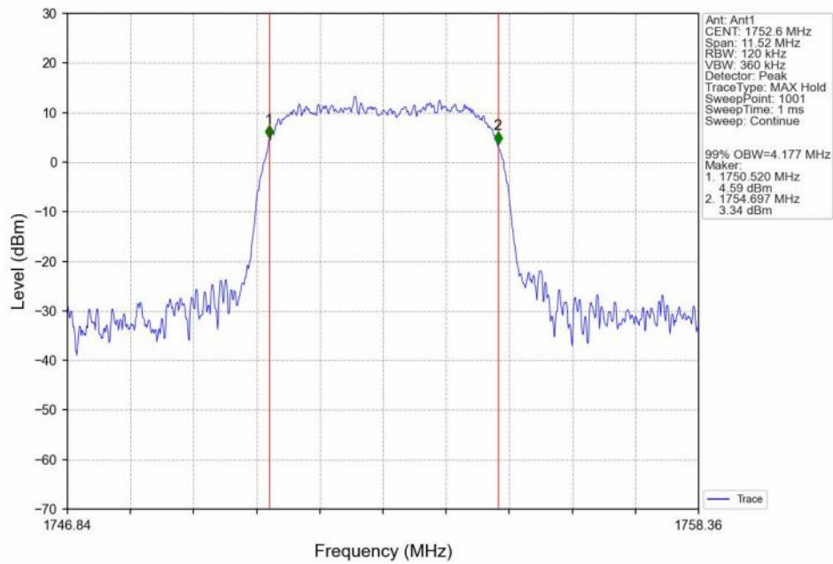
Band4 HSUPA HCH 1752.6MHz Subtest 1 NTN
