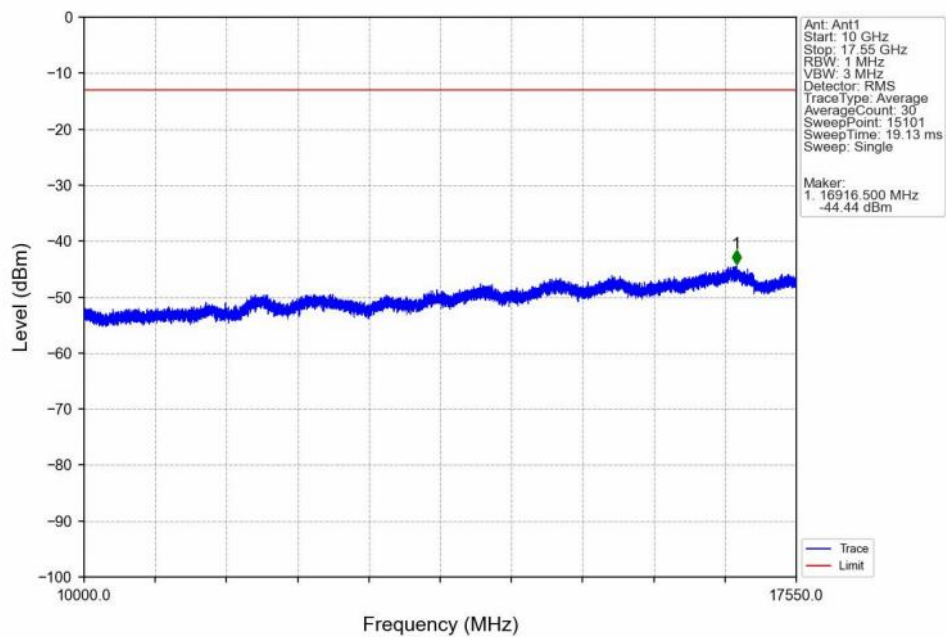
Band4_RMC_LCH_1712.4MHz_12.2kbps_RMC_NTNV
