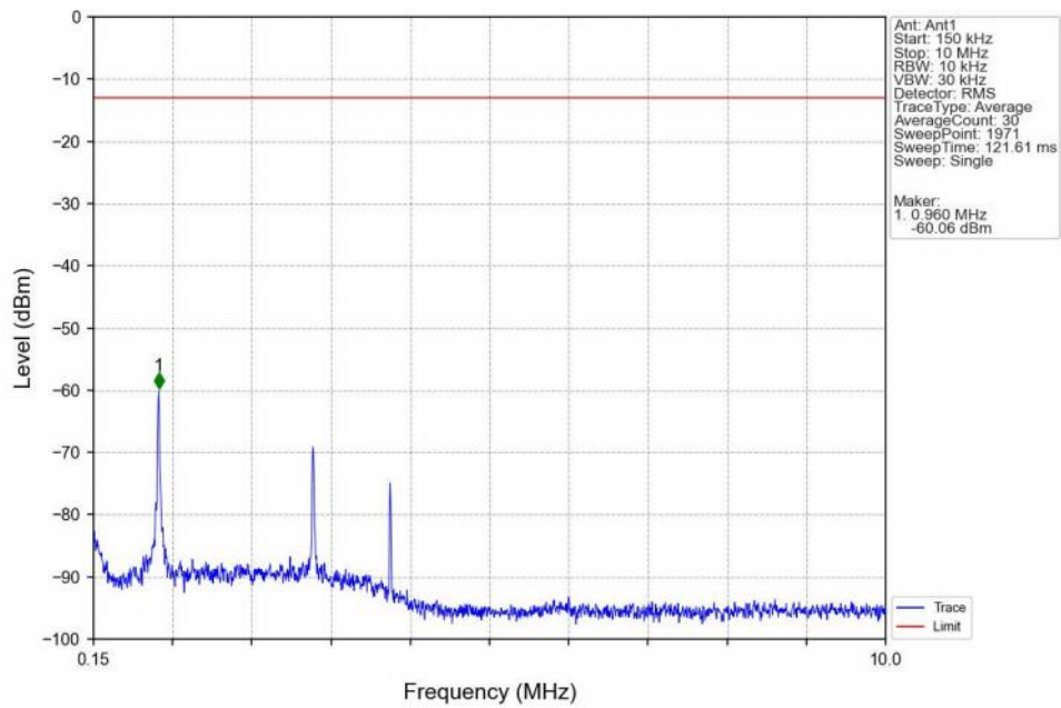
Band4 HSDPA MCH 1732.6MHz Subtest 1 NTN
