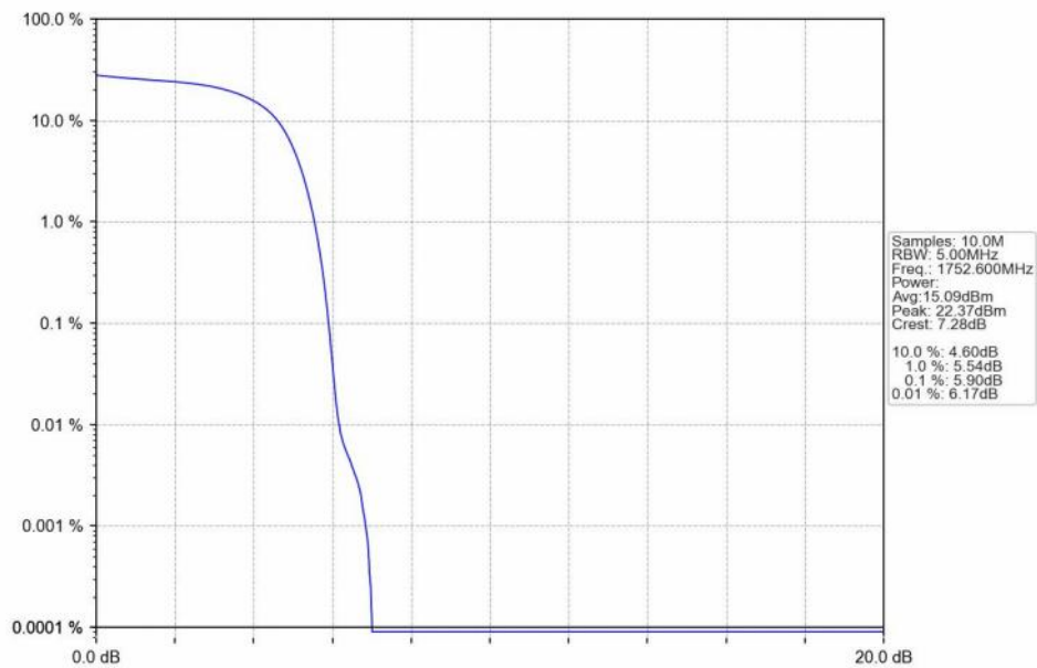
Band4 HSDPA HCH 1752.6MHz Subtest 1 NTN
