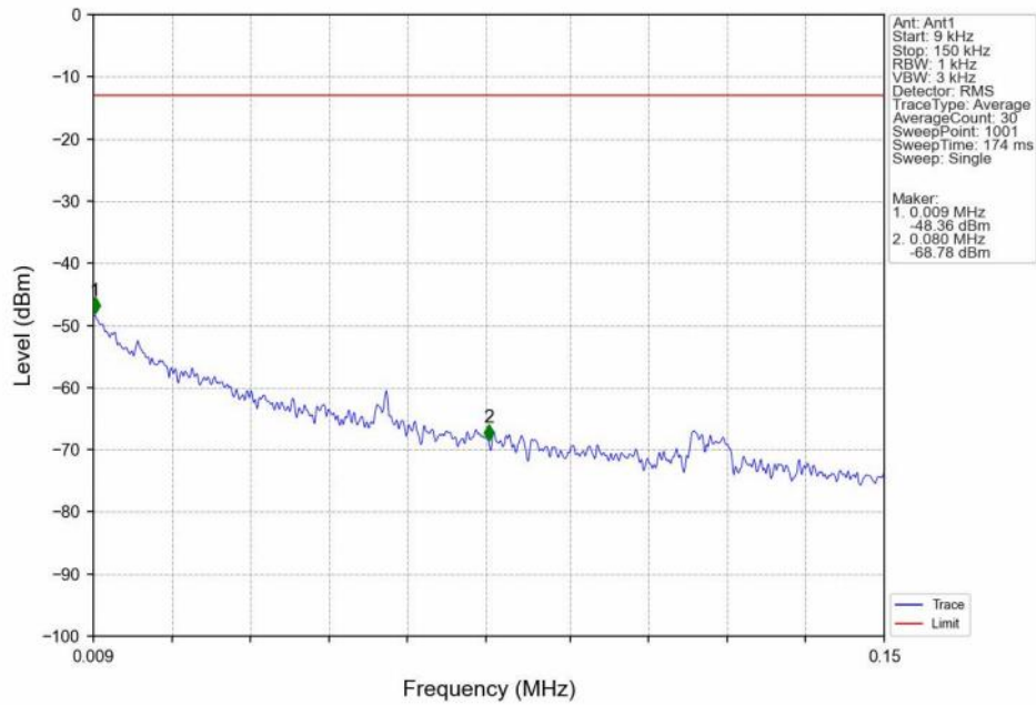
Band4 HSUPA MCH 1732.6MHz Subtest 1 NTN
