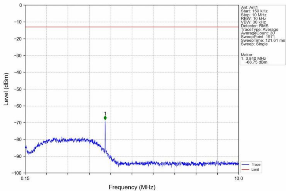
Band4_RMC_MCH_1732.6MHz_12.2kbps_RMC_NTNV
