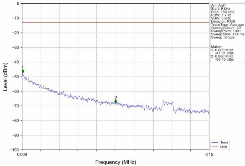
Band4 HSDPA_LCH 1712.4MHz Subtest 1_NTNV
