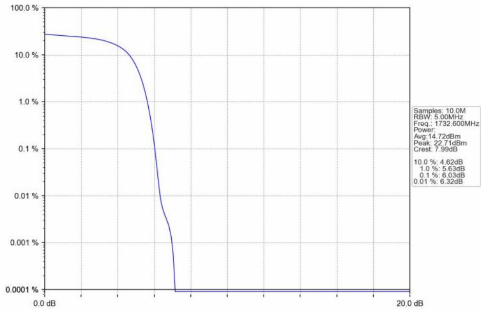
Band4 HSDPA MCH 1732.6MHz Subtest 1 NTN
