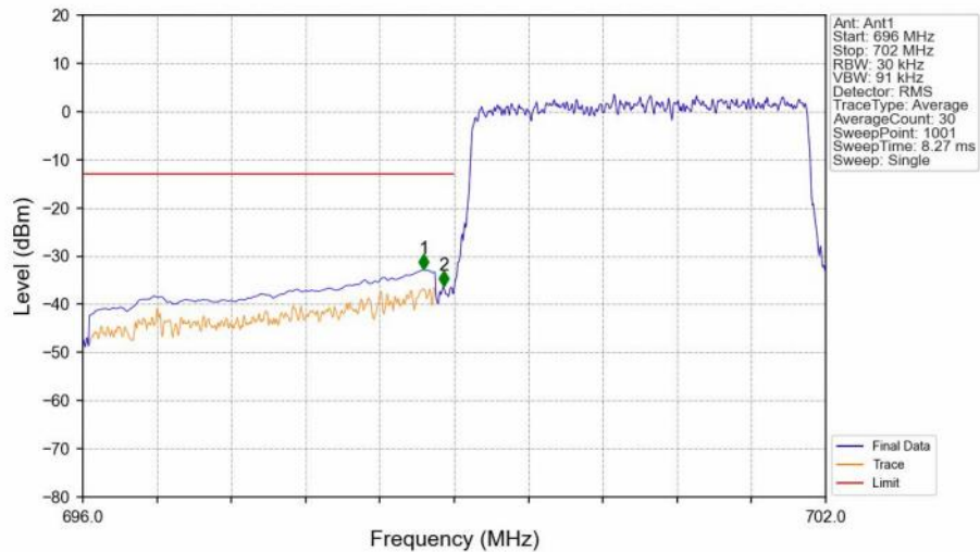
Band12_3MHz_QPSK_LCH_700.5MHz_RB_15_0_NTNV
