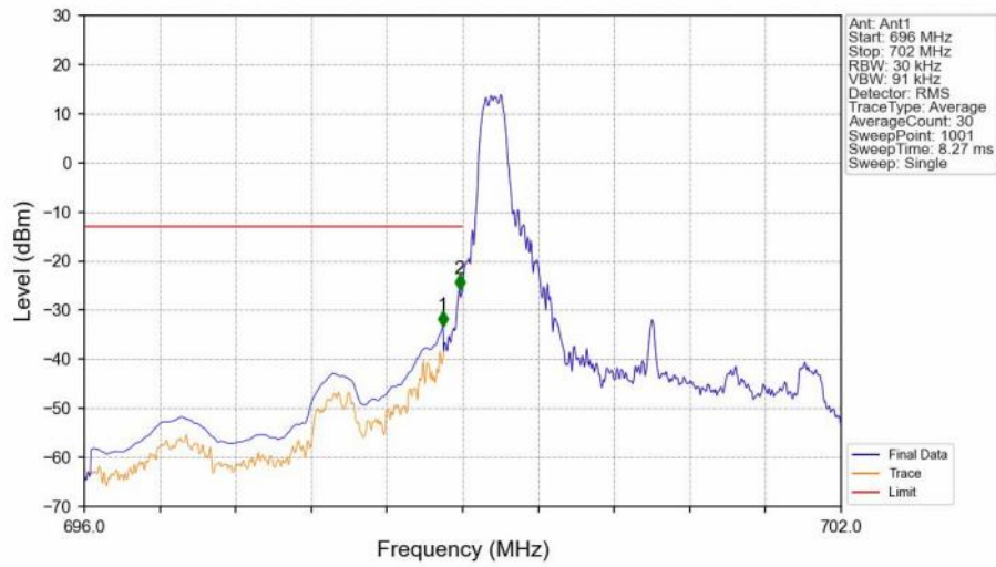
Band12_3MHz_16QAM_LCH_700.5MHz_RB_1_0_NTNV
