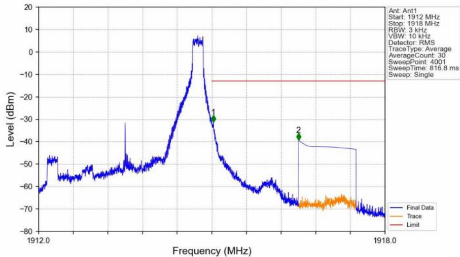
Band25_3MHz_QPSK_HCH_1913.5MHz_RB_1_14_NTNV
