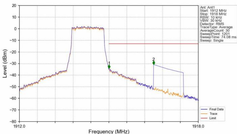
Band25_1.4MHz_16QAM_HCH_1914.3MHz_RB_6_0_NTNV
