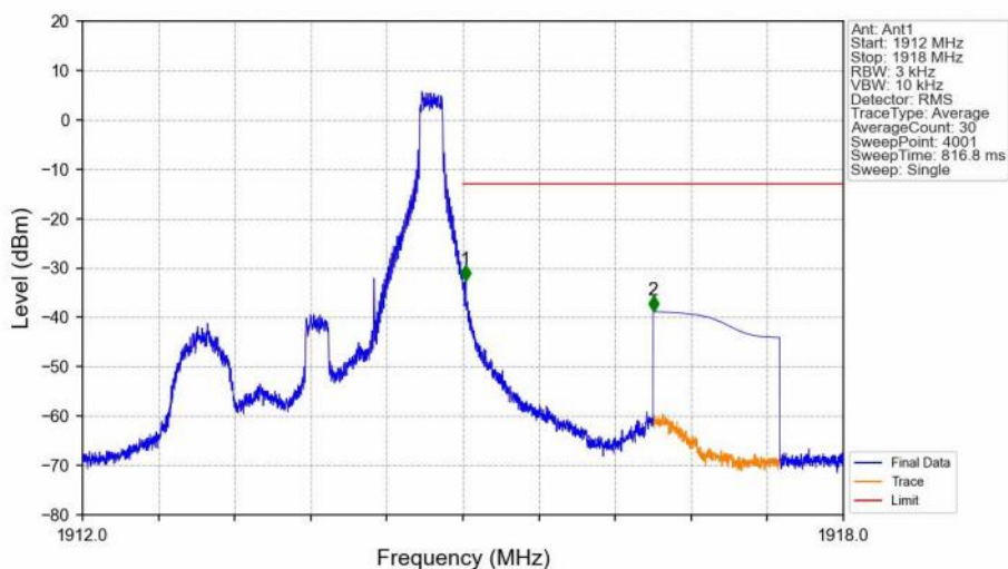
Band25_1.4MHz_16QAM_HCH_1914.3MHz_RB_1_5_NTNV
