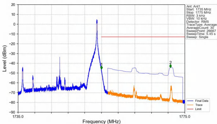
Band4_20MHz_16QAM_HCH_1745MHz_RB_1_99_NTNV
