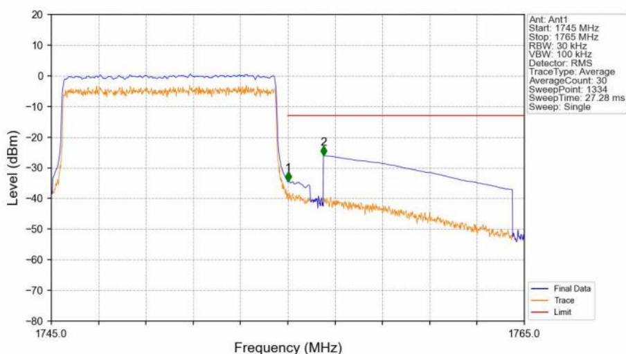
Band4_10MHz_16QAM_HCH_1750MHz_RB_50_0_NTNV
