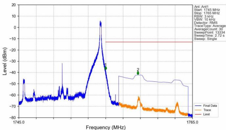
Band4_10MHz_16QAM_HCH_1750MHz_RB_1_49_NTNV
