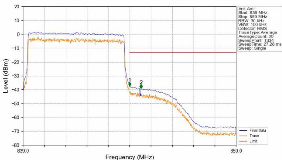
Band5_10MHz_16QAM_HCH_844MHz_RB_50_0_NTNV
