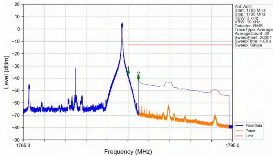
Band66_15MHz_16QAM_HCH_1772.5MHz_RB_1_74_NTNV
