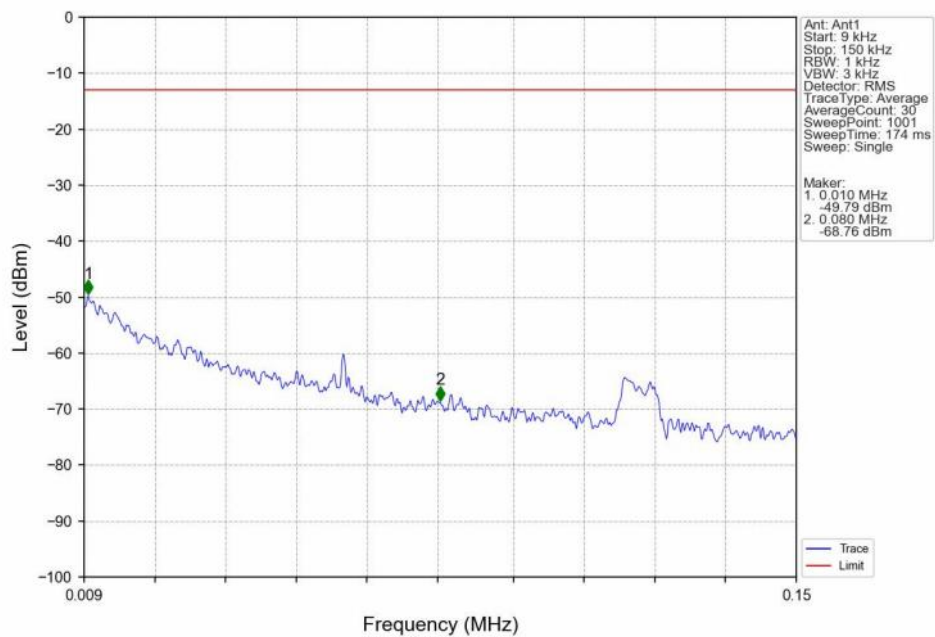
Band66_20MHz_16QAM_HCH_1770MHz_RB_1_0 NTN
