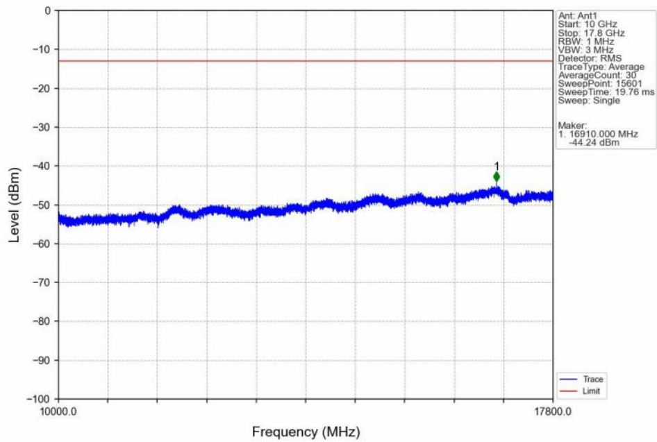
Band66_20MHz_16QAM_HCH_1770MHz_RB_1_0 NTN
