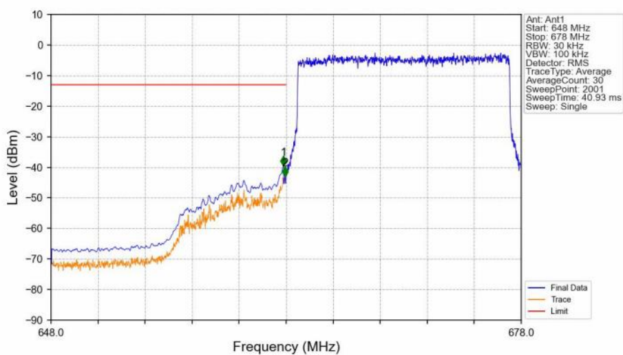
Band71_15MHz_QPSK_LCH_670.5MHz_RB_75_0_NTNV
