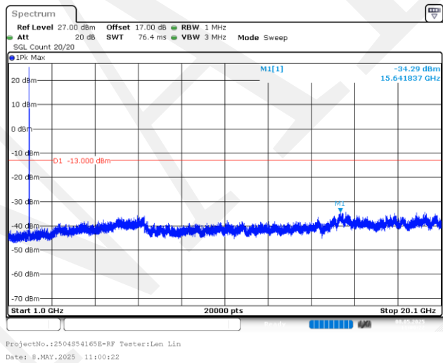
5MHz_High_QPSK_25@0(1GHz~20.1GHz)
