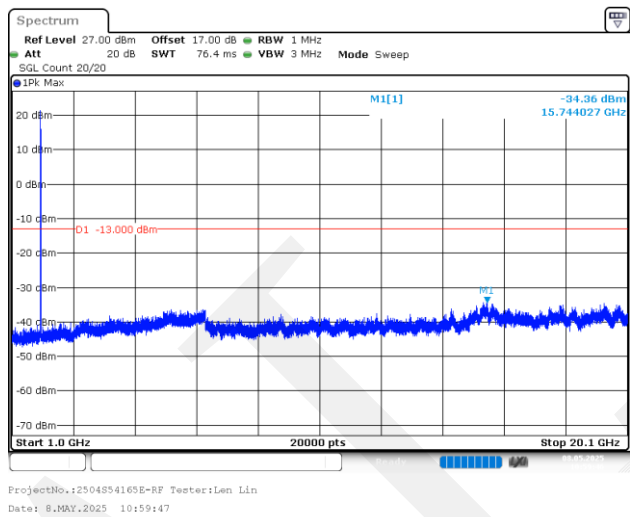
5MHz_High_QPSK_1@0(1GHz~20.1GHz)
