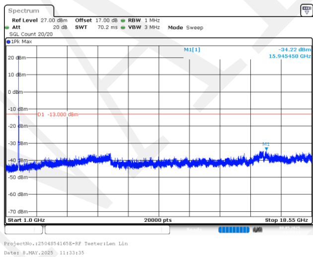
10MHz_Middle_QPSK_1@0(1GHz~18.55GHz)
