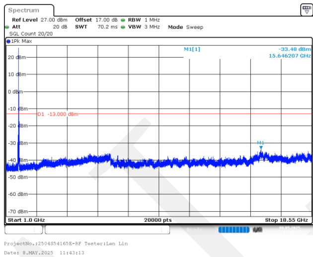
20MHz_Low_QPSK_100@0(1GHz~18.55GHz)
