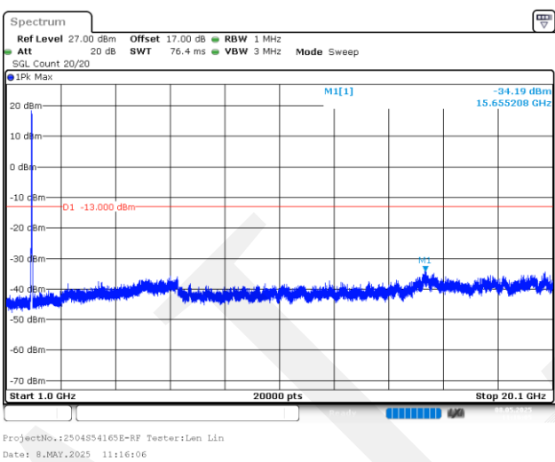
20MHz_High_QPSK_1@0(1GHz~20.1GHz)
