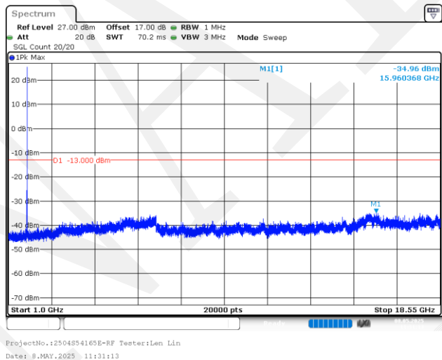
5MHz_High_QPSK_25@0(1GHz~18.55GHz)
