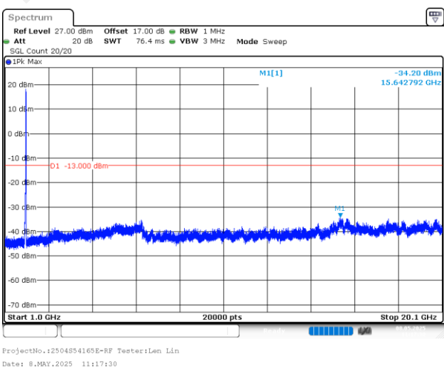
20MHz_High_QPSK_100@0(1GHz~20.1GHz)
