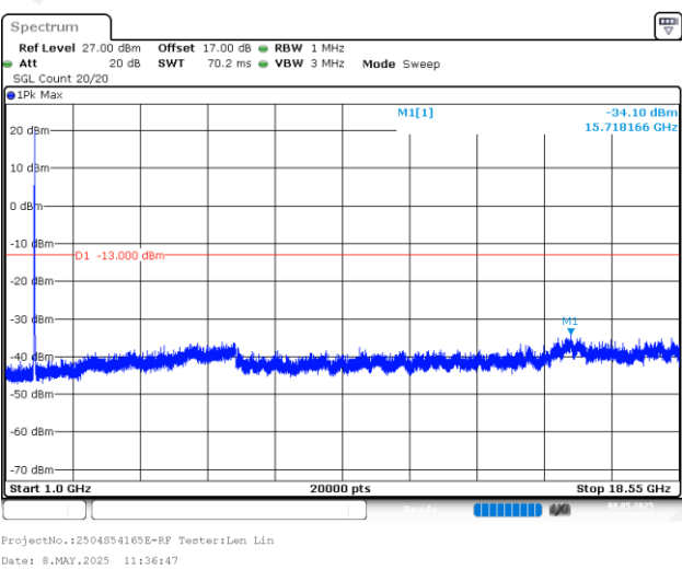
10MHz_High_QPSK_50@0(1GHz~18.55GHz)
