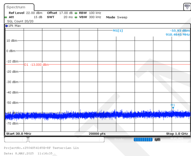
20MHz_High_QPSK_100@0(30MHz~1GHz)
