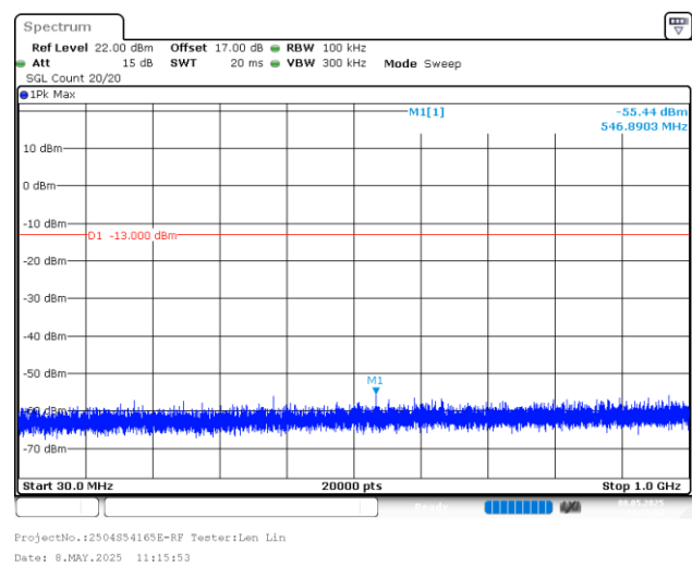
20MHz_High_QPSK_1@0(30MHz~1GHz)
