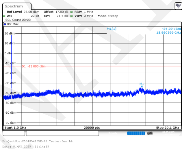
20MHz_Middle_QPSK_1@0(1GHz~20.1GHz)
