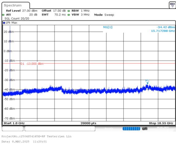
1.4MHz_Middle_QPSK_1@0(1GHz~18.55GHz)
