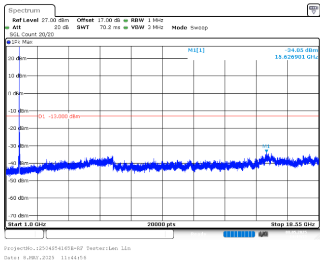
20MHz_Middle_QPSK_1@0(1GHz~18.55GHz)
