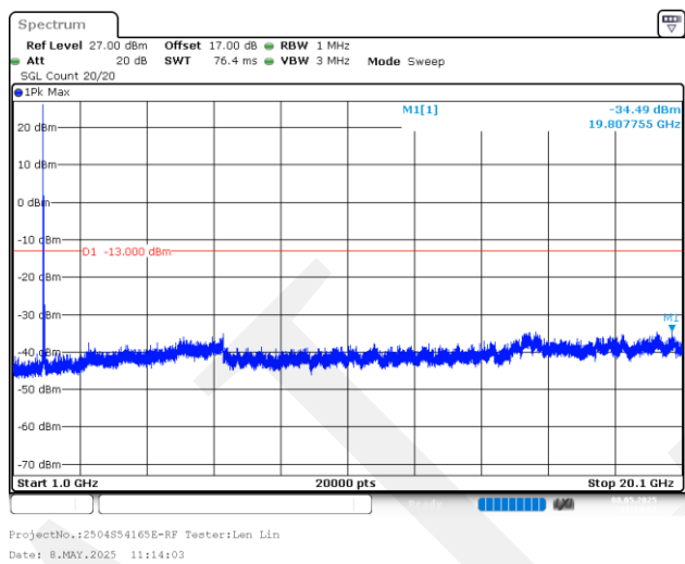
20MHz_Low_QPSK_100@0(1GHz~20.1GHz)
