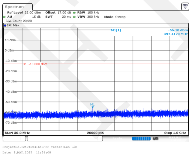
10MHz_Middle_QPSK_1@0(30MHz~1GHz)
