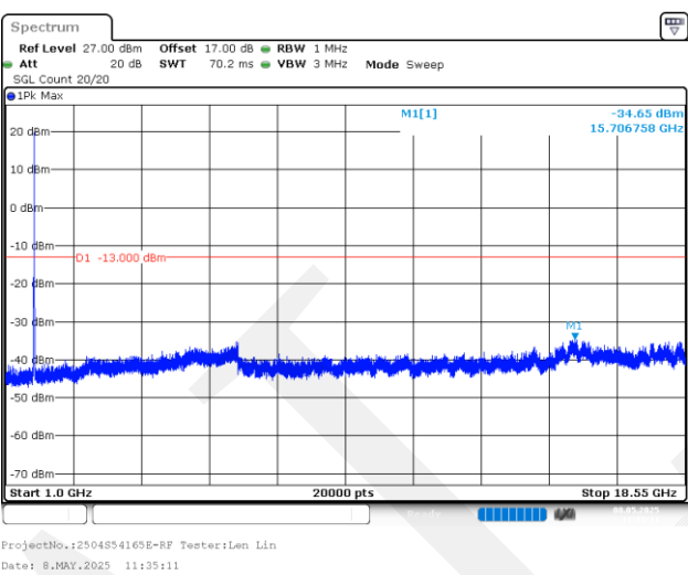
10MHz_High_QPSK_1@0(1GHz~18.55GHz)
