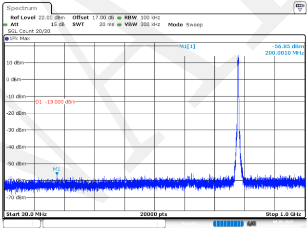
5MHz_High_QPSK_25@0(30MHz~1GHz)
