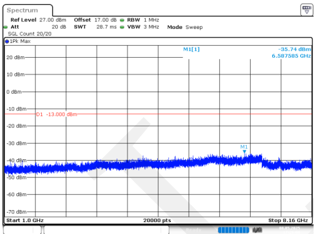
5MHz_Middle_QPSK_25@0(1GHz~8.16GHz)
