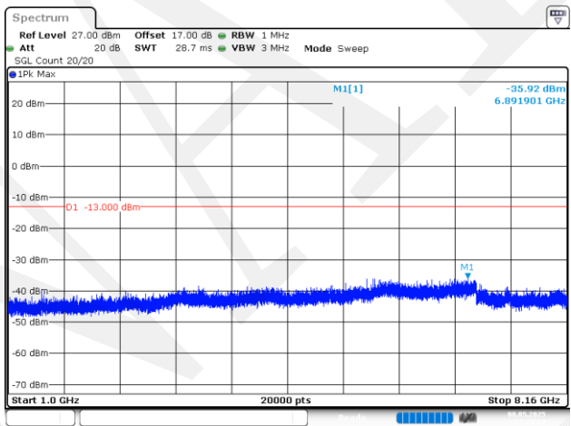
5MHz_High_QPSK_1@0(1GHz~8.16GHz)
