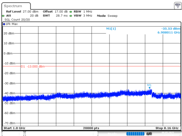
5MHz_High_QPSK_25@0(1GHz~8.16GHz)
