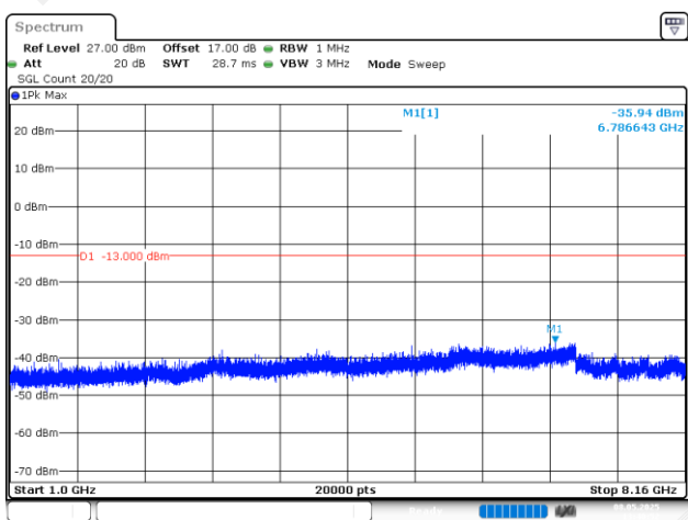
10MHz_High_QPSK_50@0(1GHz~8.16GHz)
