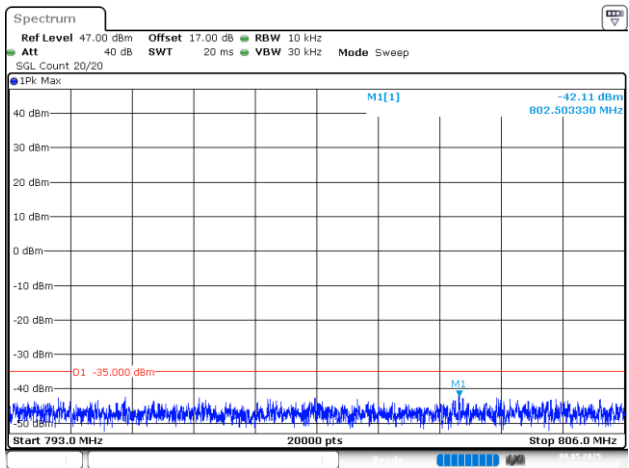
5MHz_High_QPSK_25@0(793MHz~806MHz)
