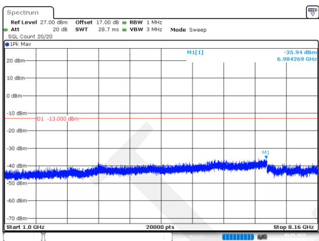
10MHz_Middle_QPSK_50@0(1GHz~8.16GHz)
