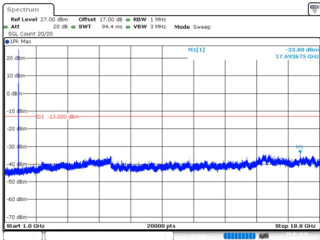
1.4MHz_High_QPSK_6@0(1GHz~18.8GHz)
