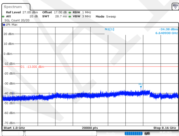
10MHz_High_QPSK_1@0(1GHz~8.16GHz)
