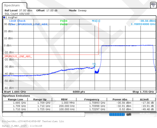
15MHz_Low_16QAM_75@0
