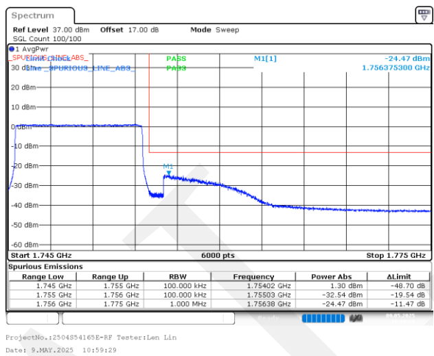
15MHz_Low_QPSK_75@0
