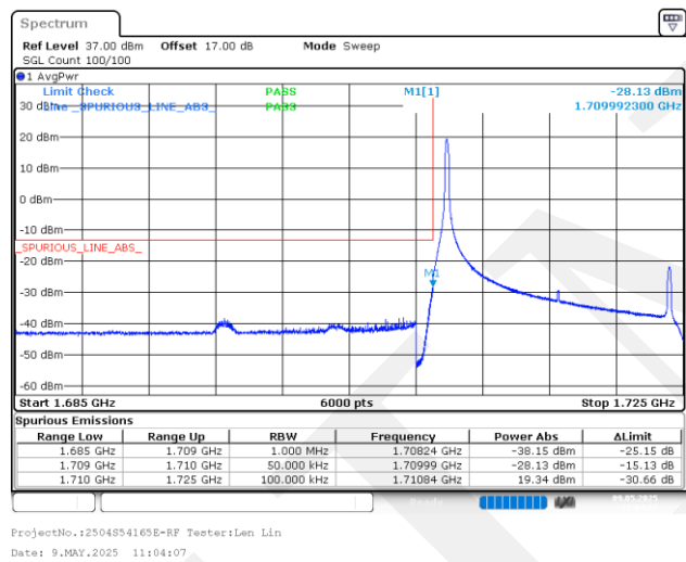
15MHz_Low_16QAM_1@0
