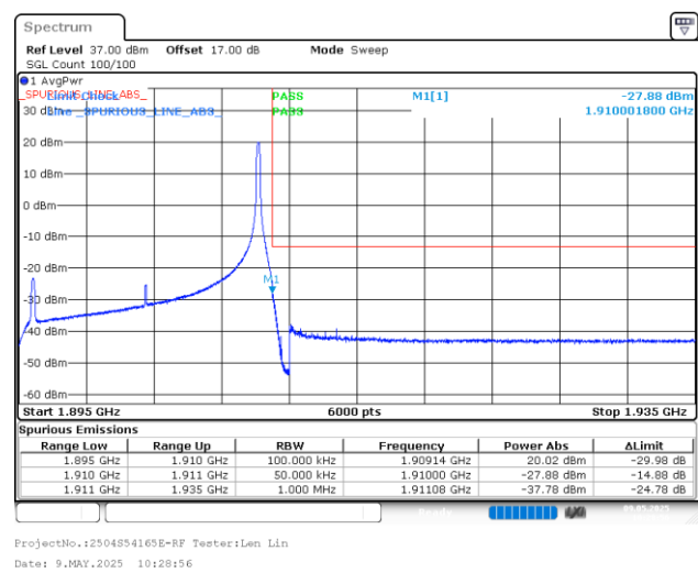
15MHz_High_16QAM_1@74
