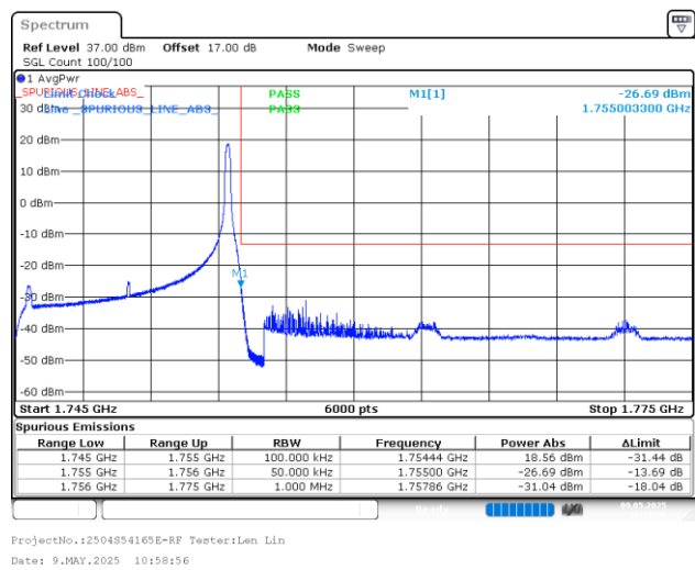
15MHz_Low_QPSK_1@0
