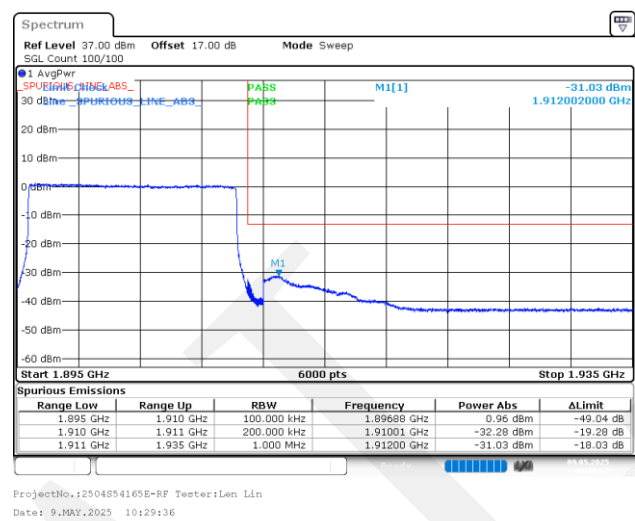
15MHz_High_16QAM_75@0
