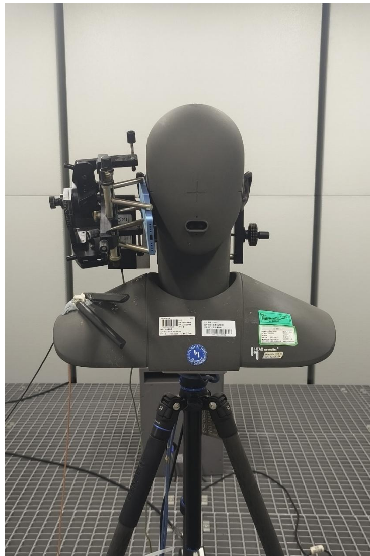
Picture 3: Volume Control Test Setup
