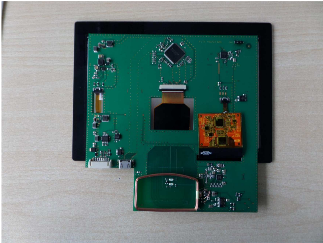
PCB mounted on Touchscreen
