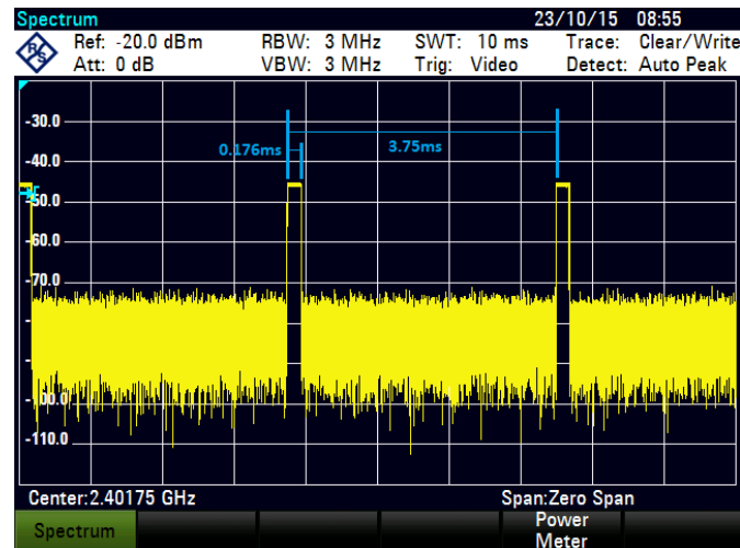
Figure 8.4-1: Duty Cycle correction pulse
