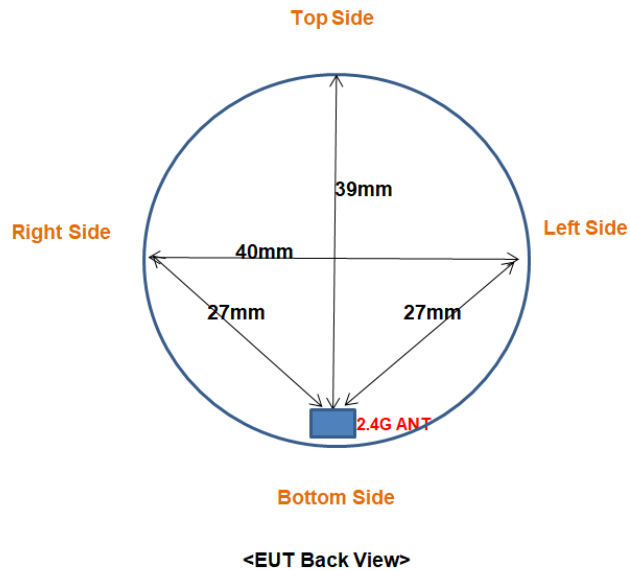
Fig 7.1 Block Diagram for EUT Antenna Position
