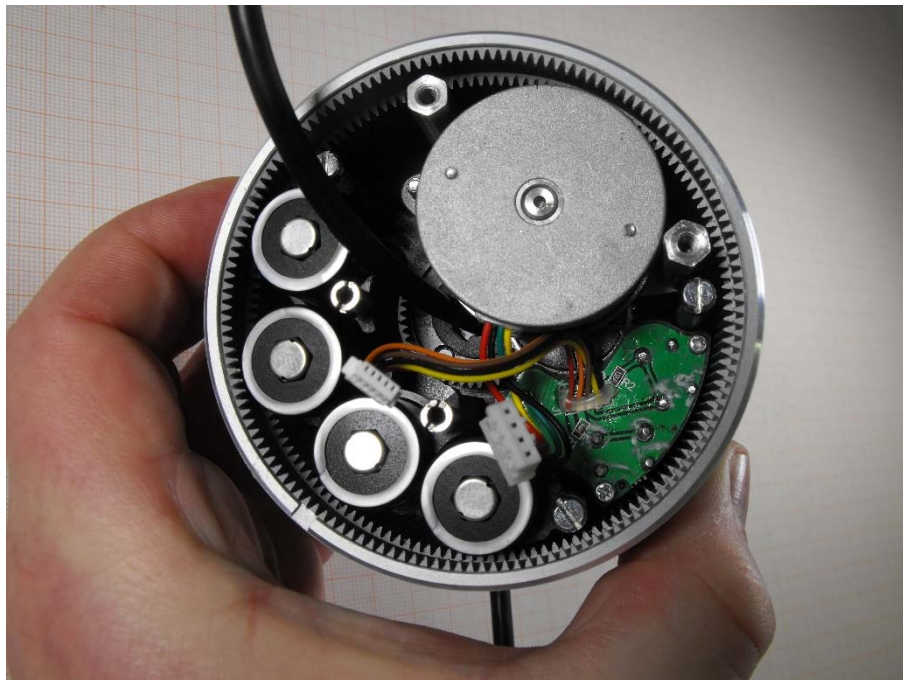
Photo 1: Gear unit
