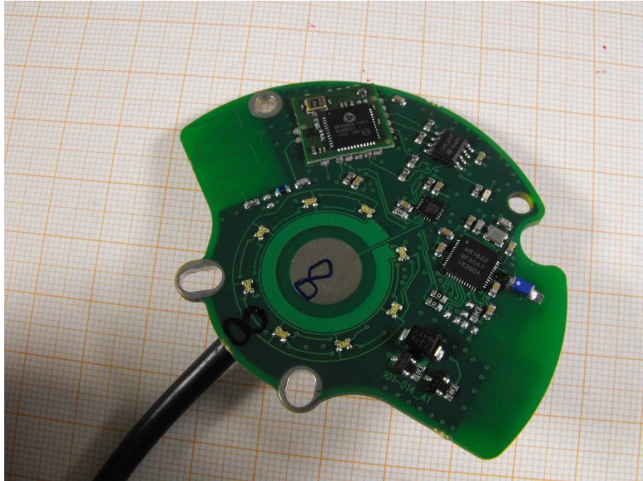
Photo 3: Main board front side
