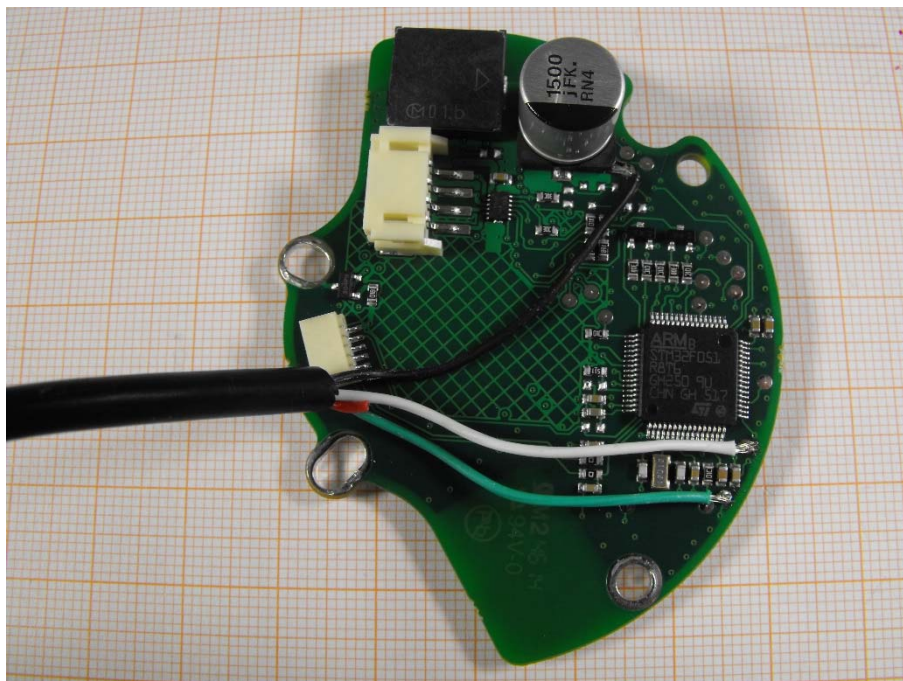
Photo 2: Main board rear side (the wires are only necessary to set the test mode)
