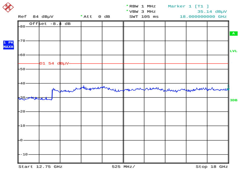
Plot 8: 12.75 GHz to 18 GHz, TX mode, channel 39, vertical & horizontal polarization
