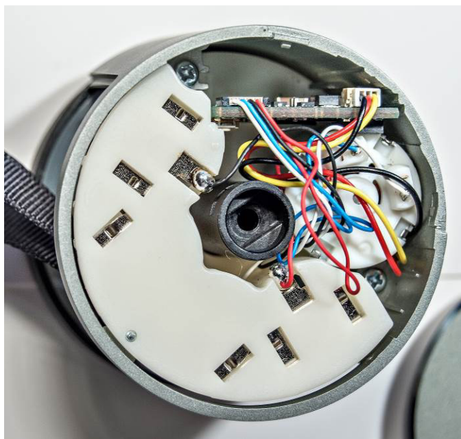
Lock with top dismantled
