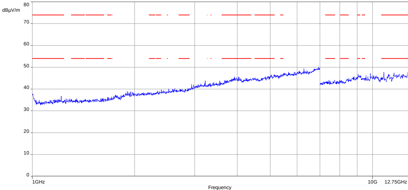
Plot 3: 1 GHz to 12.75 GHz, RX mode, vertical & horizontal polarization
