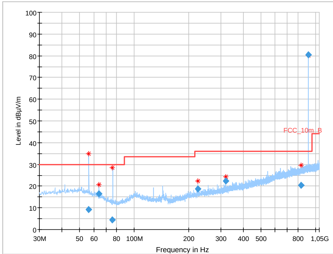
Plot 2: 30 MHz to 1 GHz, TX mode, 916.0 MHz, vertical & horizontal polarization
