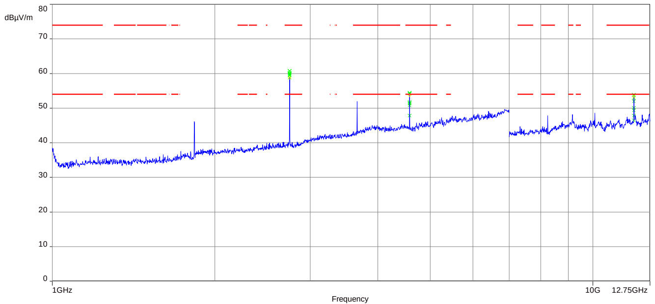
Plot 2: 1 GHz to 12.75 GHz, TX mode, 916.0 MHz, vertical & horizontal polarization
