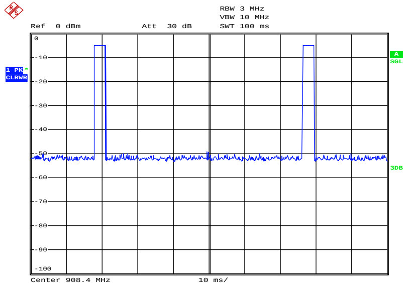
Plot 2: Number of bursts in 100ms = 2
