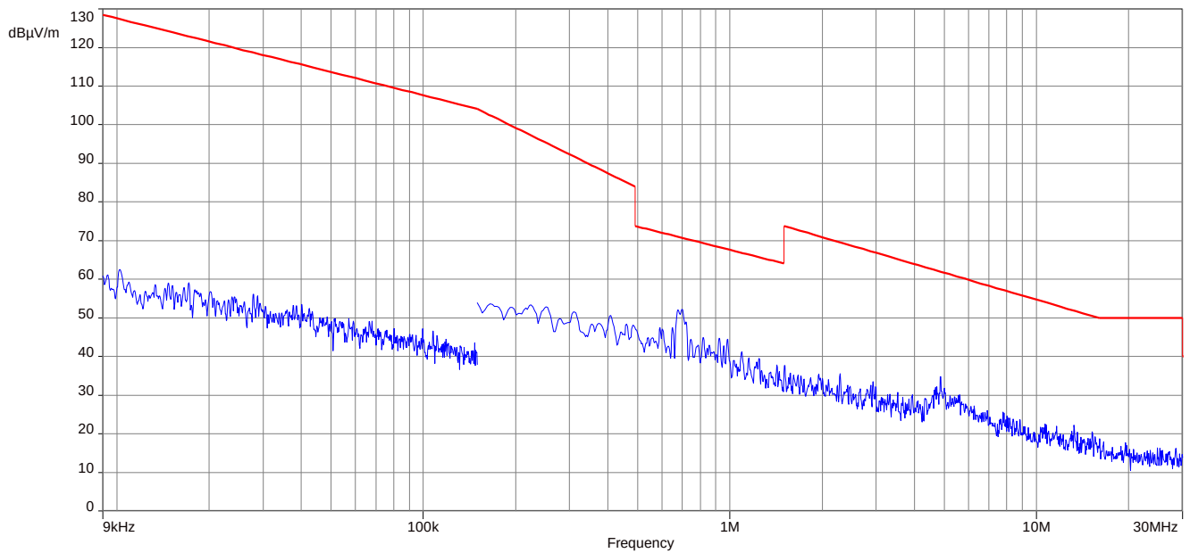
Plot 2: 9 kHz to 30 MHz, 916.0 MHz
