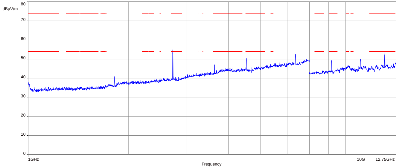
Plot 1: 1 GHz to 12.75 GHz, TX mode, 908.4 MHz, vertical & horizontal polarization
