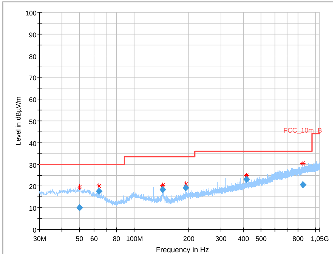
Plot 3: 30 MHz to 1 GHz, RX mode, vertical & horizontal polarization
