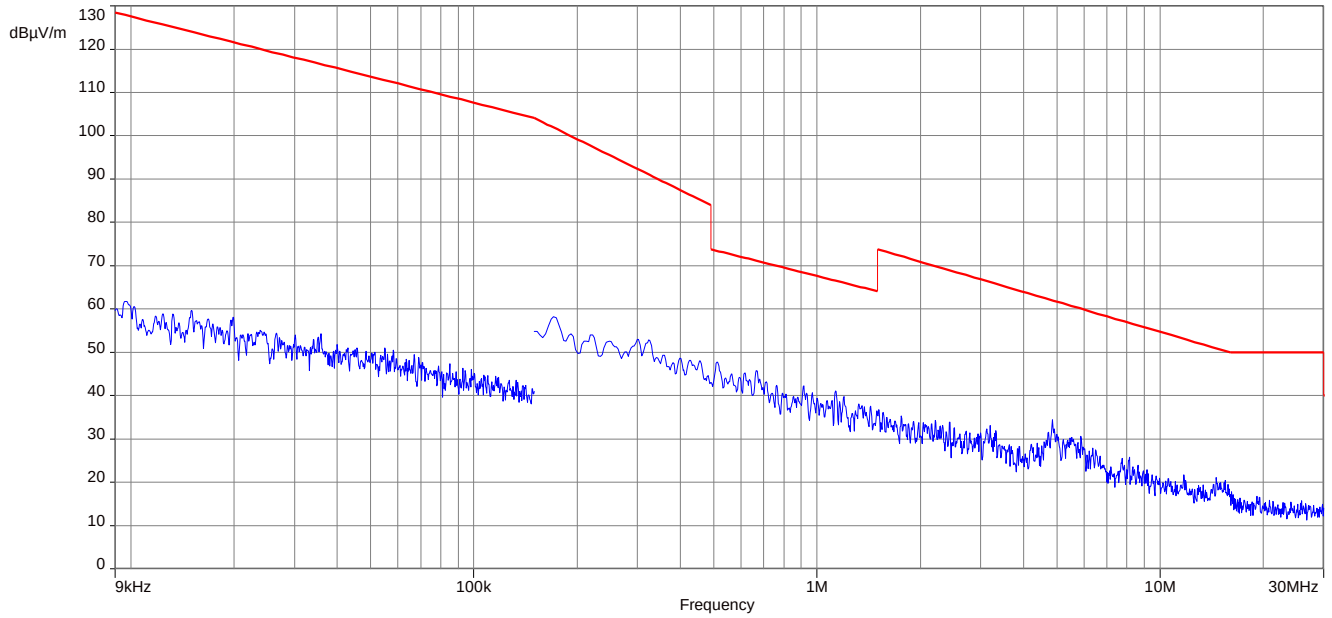
Plot 1: 9 kHz to 30 MHz, 908.4 MHz
